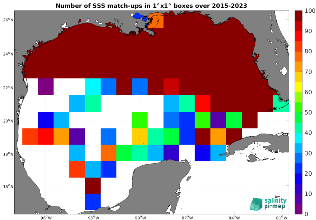
Figure 4: Number of SSS match-ups between TSG (SAMOS) SSS and the SMAP SSS L3 v5.0 - Monthly (JPL) SSS product for the Gulf of Mexico Pi-MEP region over 1^\circ \times 1^\circ boxes and for the full satellite product period.
