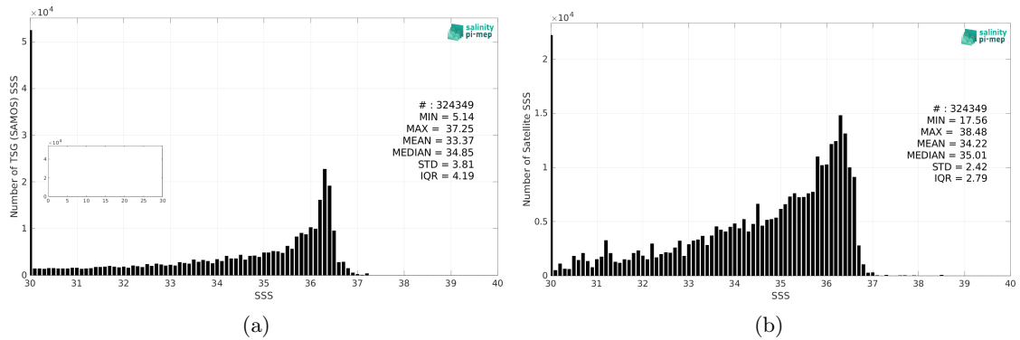
Figure 2: Histograms of SSS from TSG (SAMOS) (a) and SMAP SSS L3 v5.0 - Monthly (JPL) (b) considering all match-up pairs per bins of 0.1 over the Gulf of Mexico Pi-MEP region and for the full satellite product period.
