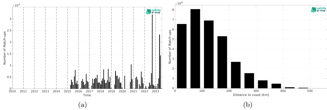
Figure 1: Number of match-ups between TSG (SAMOS) and SMAP SSS L3 v5.0 - Monthly (JPL) SSS as a function of time (a) and as function of the distance to coast (b) over the Gulf of Mexico Pi-MEP region and for the full satellite product period.
