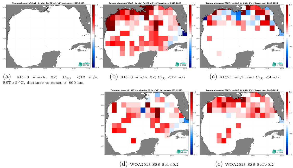
Figure 12: Temporal mean gridded over spatial boxes of size 1^\circ \times 1^\circ of \Delta\text{SSS} (SMAP SSS L3 v5.0 - Monthly (JPL) - TSG (SAMOS)) for 5 different subdatasets corresponding to:RR=0 mm/h, 3 < U_{10} < 12 m/s, SST >5^\circ\text{C} , distance to coast > 800 km (a), RR=0 mm/h, 3 < U_{10} < 12 m/s (b), RR >1 mm/h and U_{10} < 4 m/s (c), WOA2013 SSS Std <0.2 (d), WOA2013 SSS Std >0.2 (e).
