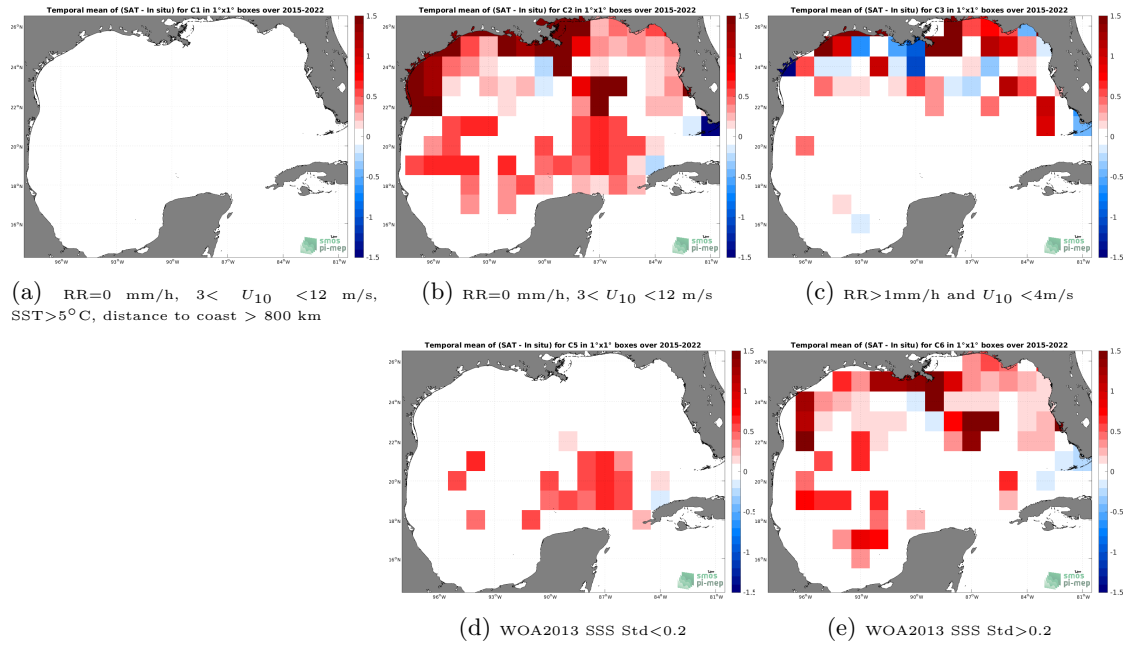
Figure 12: Temporal mean gridded over spatial boxes of size 1^\circ \times 1^\circ of \Delta SSS (SMAP SSS L3 v5.0 - Monthly (JPL) - TSG (SAMOS)) for 5 different subdatasets corresponding to:RR=0 mm/h, 3 < U_{10} < 12 m/s, SST >5^\circ C, distance to coast > 800 km (a), RR=0 mm/h, 3 < U_{10} < 12 m/s (b), RR >1 mm/h and U_{10} < 4 m/s (c), WOA2013 SSS Std <0.2 (d), WOA2013 SSS Std >0.2 (e).
