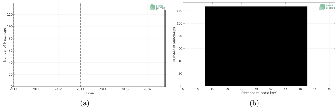
Figure 1: Number of match-ups between TSG (LEGOS-DM) and SMAP SSS L3 v5.0 - Monthly (JPL) SSS as a function of time (a) and as function of the distance to coast (b) over the Gulf of Mexico Pi-MEP region and for the full satellite product period.
