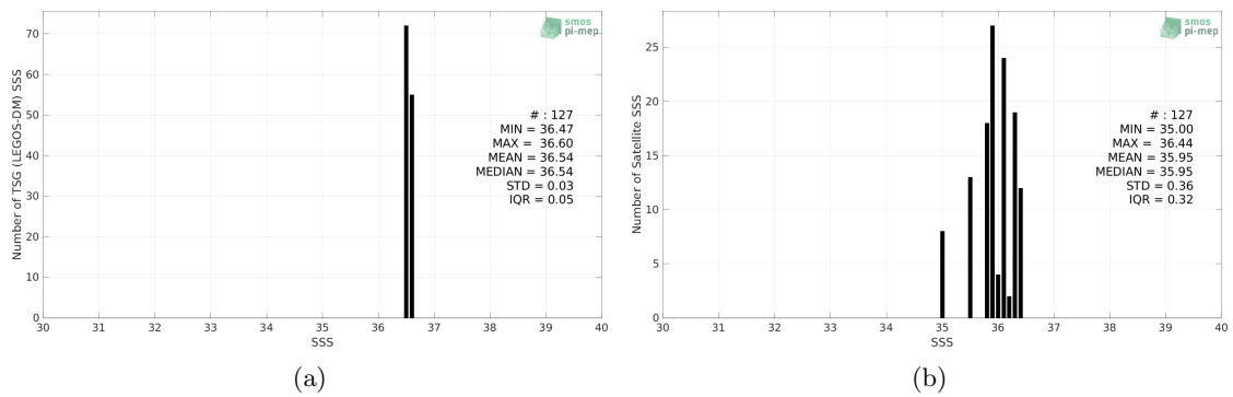
Figure 2: Histograms of SSS from TSG (LEGOS-DM) (a) and SMAP SSS L3 v5.0 - Monthly (JPL) (b) considering all match-up pairs per bins of 0.1 over the Gulf of Mexico Pi-MEP region and for the full satellite product period.
