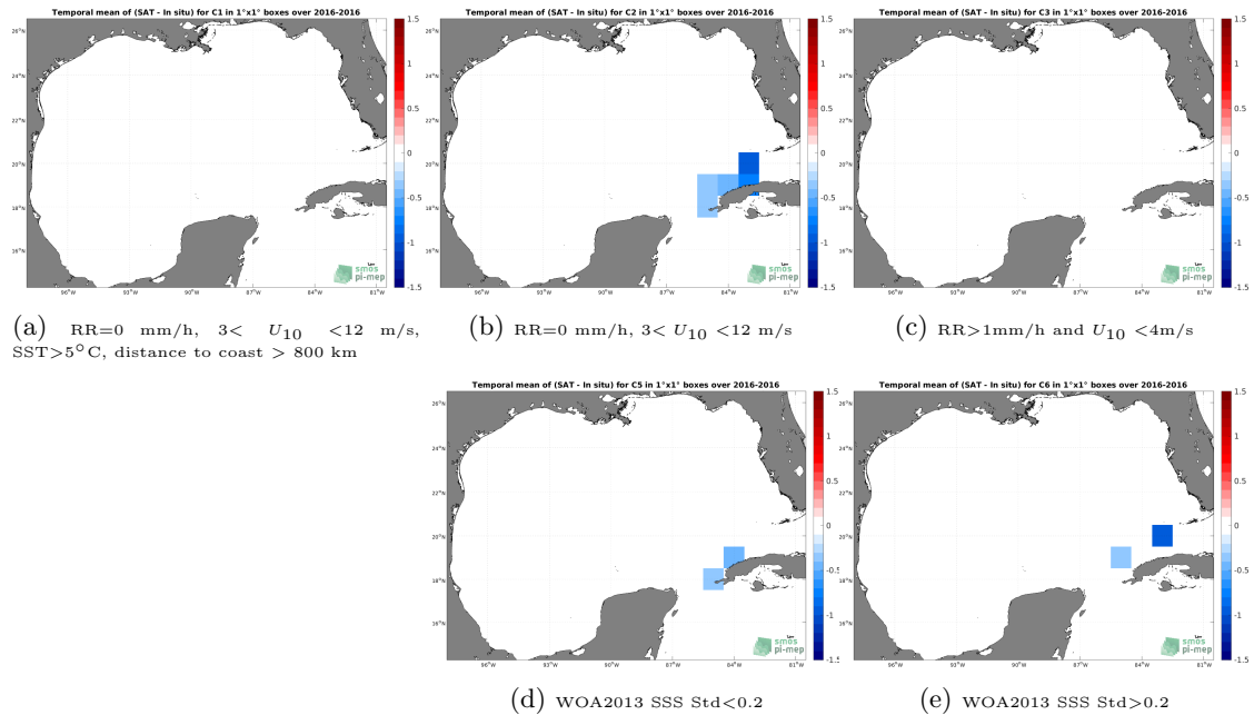
Figure 12: Temporal mean gridded over spatial boxes of size 1^{\circ}\times 1^{\circ} of \Delta\text{SSS} (SMAP SSS L3 v5.0 - Monthly (JPL) - TSG (LEGOS-DM)) for 5 different subdatasets corresponding to:RR=0 mm/h, 3 < U_{10} < 12 m/s, SST >5^{\circ}\text{C} , distance to coast > 800 km (a), RR=0 mm/h, 3 < U_{10} < 12 m/s (b), RR >1 mm/h and U_{10} < 4 m/s (c), WOA2013 SSS Std <0.2 (d), WOA2013 SSS Std >0.2 (e).
