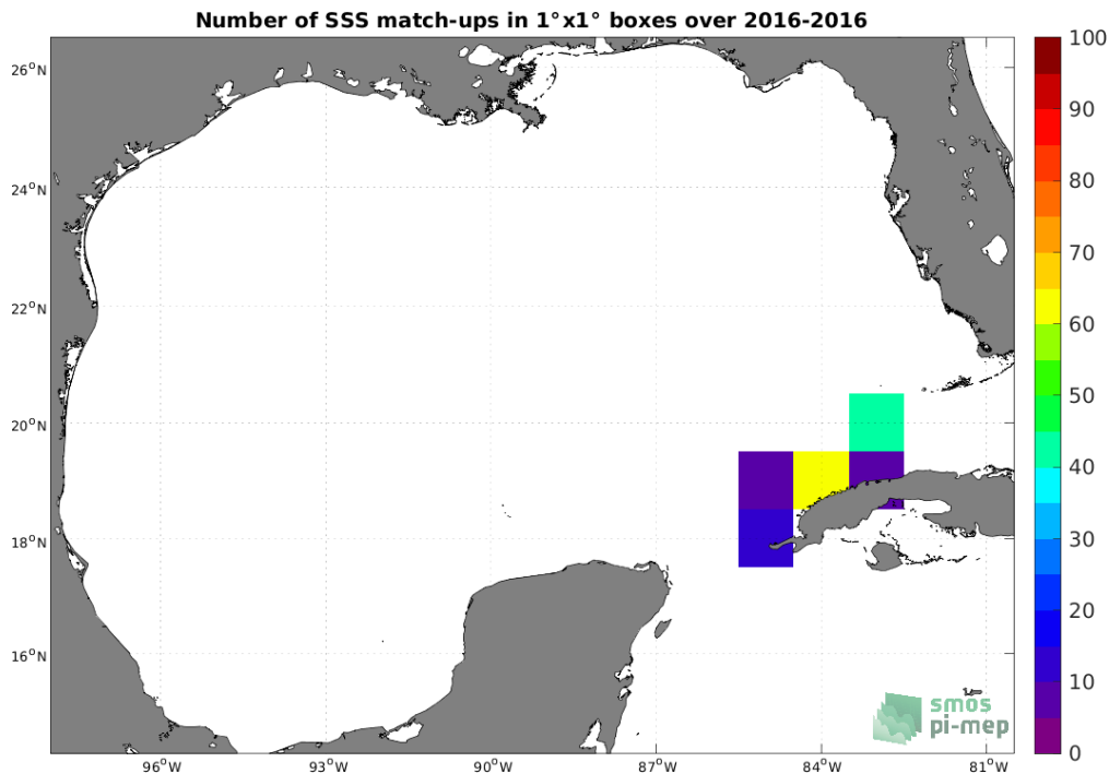
Figure 4: Number of SSS match-ups between TSG (LEGOS-DM) SSS and the SMAP SSS L3 v5.0 - Monthly (JPL) SSS product for the Gulf of Mexico Pi-MEP region over 1^\circ \times 1^\circ boxes and for the full satellite product period.
