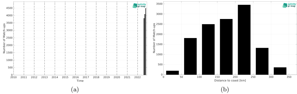
Figure 2: Number of match-ups between Saildrone and SMAP SSS L3 v5.0 - Monthly (JPL) SSS as a function of time (a) and as function of the distance to coast (b) over the Gulf of Mexico Pi-MEP region and for the full satellite product period.
