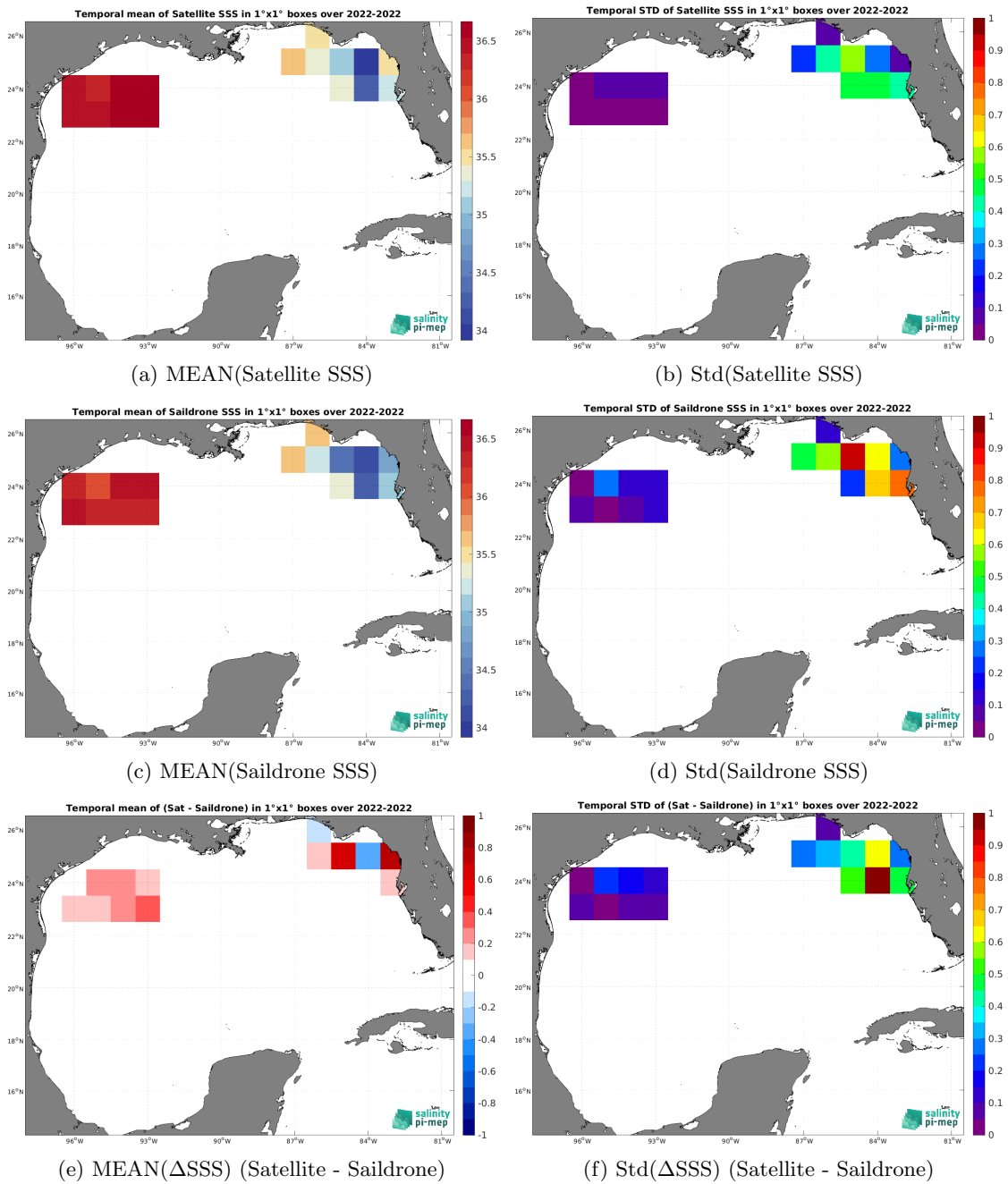
Figure 7: Temporal mean (left) and Std (right) of SSS from SMAP SSS L3 v5.0 - Monthly (JPL) (top), Saildrone (middle), and of \Delta SSS (Satellite - Saildrone). Only match-up pairs are used to generate these maps.
