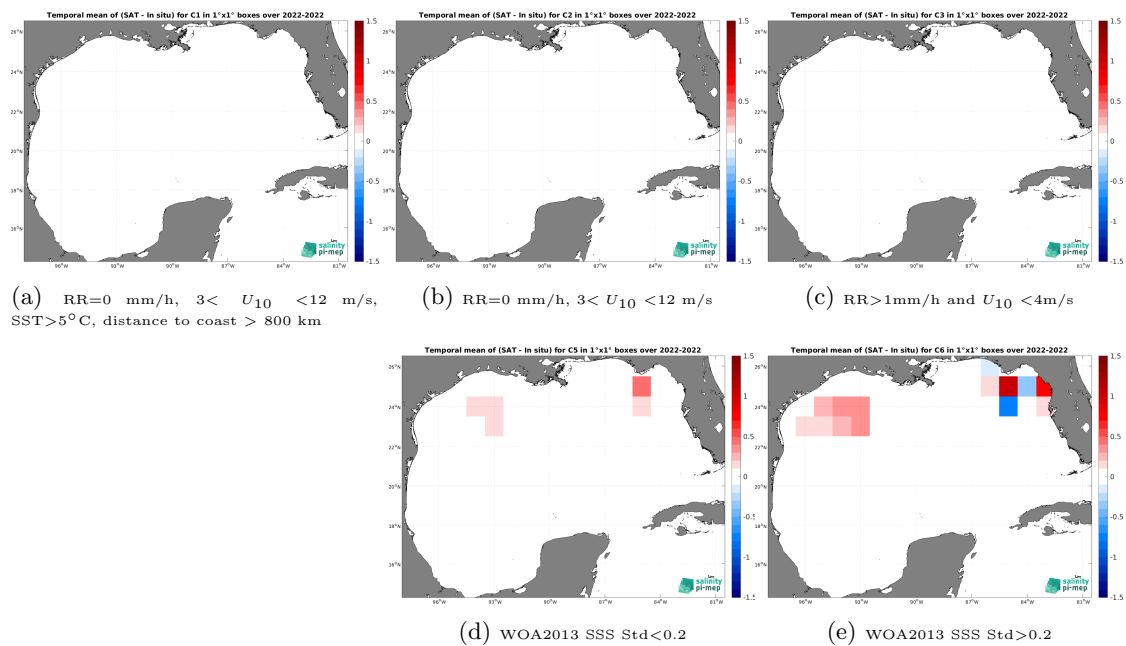
Figure 14: Temporal mean gridded over spatial boxes of size 1^\circ \times 1^\circ of \Delta SSS (SMAP SSS L3 v5.0 - Monthly (JPL) - Saildrone) for 5 different subdatasets corresponding to:RR=0 mm/h, 3 < U_{10} < 12 m/s, SST >5^\circ\text{C} , distance to coast > 800 km (a), RR=0 mm/h, 3 < U_{10} < 12 m/s (b), RR >1 mm/h and U_{10} < 4 m/s (c), WOA2013 SSS Std <0.2 (d), WOA2013 SSS Std >0.2 (e).
