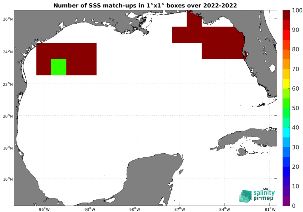
Figure 5: Number of SSS match-ups between Saildrone SSS and the SMAP SSS L3 v5.0 - Monthly (JPL) SSS product for the Gulf of Mexico Pi-MEP region over 1°×1° boxes and for the full satellite product period.
