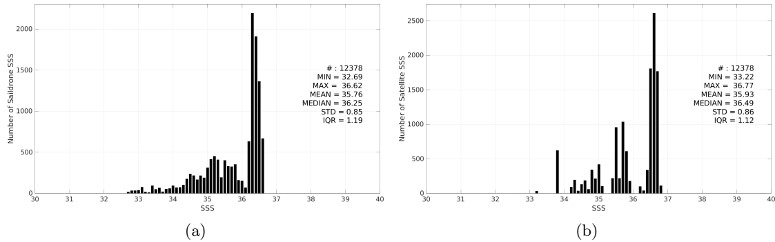
Figure 3: Histograms of SSS from Saildrone (a) and SMAP SSS L3 v5.0 - Monthly (JPL) (b) considering all match-up pairs per bins of 0.1 over the Gulf of Mexico Pi-MEP region and for the full satellite product period.
