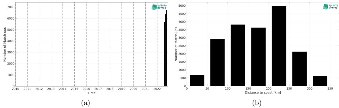
Figure 1: Number of match-ups between Saildrone and SMAP SSS L3 v5.0 - Monthly (JPL) SSS as a function of time (a) and as function of the distance to coast (b) over the Gulf of Mexico Pi-MEP region and for the full satellite product period.
