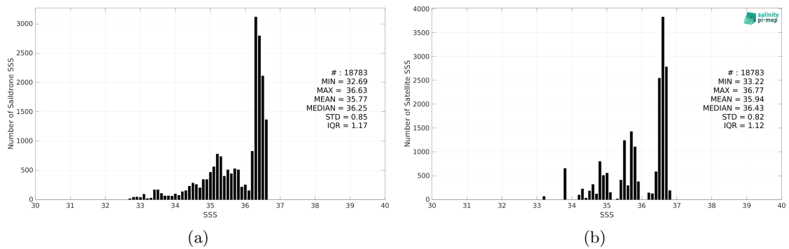
Figure 2: Histograms of SSS from Saildrone (a) and SMAP SSS L3 v5.0 - Monthly (JPL) (b) considering all match-up pairs per bins of 0.1 over the Gulf of Mexico Pi-MEP region and for the full satellite product period.
