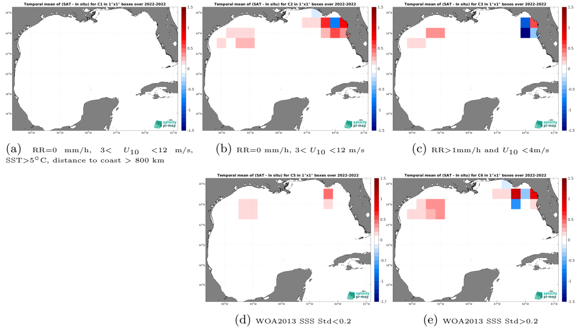
Figure 12: Temporal mean gridded over spatial boxes of size 1^{\circ}\times 1^{\circ} of \Delta\text{SSS} (SMAP SSS L3 v5.0 - Monthly (JPL) - Saildrone) for 5 different subdatasets corresponding to:RR=0 mm/h, 3 < U_{10} < 12 m/s, SST >5^{\circ}\text{C} , distance to coast > 800 km (a), RR=0 mm/h, 3 < U_{10} < 12 m/s (b), RR >1 mm/h and U_{10} < 4 m/s (c), WOA2013 SSS Std <0.2 (d), WOA2013 SSS Std >0.2 (e).
