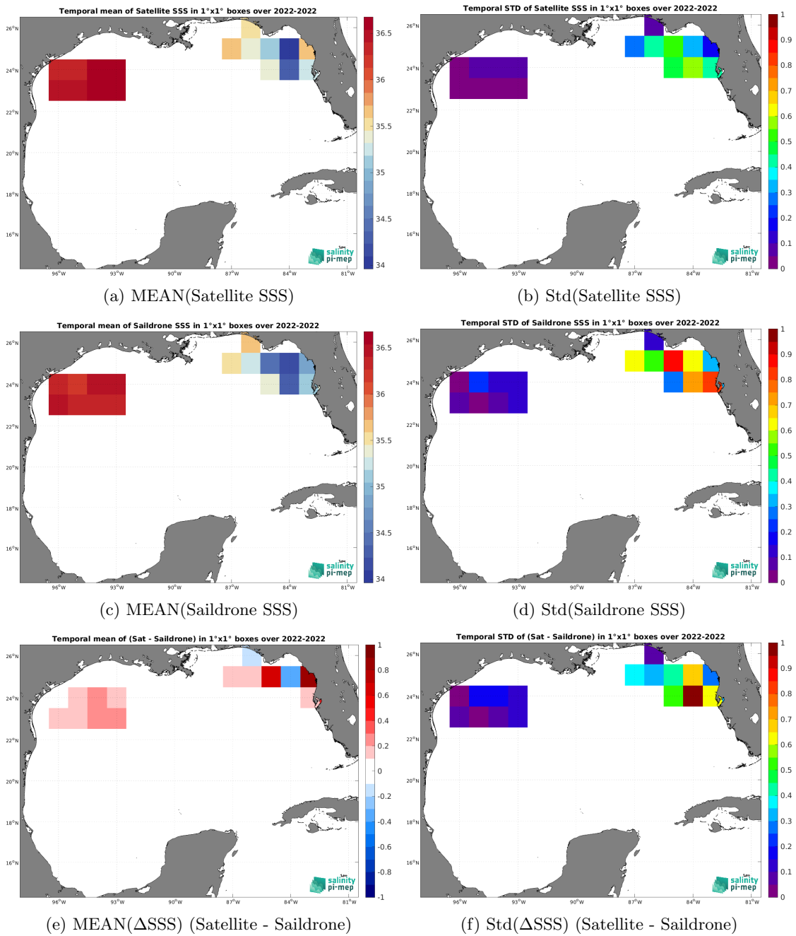
Figure 6: Temporal mean (left) and Std (right) of SSS from SMAP SSS L3 v5.0 - Monthly (JPL) (top), Saildrone (middle), and of \Delta SSS (Satellite - Saildrone). Only match-up pairs are used to generate these maps.
