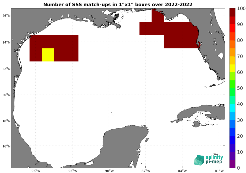
Figure 4: Number of SSS match-ups between Saildrone SSS and the SMAP SSS L3 v5.0 - Monthly (JPL) SSS product for the Gulf of Mexico Pi-MEP region over 1^\circ \times 1^\circ boxes and for the full satellite product period.
