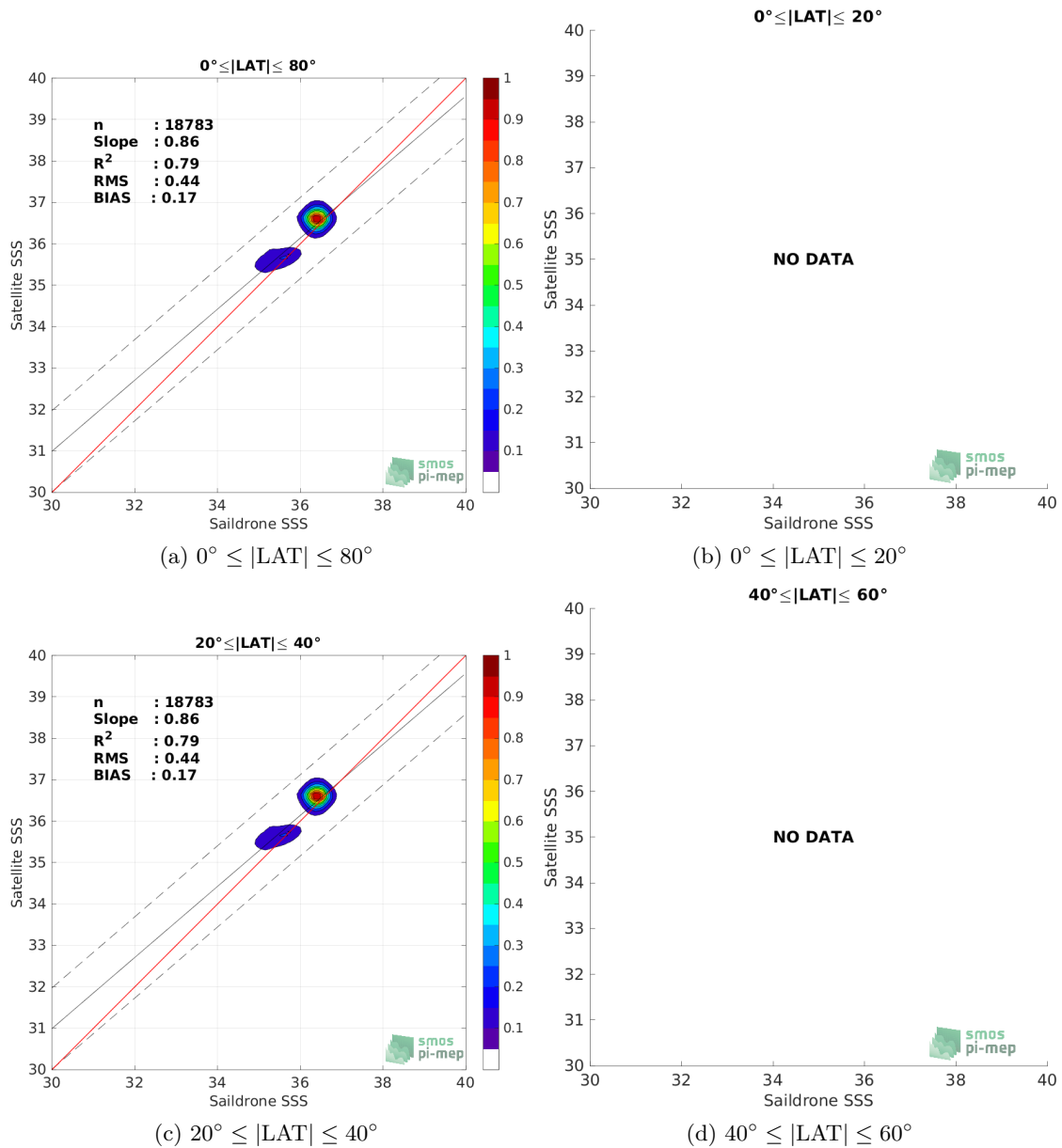
Figure 9: Contour maps of the concentration of SMAP SSS L3 v5.0 - Monthly (JPL) SSS (y-axis) versus Sailldrone SSS (x-axis) at match-up pairs for different latitude bands. For each plot, the red line shows x=y . The black thin and dashed lines indicate a linear fit through the data cloud and the \pm 95\% confidence levels, respectively. The number match-up pairs n , the slope and R^2 coefficient of the linear fit, the root mean square (RMS) and the mean bias between satellite and in situ data are indicated for each latitude band in each plots.
