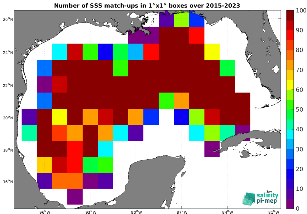
Figure 4: Number of SSS match-ups between Argo SSS and the SMAP SSS L3 v5.0 - Monthly (JPL) SSS product for the Gulf of Mexico Pi-MEP region over 1^\circ \times 1^\circ boxes and for the full satellite product period.
