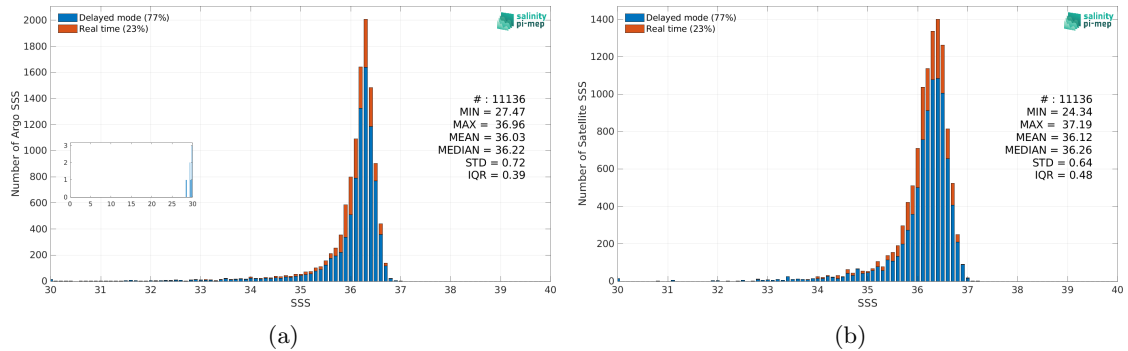
Figure 2: Histograms of SSS from Argo (a) and SMAP SSS L3 v5.0 - Monthly (JPL) (b) considering all match-up pairs per bins of 0.1 over the Gulf of Mexico Pi-MEP region and for the full satellite product period.
