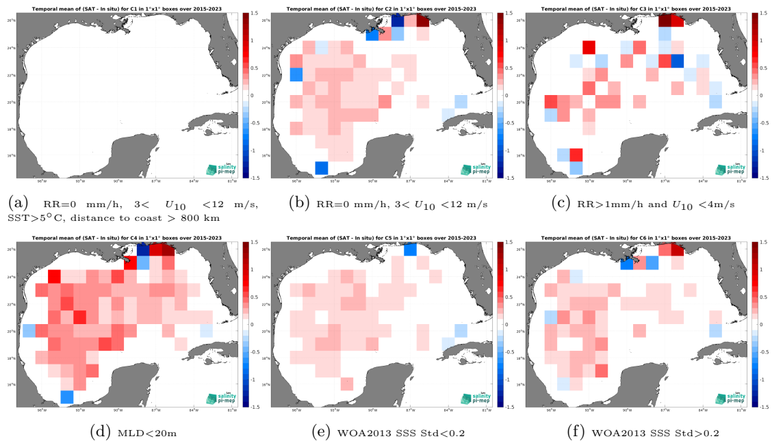
Figure 12: Temporal mean gridded over spatial boxes of size 1^\circ \times 1^\circ of \Delta SSS (SMAP SSS L3 v5.0 - Monthly (JPL) - Argo) for 6 different subdatasets corresponding to:RR=0 mm/h, 3 < U_{10} < 12 m/s, SST > 5^\circ\text{C} , distance to coast > 800 km (a), RR=0 mm/h, 3 < U_{10} < 12 m/s (b), RR > 1 mm/h and U_{10} < 4 m/s (c),MLD < 20 m (d),WOA2013 SSS Std < 0.2 (e),WOA2013 SSS Std > 0.2 (f).
