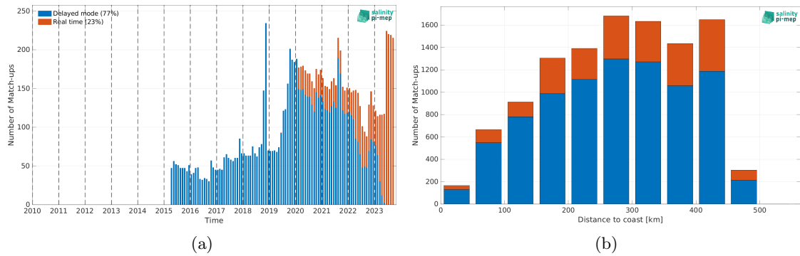
Figure 1: Number of match-ups between Argo and SMAP SSS L3 v5.0 - Monthly (JPL) SSS as a function of time (a) and as function of the distance to coast (b) over the Gulf of Mexico Pi-MEP region and for the full satellite product period.
