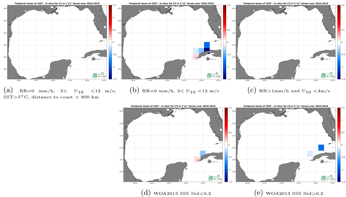
Figure 12: Temporal mean gridded over spatial boxes of size 1^{\circ}\times 1^{\circ} of \Delta\text{SSS} (SMAP-L3-JPL-V4.3-8DAY-RUNNING-60KM - TSG-LEGOS-DM) for 5 different subdatasets corresponding to:RR=0 mm/h, 3 < U_{10} < 12 m/s, SST >5^{\circ}\text{C} , distance to coast > 800 km (a), RR=0 mm/h, 3 < U_{10} < 12 m/s (b), RR >1 mm/h and U_{10} < 4 m/s (c), WOA2013 SSS Std <0.2 (d), WOA2013 SSS Std >0.2 (e).
