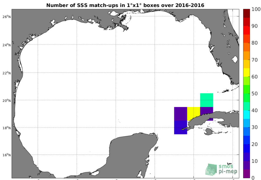
Figure 4: Number of SSS match-ups between TSG-LEGOS-DM SSS and the SMAP-L3-JPL-V4.3-8DAY-RUNNING-60KM SSS product for the Gulf of Mexico Pi-MEP region over 1°x1° boxes and for the full satellite product period.
