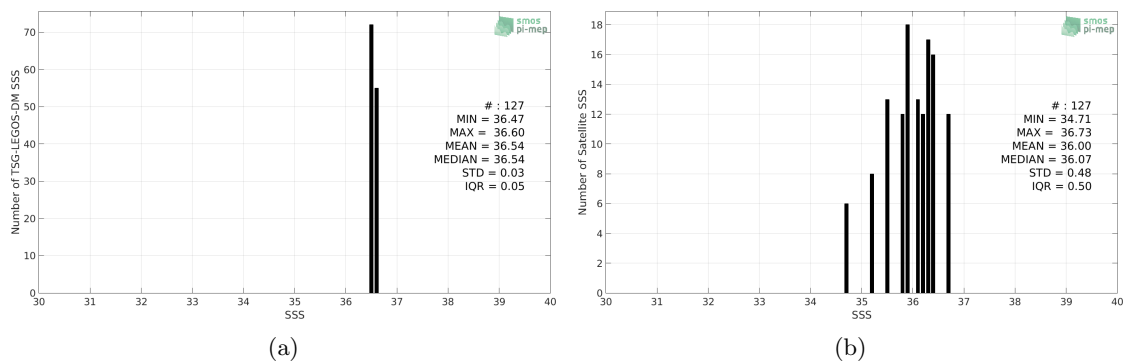
Figure 2: Histograms of SSS from TSG-LEGOS-DM (a) and SMAP-L3-JPL-V4.3-8DAY-RUNNING-60KM (b) considering all match-up pairs per bins of 0.1 over the Gulf of Mexico Pi-MEP region and for the full satellite product period.
