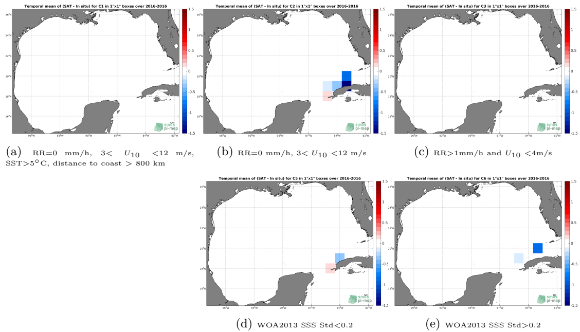
Figure 12: Temporal mean gridded over spatial boxes of size 1^\circ \times 1^\circ of \Delta SSS (SMAP-L3-JPL-V4.3-8DAY-RUNNING-60KM - TSG-LEGOS-DM) for 5 different subdatasets corresponding to: RR=0 mm/h, 3 < U_{10} < 12 m/s, SST > 5^\circ\text{C} , distance to coast > 800 km (a), RR=0 mm/h, 3 < U_{10} < 12 m/s (b), RR > 1 mm/h and U_{10} < 4 m/s (c), WOA2013 SSS Std < 0.2 (d), WOA2013 SSS Std > 0.2 (e).
