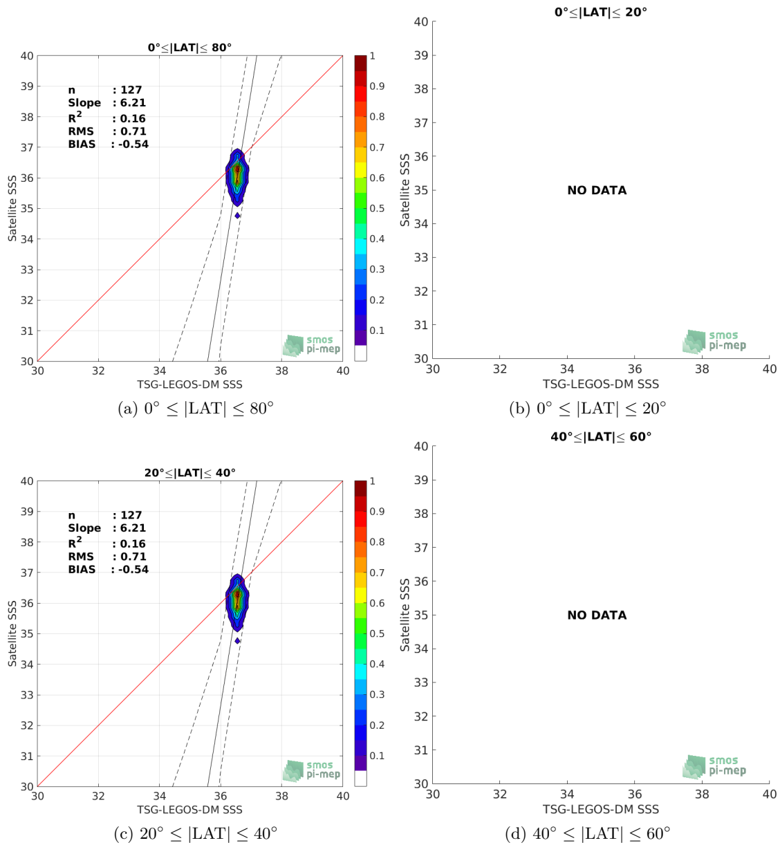
Figure 9: Contour maps of the concentration of SMAP-L3-JPL-V4.3-8DAY-RUNNING-60KM SSS (y-axis) versus TSG-LEGOS-DM SSS (x-axis) at match-up pairs for different latitude bands. For each plot, the red line shows x=y . The black thin and dashed lines indicate a linear fit through the data cloud and the \pm 95\% confidence levels, respectively. The number match-up pairs n , the slope and R^2 coefficient of the linear fit, the root mean square (RMS) and the mean bias between satellite and in situ data are indicated for each latitude band in each plots.
