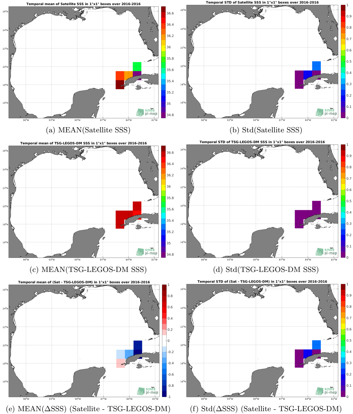
Figure 6: Temporal mean (left) and Std (right) of SSS from SMAP-L3-JPL-V4.3-8DAY-RUNNING-60KM (top), TSG-LEGOS-DM (middle), and of \Delta SSS (Satellite - TSG-LEGOS-DM). Only match-up pairs are used to generate these maps.
