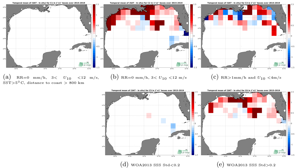
Figure 12: Temporal mean gridded over spatial boxes of size 1^{\circ}\times 1^{\circ} of \Delta\text{SSS} (SMAP-L3-JPL-V4.3-MONTHLY-60KM - TSG-SAMOS) for 5 different subdatasets corresponding to:RR=0 mm/h, 3 < U_{10} < 12 m/s, SST >5^{\circ}\text{C} , distance to coast > 800 km (a), RR=0 mm/h, 3 < U_{10} < 12 m/s (b), RR >1 mm/h and U_{10} < 4 m/s (c), WOA2013 SSS Std <0.2 (d), WOA2013 SSS Std >0.2 (e).
