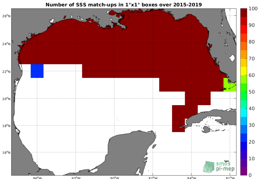
Figure 4: Number of SSS match-ups between TSG-SAMOS SSS and the SMAP-L3-JPL-V4.3-MONTHLY-60KM SSS product for the Gulf of Mexico Pi-MEP region over 1°x1° boxes and for the full satellite product period.
