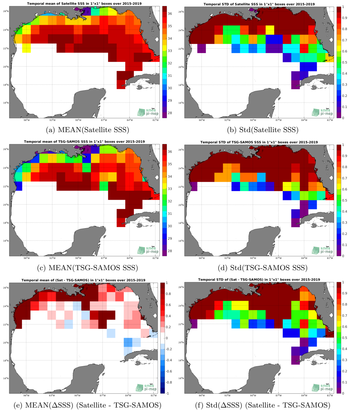
Figure 6: Temporal mean (left) and Std (right) of SSS from SMAP-L3-JPL-V4.3-MONTHLY-60KM (top), TSG-SAMOS (middle), and of \Delta SSS (Satellite - TSG-SAMOS). Only match-up pairs are used to generate these maps.
