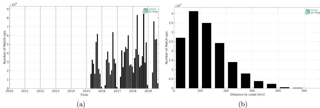
Figure 1: Number of match-ups between TSG-SAMOS and SMAP-L3-JPL-V4.3-MONTHLY-60KM SSS as a function of time (a) and as function of the distance to coast (b) over the Gulf of Mexico Pi-MEP region and for the full satellite product period.
