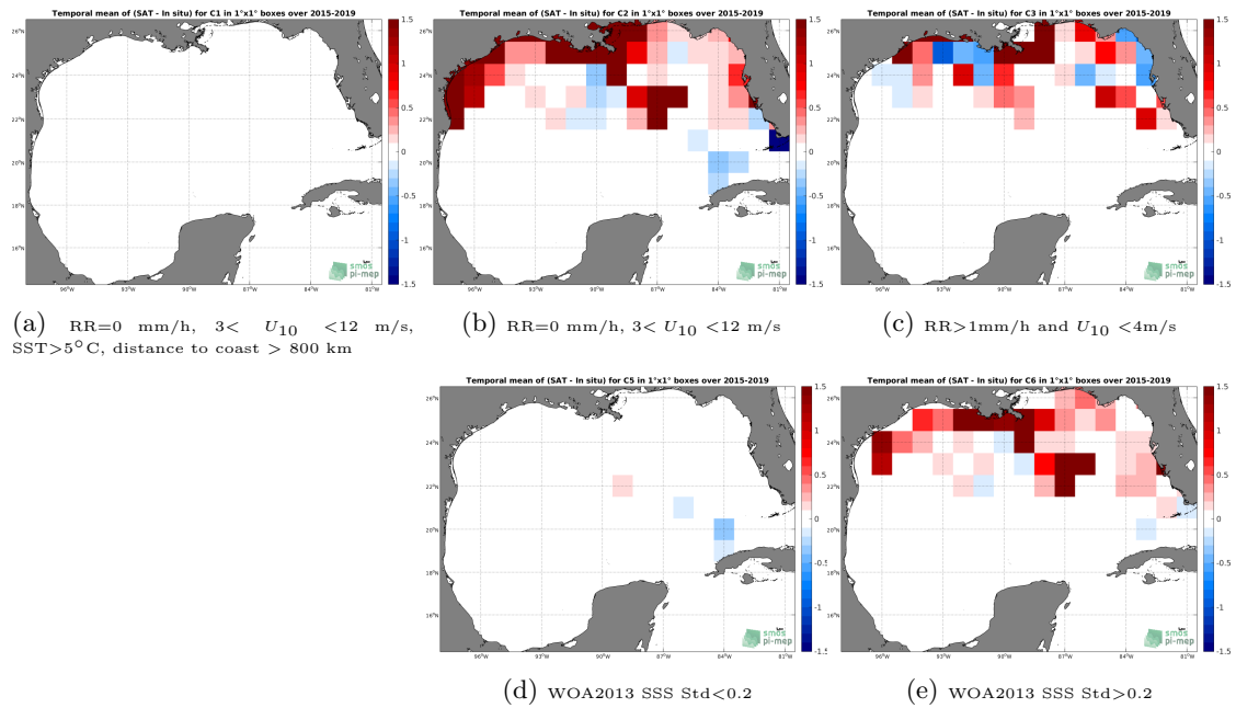
Figure 12: Temporal mean gridded over spatial boxes of size 1^\circ \times 1^\circ of \Delta SSS (SMAP-L3-JPL-V4.3-MONTHLY-60KM - TSG-SAMOS) for 5 different subdatasets corresponding to:RR=0 mm/h, 3 < U_{10} < 12 m/s, SST >5^\circ\text{C} , distance to coast > 800 km (a), RR=0 mm/h, 3 < U_{10} < 12 m/s (b), RR >1 mm/h and U_{10} < 4 m/s (c), WOA2013 SSS Std <0.2 (d), WOA2013 SSS Std >0.2 (e).
