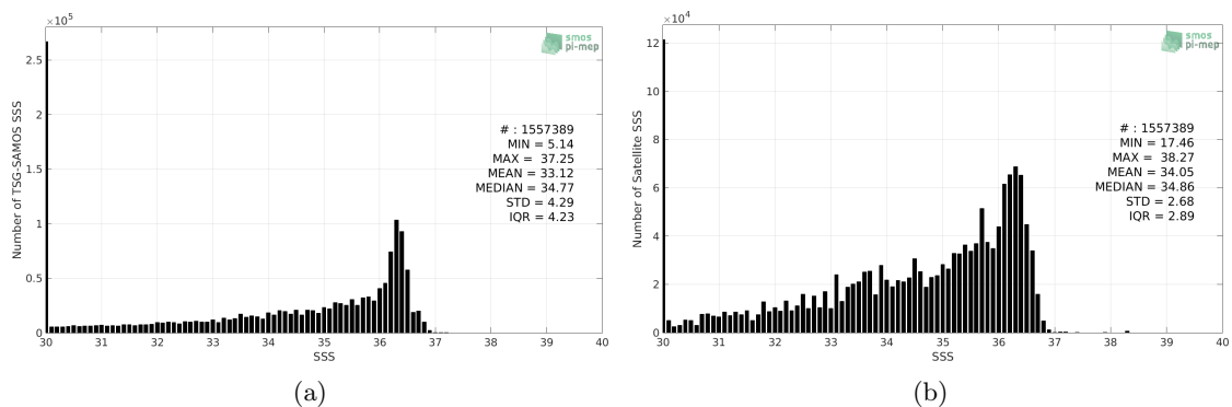
Figure 2: Histograms of SSS from TSG-SAMOS (a) and SMAP-L3-JPL-V4.3-MONTHLY-60KM (b) considering all match-up pairs per bins of 0.1 over the Gulf of Mexico Pi-MEP region and for the full satellite product period.
