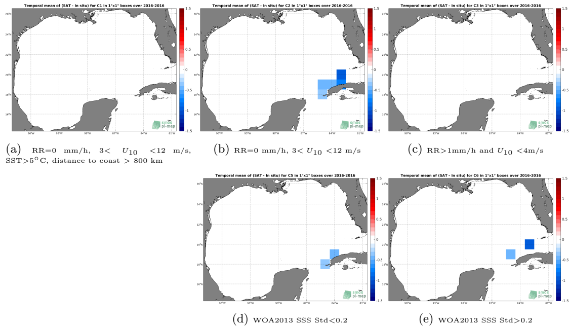
Figure 12: Temporal mean gridded over spatial boxes of size 1^{\circ}\times 1^{\circ} of \Delta\text{SSS} (SMAP-L3-JPL-V4.3-MONTHLY-60KM - TSG-LEGOS-DM) for 5 different subdatasets corresponding to:RR=0 mm/h, 3 < U_{10} < 12 m/s, SST >5^{\circ}\text{C} , distance to coast > 800 km (a), RR=0 mm/h, 3 < U_{10} < 12 m/s (b), RR >1 mm/h and U_{10} < 4 m/s (c), WOA2013 SSS Std <0.2 (d), WOA2013 SSS Std >0.2 (e).
