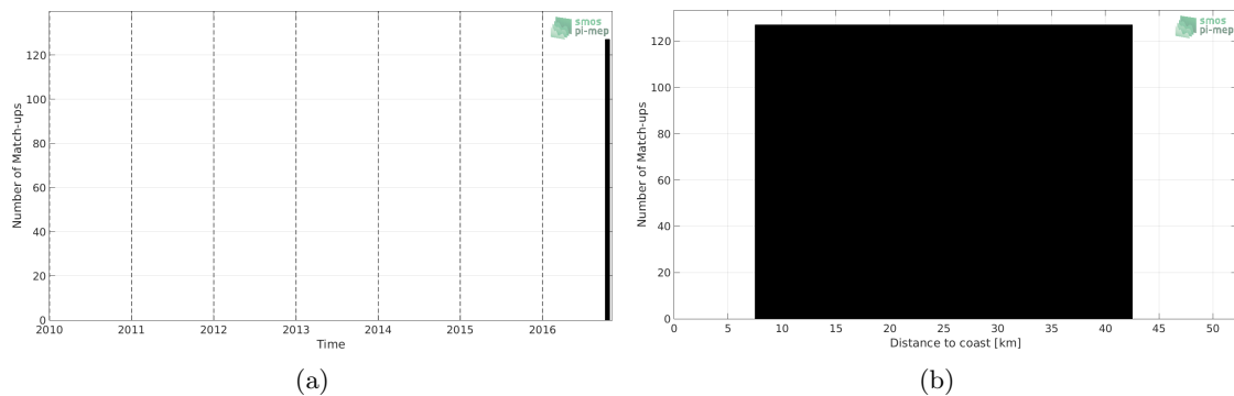
Figure 1: Number of match-ups between TSG-LEGOS-DM and SMAP-L3-JPL-V4.3-MONTHLY-60KM SSS as a function of time (a) and as function of the distance to coast (b) over the Gulf of Mexico Pi-MEP region and for the full satellite product period.
