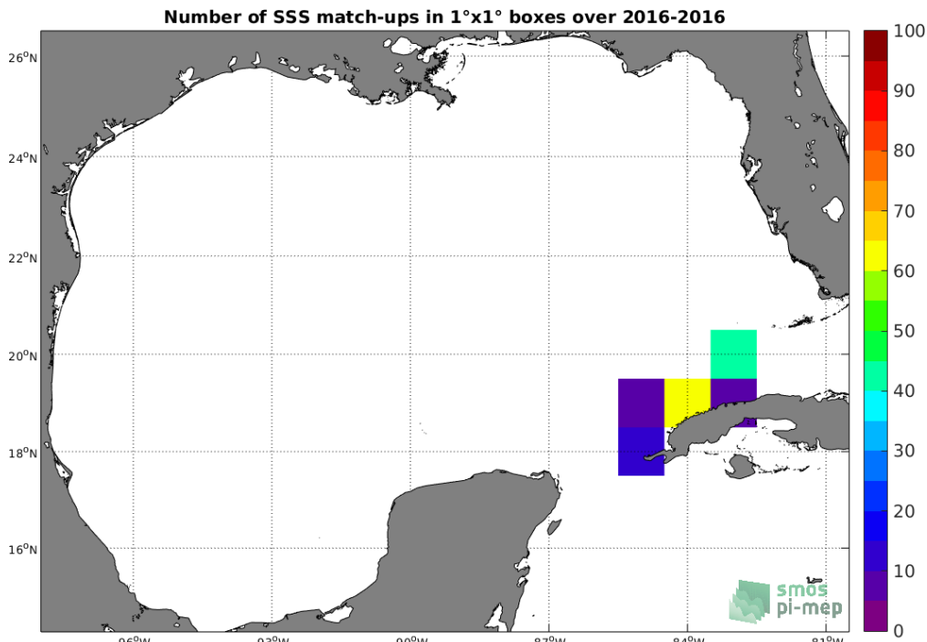
Figure 4: Number of SSS match-ups between TSG-LEGOS-DM SSS and the SMAP-L3-JPL-V4.3-MONTHLY-60KM SSS product for the Gulf of Mexico Pi-MEP region over 1°x1° boxes and for the full satellite product period.
