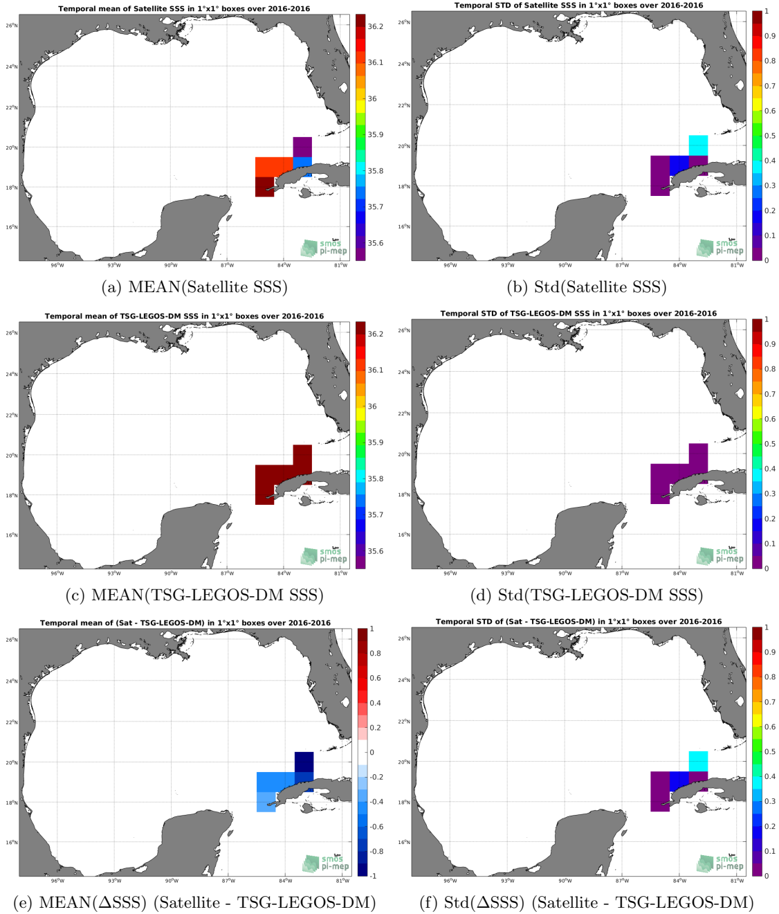
Figure 6: Temporal mean (left) and Std (right) of SSS from SMAP-L3-JPL-V4.3-MONTHLY-60KM (top), TSG-LEGOS-DM (middle), and of \Delta SSS (Satellite - TSG-LEGOS-DM). Only match-up pairs are used to generate these maps.
