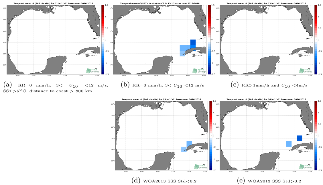
Figure 12: Temporal mean gridded over spatial boxes of size 1^\circ \times 1^\circ of \Delta SSS (SMAP-L3-JPL-V4.3-MONTHLY-60KM - TSG-LEGOS-DM) for 5 different subdatasets corresponding to:RR=0 mm/h, 3 < U_{10} < 12 m/s, SST >5^\circ\text{C} , distance to coast > 800 km (a), RR=0 mm/h, 3 < U_{10} < 12 m/s (b), RR >1 mm/h and U_{10} < 4 m/s (c), WOA2013 SSS Std <0.2 (d), WOA2013 SSS Std >0.2 (e).
