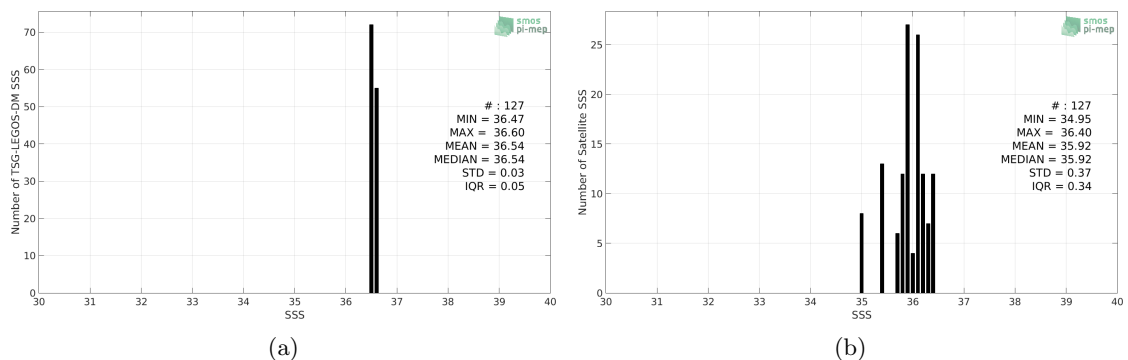
Figure 2: Histograms of SSS from TSG-LEGOS-DM (a) and SMAP-L3-JPL-V4.3-MONTHLY-60KM (b) considering all match-up pairs per bins of 0.1 over the Gulf of Mexico Pi-MEP region and for the full satellite product period.
