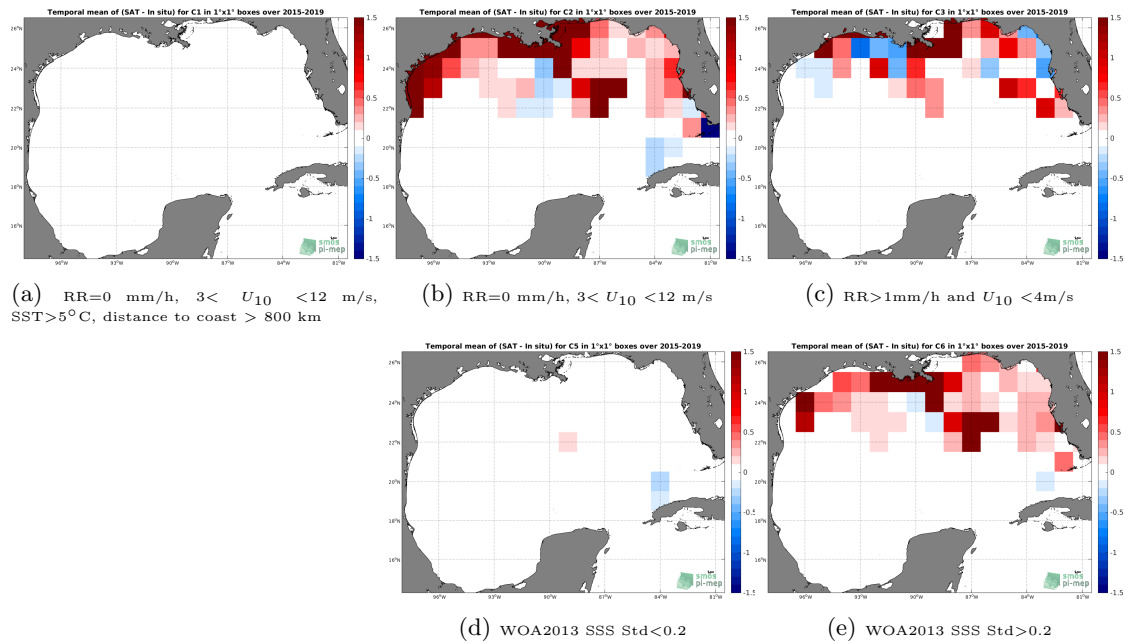
Figure 12: Temporal mean gridded over spatial boxes of size 1^\circ \times 1^\circ of \Delta SSS (SMAP-L3-JPL-V4.2-MONTHLY-60KM - TSG-SAMOS) for 5 different subdatasets corresponding to:RR=0 mm/h, 3 < U_{10} < 12 m/s, SST >5^\circ C, distance to coast > 800 km (a), RR=0 mm/h, 3 < U_{10} < 12 m/s (b), RR >1 mm/h and U_{10} < 4 m/s (c), WOA2013 SSS Std <0.2 (d), WOA2013 SSS Std >0.2 (e).
