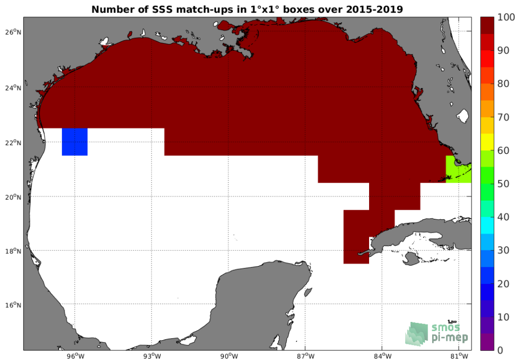
Figure 4: Number of SSS match-ups between TSG-SAMOS SSS and the SMAP-L3-JPL-V4.2-MONTHLY-60KM SSS product for the Gulf of Mexico Pi-MEP region over 1^\circ \times 1^\circ boxes and for the full satellite product period.
