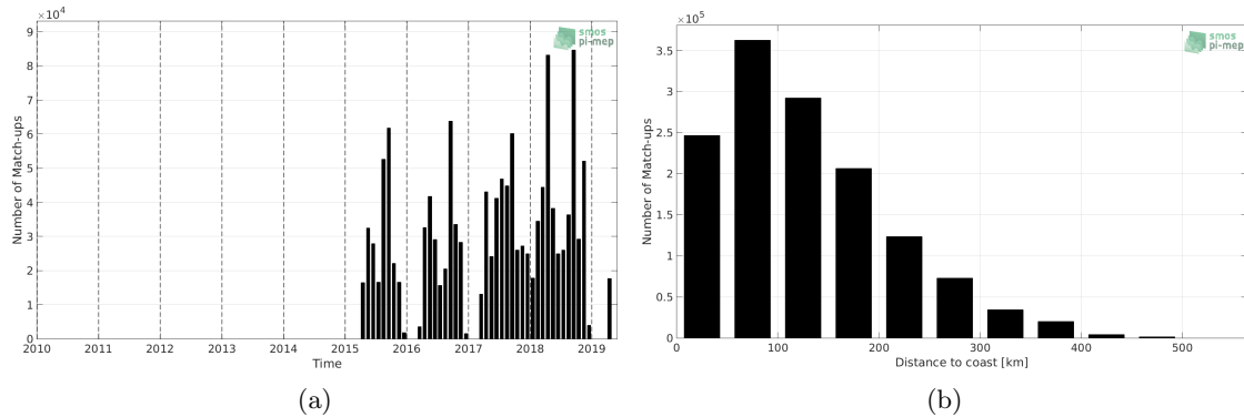
Figure 1: Number of match-ups between TSG-SAMOS and SMAP-L3-JPL-V4.2-MONTHLY-60KM SSS as a function of time (a) and as function of the distance to coast (b) over the Gulf of Mexico Pi-MEP region and for the full satellite product period.
