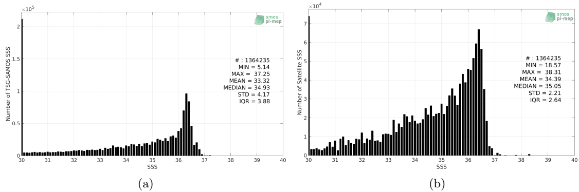
Figure 2: Histograms of SSS from TSG-SAMOS (a) and SMAP-L3-JPL-V4.2-MONTHLY-60KM (b) considering all match-up pairs per bins of 0.1 over the Gulf of Mexico Pi-MEP region and for the full satellite product period.
