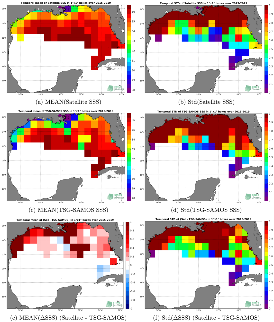
Figure 6: Temporal mean (left) and Std (right) of SSS from SMAP-L3-JPL-V4.2-MONTHLY-60KM (top), TSG-SAMOS (middle), and of \Delta SSS (Satellite - TSG-SAMOS). Only match-up pairs are used to generate these maps.
