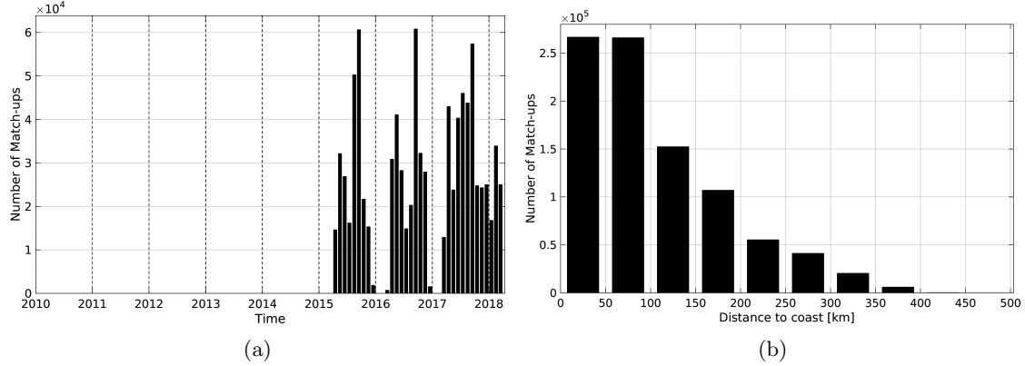
Figure 1: Number of match-ups between TSG-SAMOS and SMAP-L3-JPL-V4-8DAY-RUNNING-60KM SSS as a function of time (a) and as function of the distance to coast (b) over the Gulf of Mexico Pi-MEP region and for the full satellite product period.
