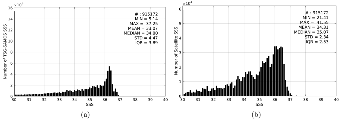
Figure 2: Histograms of SSS from TSG-SAMOS (a) and SMAP-L3-JPL-V4-8DAY-RUNNING-60KM (b) considering all match-up pairs per bins of 0.1 over the Gulf of Mexico Pi-MEP region and for the full satellite product period.
