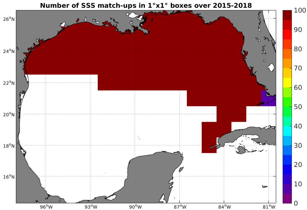
Figure 4: Number of SSS match-ups between TSG-SAMOS SSS and the SMAP-L3-JPL-V4-8DAY-RUNNING-60KM SSS product for the Gulf of Mexico Pi-MEP region over 1°x1° boxes and for the full satellite product period.
