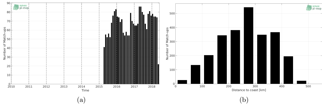
Figure 1: Number of match-ups between Argo and SMAP-L3-JPL-V4-8DAY-RUNNING-60KM SSS as a function of time (a) and as function of the distance to coast (b) over the Gulf of Mexico Pi-MEP region and for the full satellite product period.
