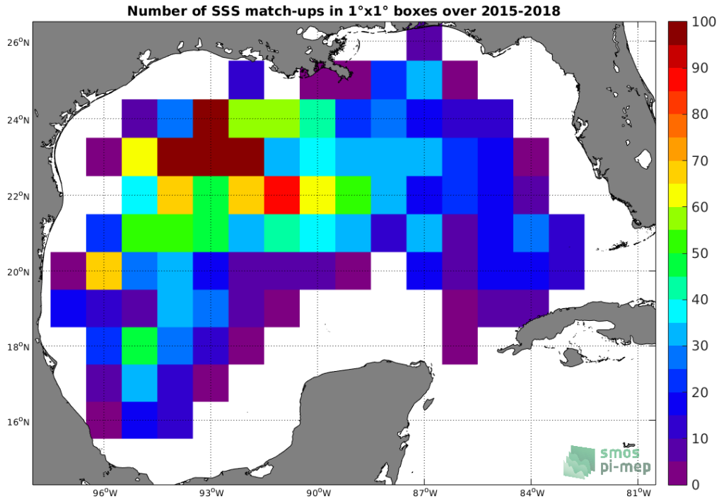
Figure 4: Number of SSS match-ups between Argos SSS and the SMAP-L3-JPL-V4-8DAY-RUNNING-60KM SSS product for the Gulf of Mexico Pi-MEP region over 1^\circ \times 1^\circ boxes and for the full satellite product period.
