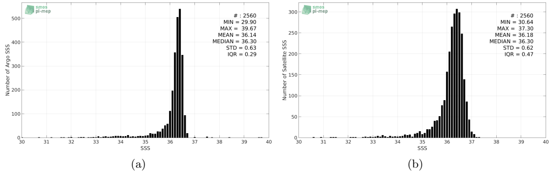
Figure 2: Histograms of SSS from Argo (a) and SMAP-L3-JPL-V4-8DAY-RUNNING-60KM (b) considering all match-up pairs per bins of 0.1 over the Gulf of Mexico Pi-MEP region and for the full satellite product period.
