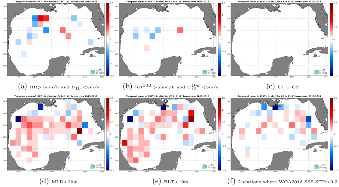
Figure 12: Temporal mean gridded over spatial boxes of size 1^\circ \times 1^\circ of \Delta\text{SSS} (SMAP-L3-JPL-V4-8DAY-RUNNING-60KM - Argo) for 6 different subdatasets corresponding to: RR > 1\text{mm/h} and U_{10} < 5\text{m/s} (a), RR^{10d} > 5\text{mm/h} and U_{10}^{10d} < 5\text{m/s} (b), C1 U C2 (c), MLD < 20\text{m} (d), BLT > 10\text{m} (e), Locations where WOA2013 SSS STD > 0.2 (f).
