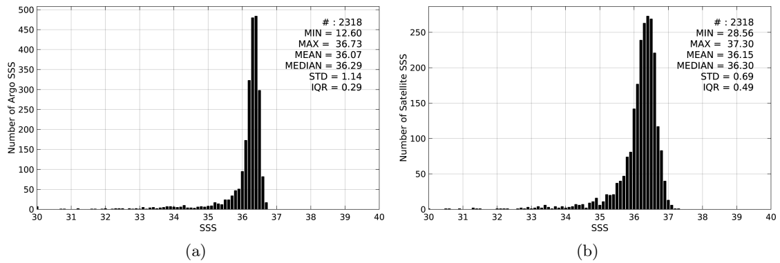
Figure 2: Histograms of SSS from Argo (a) and SMAP-L3-JPL-V4-8DAY-RUNNING-60KM (b) considering all match-up pairs per bins of 0.1 over the Gulf of Mexico Pi-MEP region and for the full satellite product period.
