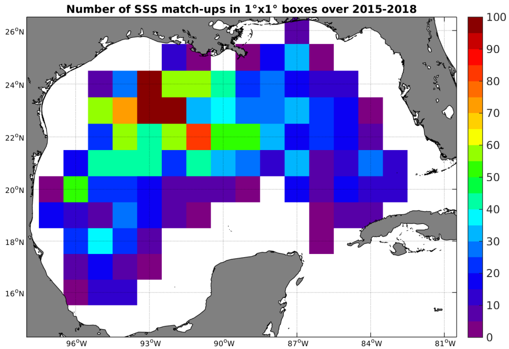
Figure 4: Number of SSS match-ups between Argo SSS and the SMAP-L3-JPL-V4-8DAY-RUNNING-60KM SSS product for the Gulf of Mexico Pi-MEP region over 1^\circ \times 1^\circ boxes and for the full satellite product period.
