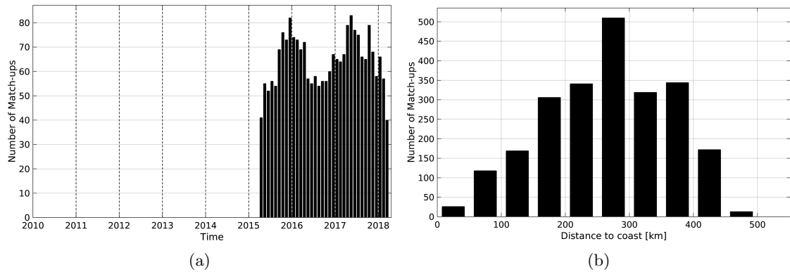
Figure 1: Number of match-ups between Argo and SMAP-L3-JPL-V4-8DAY-RUNNING-60KM SSS as a function of time (a) and as function of the distance to coast (b) over the Gulf of Mexico Pi-MEP region and for the full satellite product period.
