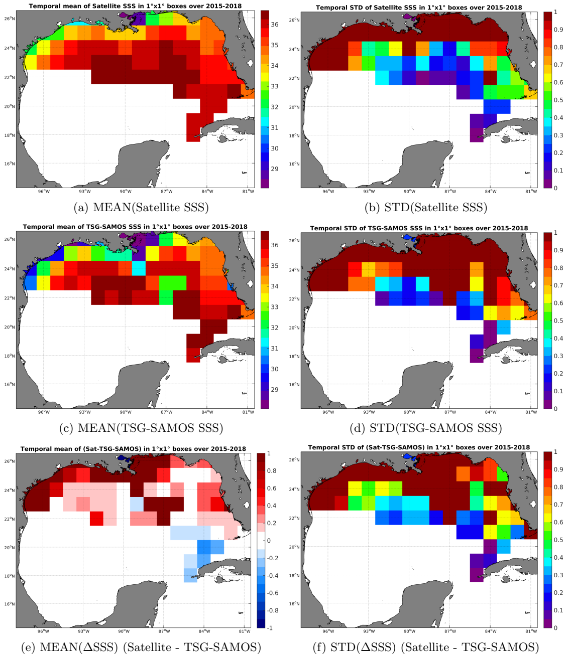
Figure 6: Temporal mean (left) and STD (right) of SSS from SMAP-L3-JPL-V4-MONTHLY-60KM (top), TSG-SAMOS (middle), and of \Delta SSS (Satellite - TSG-SAMOS). Only match-up pairs are used to generate these maps.
