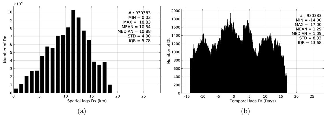
Figure 5: Histograms of the spatial (a) and temporal (b) lags between the time of the TSG-SAMOS measurements and the date of the corresponding SMAP-L3-JPL-V4-MONTHLY-60KM SSS product.
