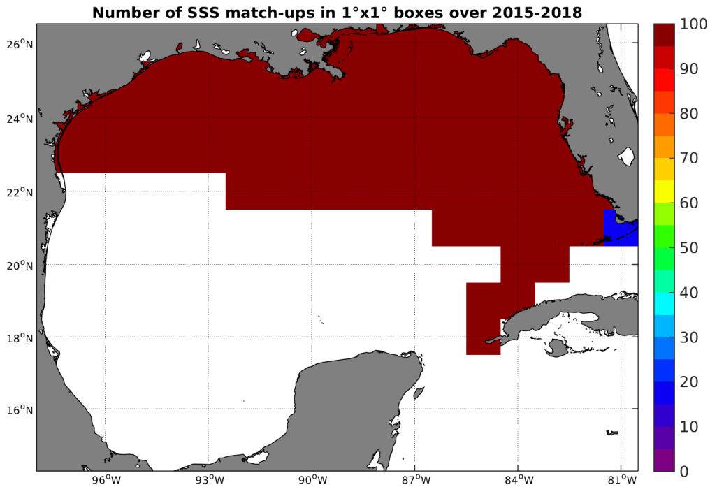
Figure 4: Number of SSS match-ups between TSG-SAMOS SSS and the SMAP-L3-JPL-V4-MONTHLY-60KM SSS product for the Gulf of Mexico Pi-MEP region over 1^\circ \times 1^\circ boxes and for the full satellite product period.
