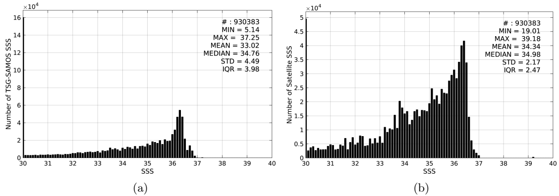
Figure 2: Histograms of SSS from TSG-SAMOS (a) and SMAP-L3-JPL-V4-MONTHLY-60KM (b) considering all match-up pairs per bins of 0.1 over the Gulf of Mexico Pi-MEP region and for the full satellite product period.
