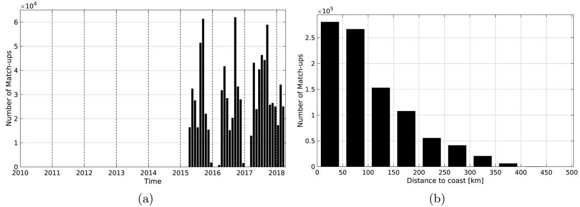
Figure 1: Number of match-ups between TSG-SAMOS and SMAP-L3-JPL-V4-MONTHLY-60KM SSS as a function of time (a) and as function of the distance to coast (b) over the Gulf of Mexico Pi-MEP region and for the full satellite product period.
