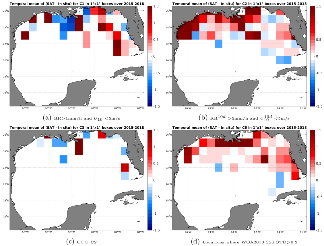
Figure 12: Temporal mean gridded over spatial boxes of size 1^\circ \times 1^\circ of \Delta SSS (SMAP-L3-JPL-V4-MONTHLY-60KM - TSG-SAMOS) for 4 different subdatasets corresponding to:RR > 1 mm/h and U_{10} < 5 m/s (a), RR 10d > 5 mm/h and U_{10}^{10d} < 5 m/s (b), C1 U C2 (c),Locations where WOA2013 SSS STD > 0.2 (d).
