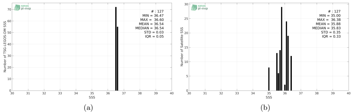
Figure 2: Histograms of SSS from TSG-LEGOS-DM (a) and SMAP-L3-JPL-V4-MONTHLY-60KM (b) considering all match-up pairs per bins of 0.1 over the Gulf of Mexico Pi-MEP region and for the full satellite product period.
