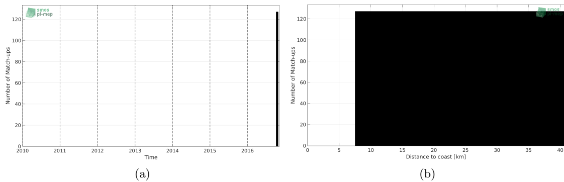
Figure 1: Number of match-ups between TSG-LEGOS-DM and SMAP-L3-JPL-V4-MONTHLY-60KM SSS as a function of time (a) and as function of the distance to coast (b) over the Gulf of Mexico Pi-MEP region and for the full satellite product period.
