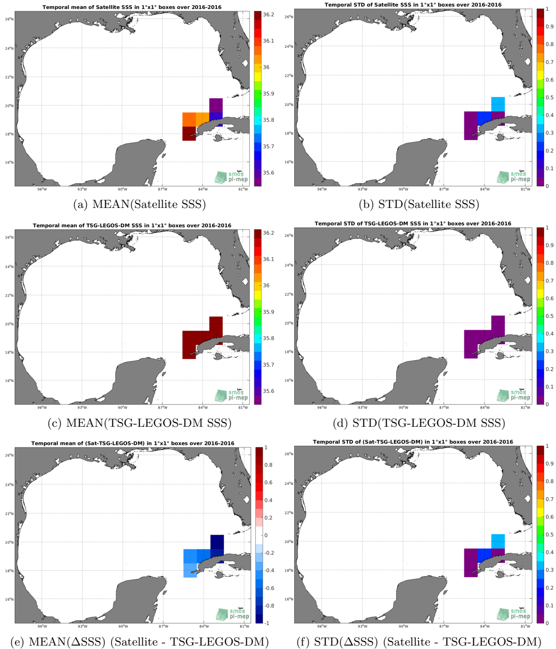
Figure 6: Temporal mean (left) and STD (right) of SSS from SMAP-L3-JPL-V4-MONTHLY-60KM (top), TSG-LEGOS-DM (middle), and of \Delta SSS (Satellite - TSG-LEGOS-DM). Only match-up pairs are used to generate these maps.
