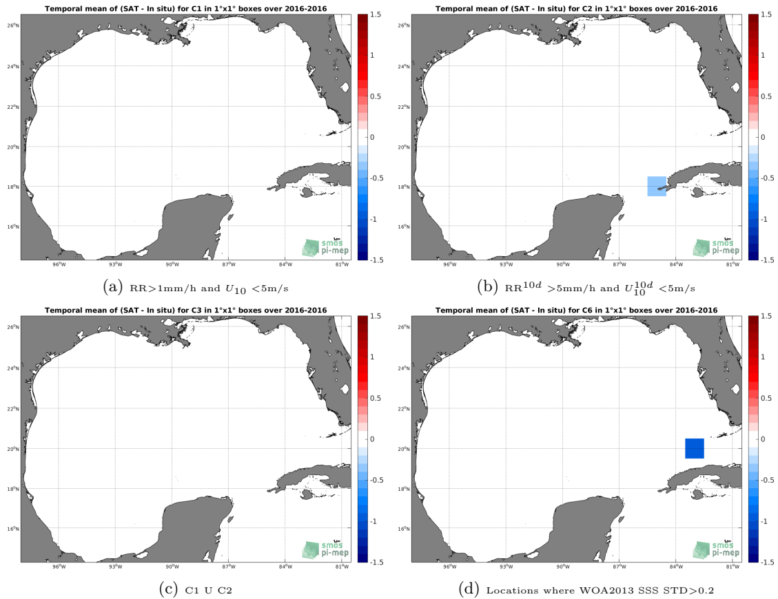
Figure 12: Temporal mean gridded over spatial boxes of size 1^\circ \times 1^\circ of \Delta SSS (SMAP-L3-JPL-V4-MONTHLY-60KM - TSG-LEGOS-DM) for 4 different subdatasets corresponding to: RR > 1\text{mm/h} and U_{10} < 5\text{m/s} (a), RR^{10d} > 5\text{mm/h} and U_{10}^{10d} < 5\text{m/s} (b), C1 U C2 (c), Locations where WOA2013 SSS STD > 0.2 (d).
