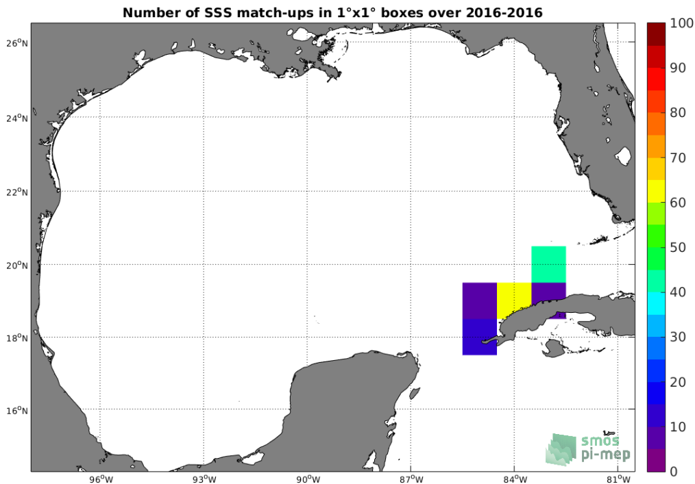
Figure 4: Number of SSS match-ups between TSG-LEGOS-DM SSS and the SMAP-L3-JPL-V4-MONTHLY-60KM SSS product for the Gulf of Mexico Pi-MEP region over 1^\circ \times 1^\circ boxes and for the full satellite product period.
