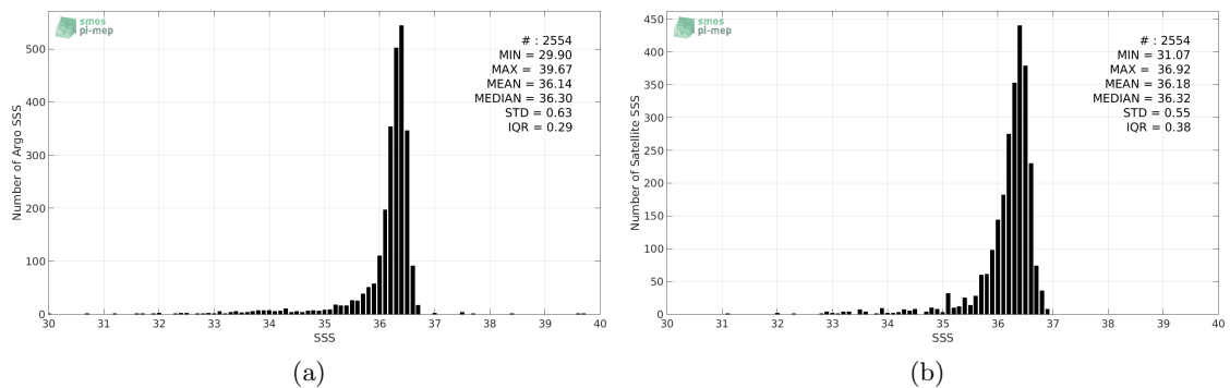
Figure 2: Histograms of SSS from Argo (a) and SMAP-L3-JPL-V4-MONTHLY-60KM (b) considering all match-up pairs per bins of 0.1 over the Gulf of Mexico Pi-MEP region and for the full satellite product period.
