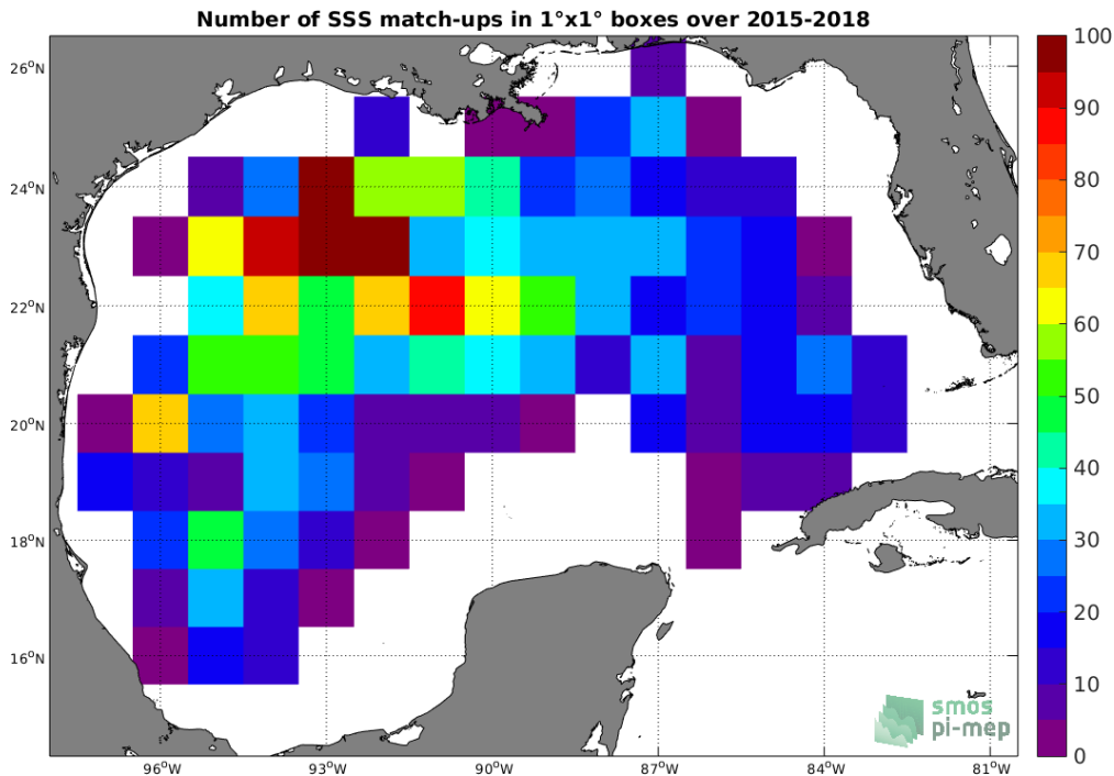
Figure 4: Number of SSS match-ups between Argo SSS and the SMAP-L3-JPL-V4-MONTHLY-60KM SSS product for the Gulf of Mexico Pi-MEP region over 1°x1° boxes and for the full satellite product period.
