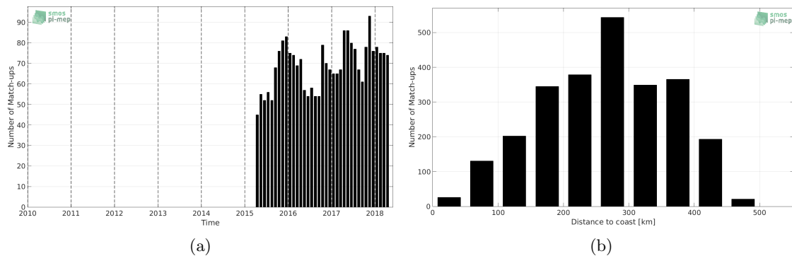
Figure 1: Number of match-ups between Argo and SMAP-L3-JPL-V4-MONTHLY-60KM SSS as a function of time (a) and as function of the distance to coast (b) over the Gulf of Mexico Pi-MEP region and for the full satellite product period.
