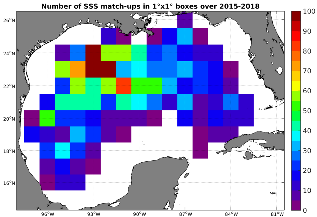
Figure 4: Number of SSS match-ups between Argo SSS and the SMAP-L3-JPL-V4-MONTHLY-60KM SSS product for the Gulf of Mexico Pi-MEP region over 1°x1° boxes and for the full satellite product period.
