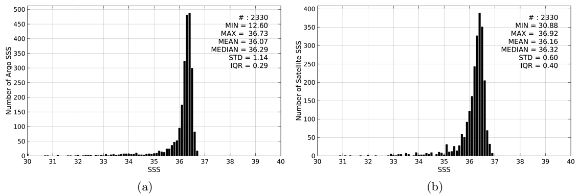
Figure 2: Histograms of SSS from Argo (a) and SMAP-L3-JPL-V4-MONTHLY-60KM (b) considering all match-up pairs per bins of 0.1 over the Gulf of Mexico Pi-MEP region and for the full satellite product period.
