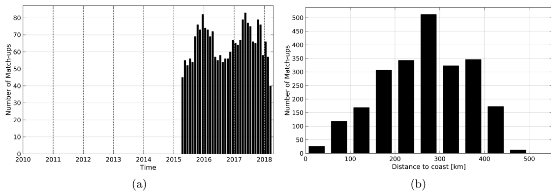
Figure 1: Number of match-ups between Argo and SMAP-L3-JPL-V4-MONTHLY-60KM SSS as a function of time (a) and as function of the distance to coast (b) over the Gulf of Mexico Pi-MEP region and for the full satellite product period.
