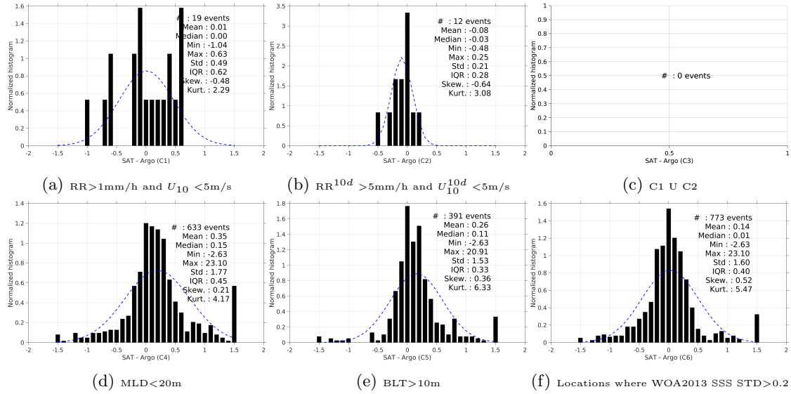
Figure 13: Normalized histogram of \Delta SSS (SMAP-L3-JPL-V4-MONTHLY-60KM - Argo) for 6 different subdatasets corresponding to: RR > 1mm/h and U_{10} < 5 m/s (a), RR 10d > 5mm/h and U_{10}^{10d} < 5 m/s (b), C1 U C2 (c), MLD < 20m (d), BLT > 10m (e), Locations where WOA2013 SSS STD > 0.2 (f).
