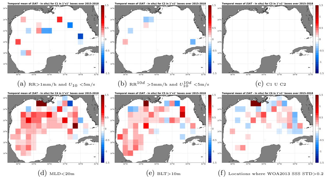
Figure 12: Temporal mean gridded over spatial boxes of size 1^\circ \times 1^\circ of \Delta SSS (SMAP-L3-JPL-V4-MONTHLY-60KM - Argo) for 6 different subdatasets corresponding to: RR > 1\text{mm/h} and U_{10} < 5\text{m/s} (a), RR^{10d} > 5\text{mm/h} and U_{10}^{10d} < 5\text{m/s} (b), C1 U C2 (c), MLD < 20\text{m} (d), BLT > 10\text{m} (e), Locations where WOA2013 SSS STD > 0.2 (f).
