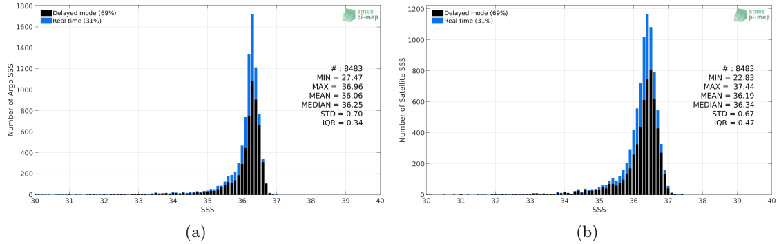
Figure 2: Histograms of SSS from Argo (a) and SMAP SSS L2-AVERAGED v5 (RSS) (b) considering all match-up pairs per bins of 0.1 over the Gulf of Mexico Pi-MEP region and for the full satellite product period.
