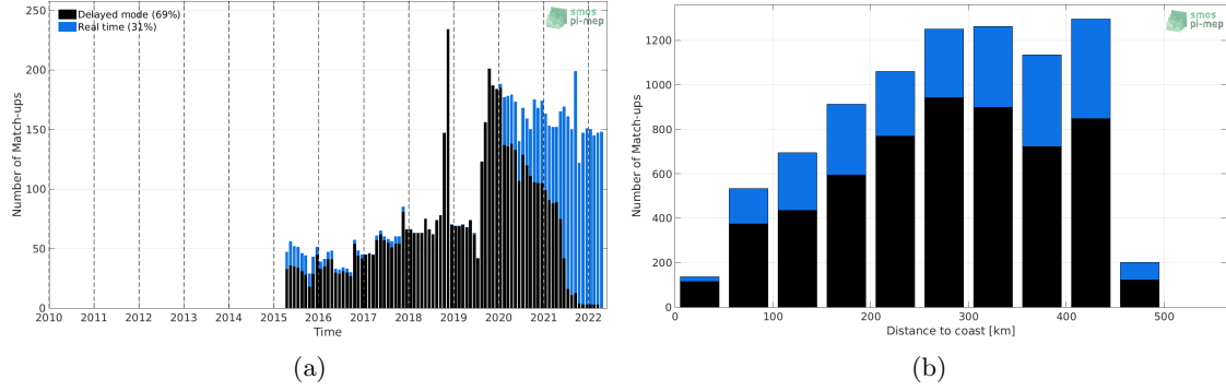
Figure 1: Number of match-ups between Argo and SMAP SSS L2-AVERAGED v5 (RSS) SSS as a function of time (a) and as function of the distance to coast (b) over the Gulf of Mexico Pi-MEP region and for the full satellite product period.
