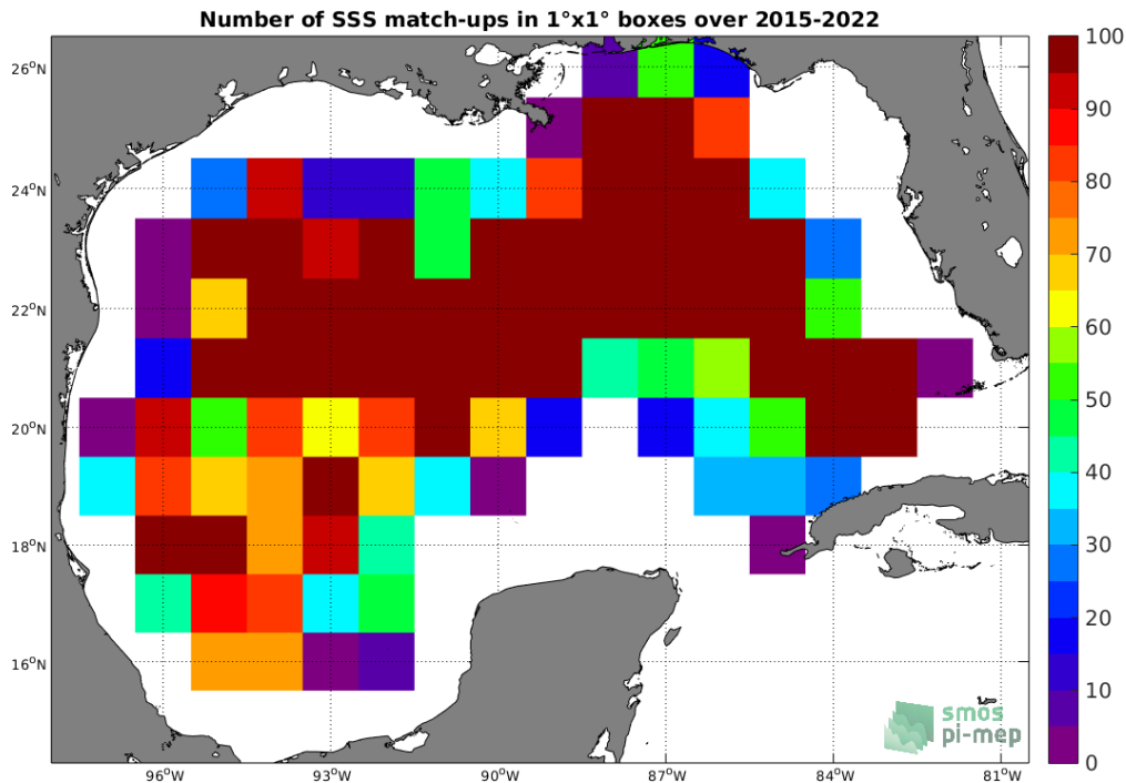
Figure 4: Number of SSS match-ups between Argo SSS and the SMAP SSS L2-AVERAGED v5 (RSS) SSS product for the Gulf of Mexico Pi-MEP region over 1°x1° boxes and for the full satellite product period.
