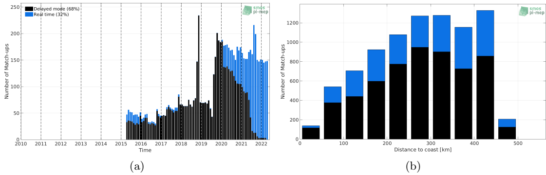
Figure 1: Number of match-ups between Argo and SMAP SSS L2-AVERAGED v5.0 (JPL) SSS as a function of time (a) and as function of the distance to coast (b) over the Gulf of Mexico Pi-MEP region and for the full satellite product period.
