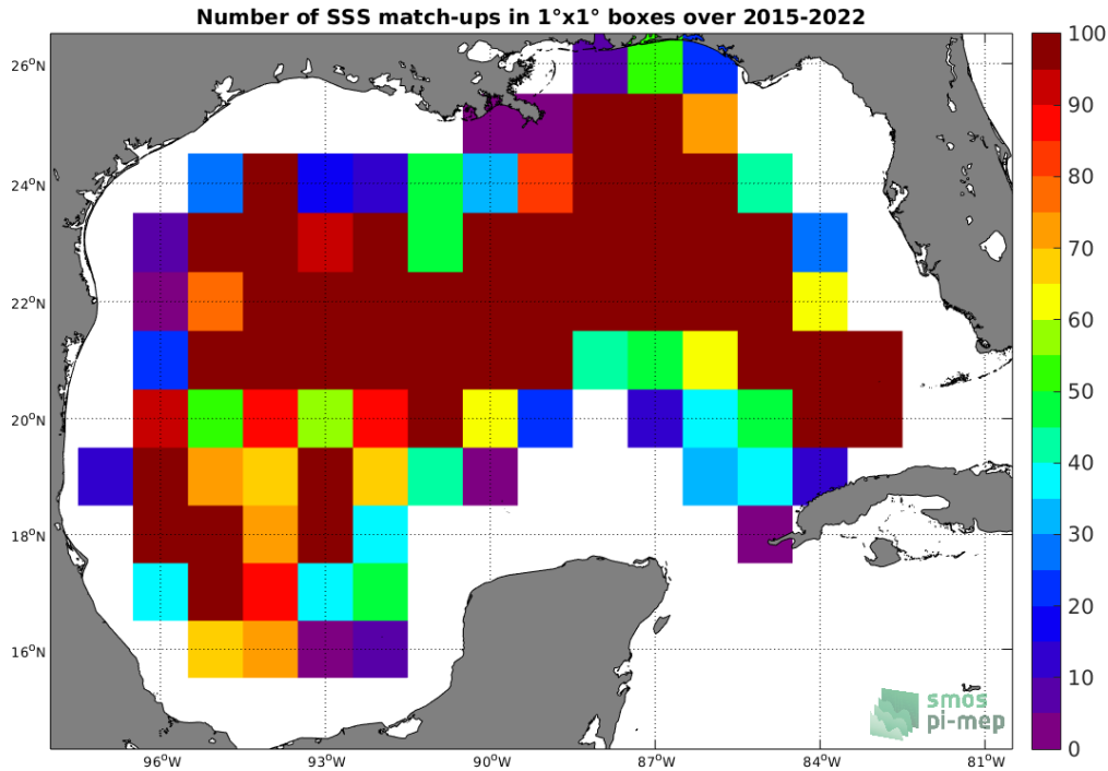
Figure 4: Number of SSS match-ups between Argo SSS and the SMAP SSS L2-AVERAGED v5.0 (JPL) SSS product for the Gulf of Mexico Pi-MEP region over 1^\circ \times 1^\circ boxes and for the full satellite product period.
