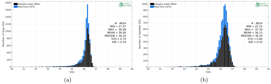
Figure 2: Histograms of SSS from Argo (a) and SMAP SSS L2-AVERAGED v5.0 (JPL) (b) considering all match-up pairs per bins of 0.1 over the Gulf of Mexico Pi-MEP region and for the full satellite product period.
