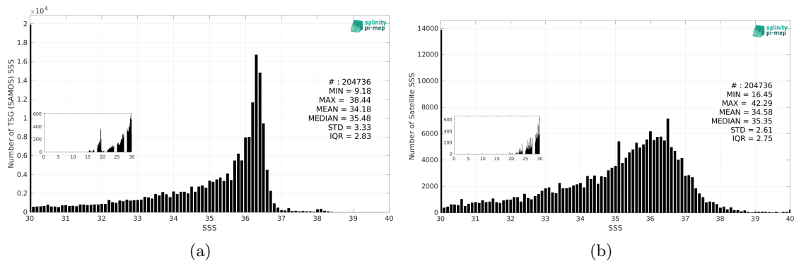
Figure 3: Histograms of SSS from TSG (SAMOS) (a) and SMAP SSS L2 v6 - 40 km (RSS) (b) considering all match-up pairs per bins of 0.1 over the Gulf of Mexico Pi-MEP region and for the full satellite product period.
