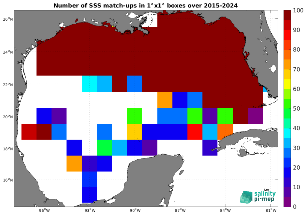
Figure 5: Number of SSS match-ups between TSG (SAMOS) SSS and the SMAP SSS L2 v6 - 40 km (RSS) SSS product for the Gulf of Mexico Pi-MEP region over 1^\circ \times 1^\circ boxes and for the full satellite product period.
