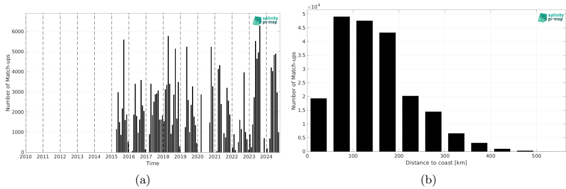
Figure 2: Number of match-ups between TSG (SAMOS) and SMAP SSS L2 v6 - 40 km (RSS) SSS as a function of time (a) and as function of the distance to coast (b) over the Gulf of Mexico Pi-MEP region and for the full satellite product period.
