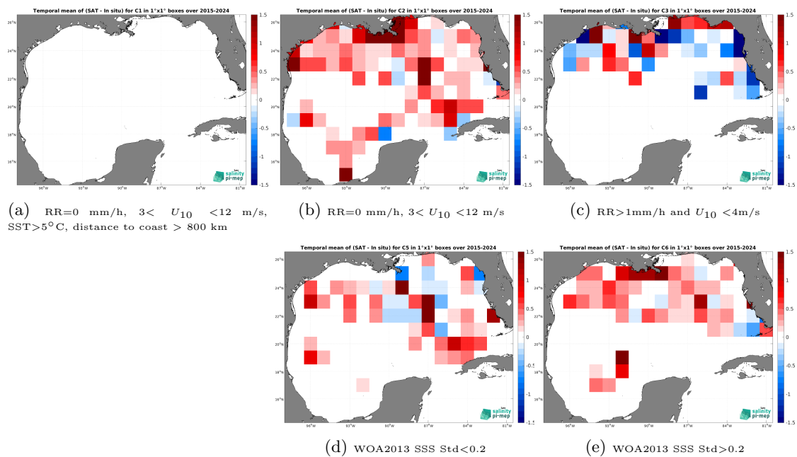
Figure 14: Temporal mean gridded over spatial boxes of size 1^\circ \times 1^\circ of \Delta SSS (SMAP SSS L2 v6 - 40 km (RSS) - TSG (SAMOS)) for 5 different subdatasets corresponding to:RR=0 mm/h, 3 < U_{10} < 12 m/s, SST >5^\circ C, distance to coast > 800 km (a), RR=0 mm/h, 3 < U_{10} < 12 m/s (b), RR >1 mm/h and U_{10} < 4 m/s (c), WOA2013 SSS Std <0.2 (d), WOA2013 SSS Std >0.2 (e).
