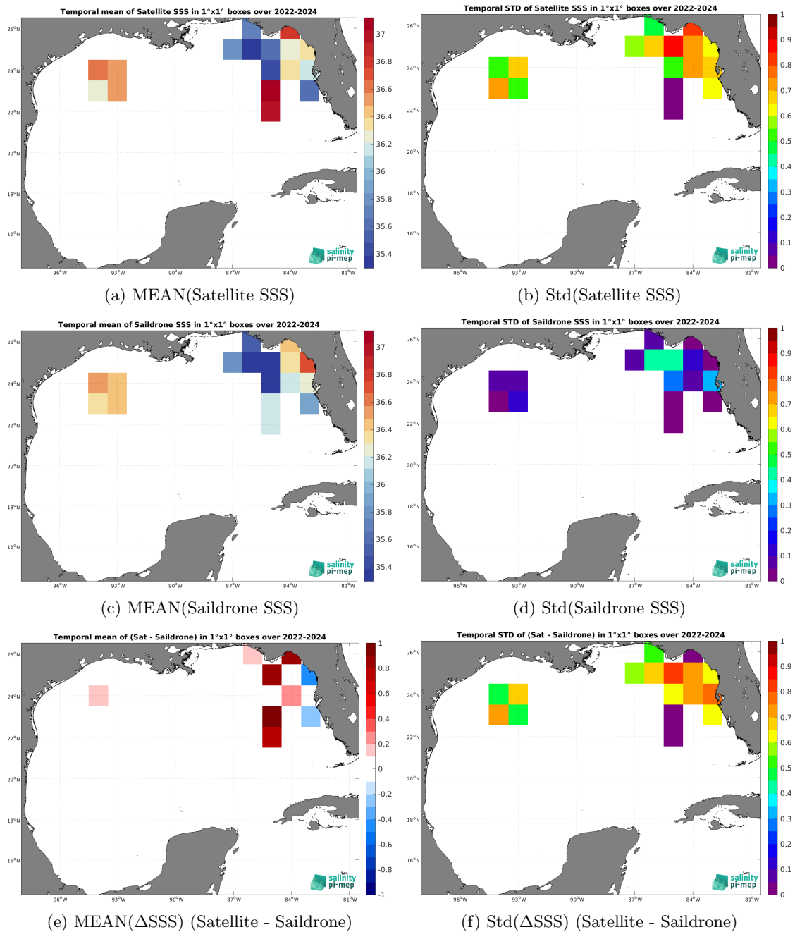
Figure 7: Temporal mean (left) and Std (right) of SSS from SMAP SSS L2 v6 - 40 km (RSS) (top), Saildrone (middle), and of \Delta SSS (Satellite - Saildrone). Only match-up pairs are used to generate these maps.
