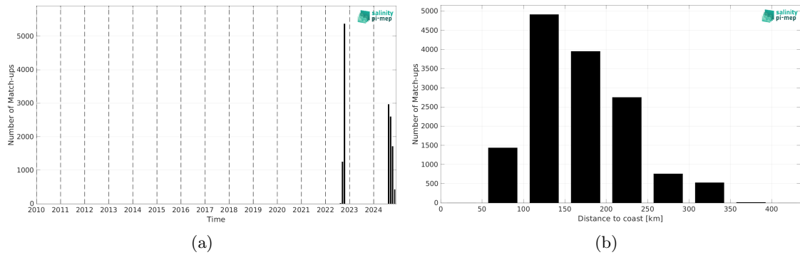
Figure 2: Number of match-ups between Saildrone and SMAP SSS L2 v6 - 40 km (RSS) SSS as a function of time (a) and as function of the distance to coast (b) over the Gulf of Mexico Pi-MEP region and for the full satellite product period.
