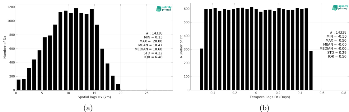
Figure 6: Histograms of the spatial (a) and temporal (b) lags between the location/time of the Saildrone measurement and the date of the corresponding SMAP SSS L2 v6 - 40 km (RSS) SSS pixel.
