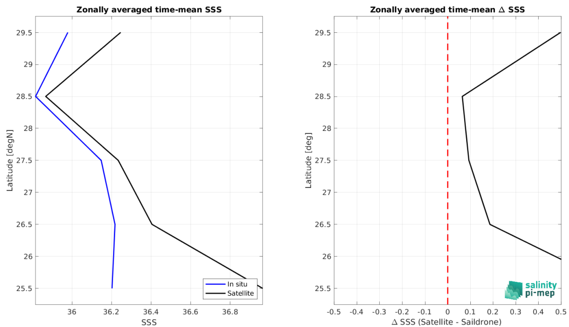
Figure 9: Left panel: Zonal mean SSS from SMAP SSS L2 v6 - 40 km (RSS) satellite product (black) and from Sairdrone (blue). Right panel: Zonal mean of \Delta SSS (Satellite - Sairdrone) for all the collected Pi-MEP match-up pairs estimated over the full satellite product period.
