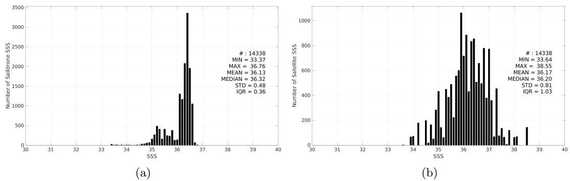
Figure 3: Histograms of SSS from Saildrone (a) and SMAP SSS L2 v6 - 40 km (RSS) (b) considering all match-up pairs per bins of 0.1 over the Gulf of Mexico Pi-MEP region and for the full satellite product period.
