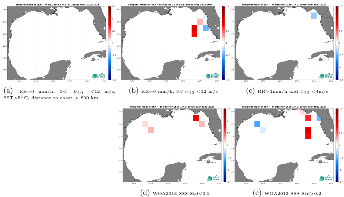
Figure 14: Temporal mean gridded over spatial boxes of size 1^\circ \times 1^\circ of \Delta SSS (SMAP SSS L2 v6 - 40 km (RSS) - Sairdrone) for 5 different subdatasets corresponding to:RR=0 mm/h, 3 < U_{10} < 12 m/s, SST >5^\circ C, distance to coast > 800 km (a), RR=0 mm/h, 3 < U_{10} < 12 m/s (b), RR >1 mm/h and U_{10} < 4 m/s (c), WOA2013 SSS Std <0.2 (d), WOA2013 SSS Std >0.2 (e).
