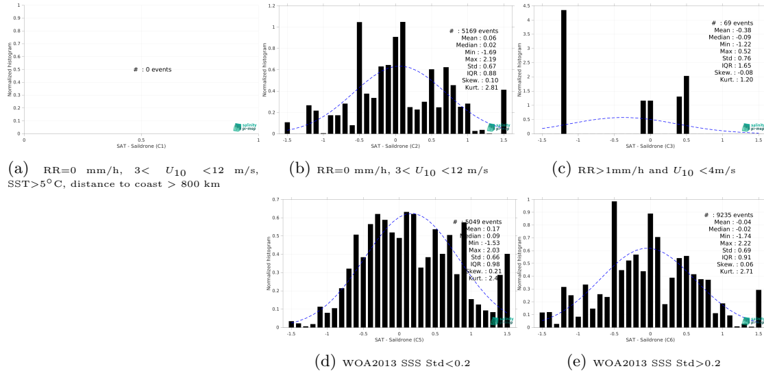
Figure 15: Normalized histogram of \Delta SSS (SMAP SSS L2 v6 - 40 km (RSS) - Saildrone) for 5 different subdatasets corresponding to: RR=0 mm/h, 3 < U_{10} < 12 m/s, SST > 5°C, distance to coast > 800 km (a), RR=0 mm/h, 3 < U_{10} < 12 m/s (b), RR > 1mm/h and U_{10} < 4 m/s (c), WOA2013 SSS Std < 0.2 (d), WOA2013 SSS Std > 0.2 (e).
