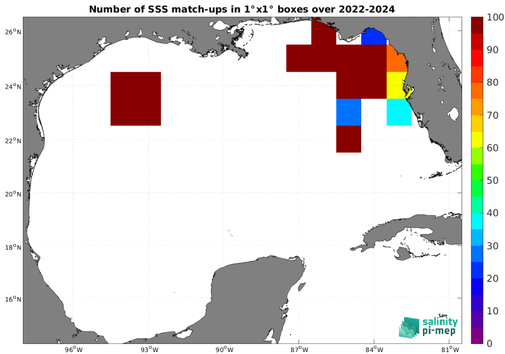
Figure 5: Number of SSS match-ups between Saildrone SSS and the SMAP SSS L2 v6 - 40 km (RSS) SSS product for the Gulf of Mexico Pi-MEP region over 1^\circ \times 1^\circ boxes and for the full satellite product period.
