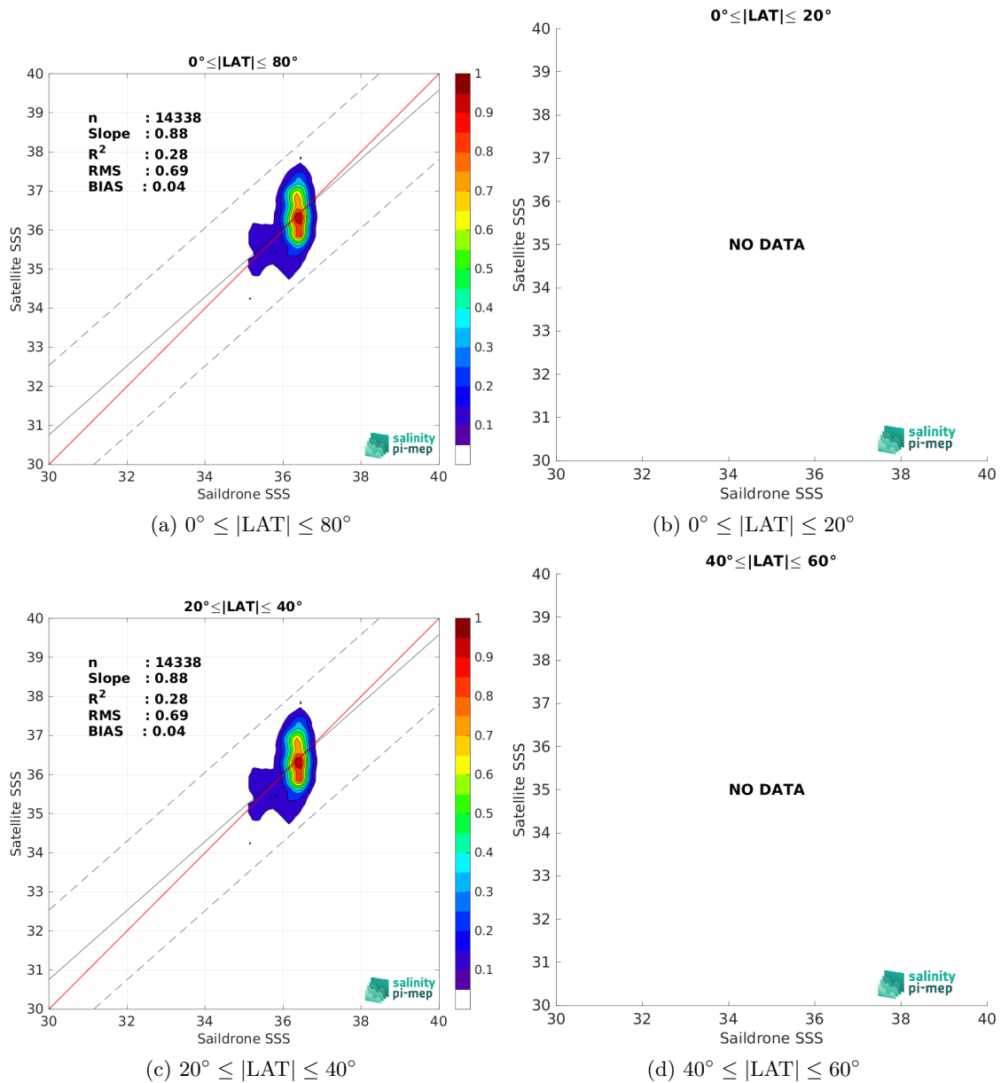
Figure 10: Contour maps of the concentration of SMAP SSS L2 v6 - 40 km (RSS) SSS (y-axis) versus Saildrone SSS (x-axis) at match-up pairs for different latitude bands. For each plot, the red line shows x=y . The black thin and dashed lines indicate a linear fit through the data cloud and the \pm 95\% confidence levels, respectively. The number match-up pairs n , the slope and R^2 coefficient of the linear fit, the root mean square (RMS) and the mean bias between satellite and in situ data are indicated for each latitude band in each plots.
