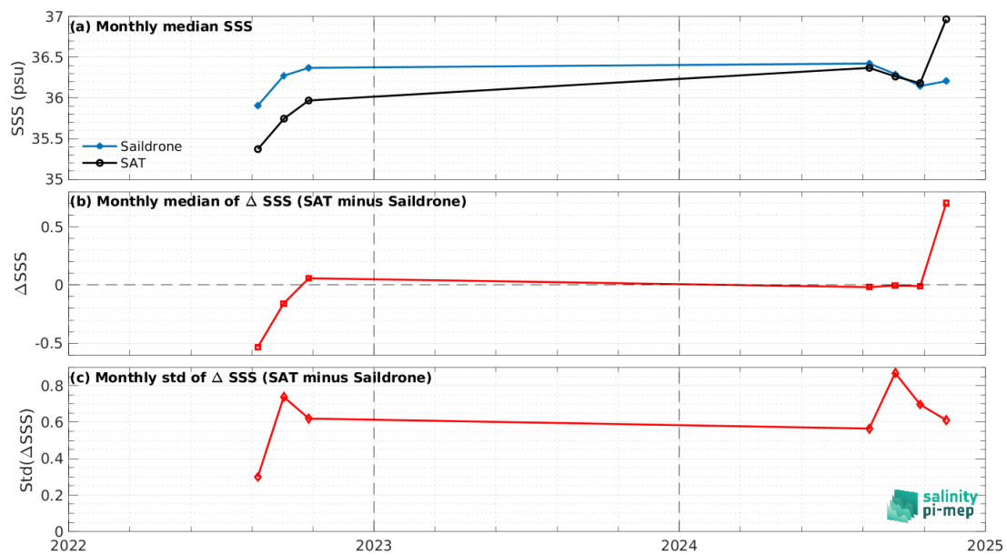
Figure 8: Time series of the monthly median SSS (top), median of \Delta SSS (Satellite - Sairdrone) and Std of \Delta SSS (Satellite - Sairdrone) over the Gulf of Mexico Pi-MEP region considering all match-ups collected by the Pi-MEP.
