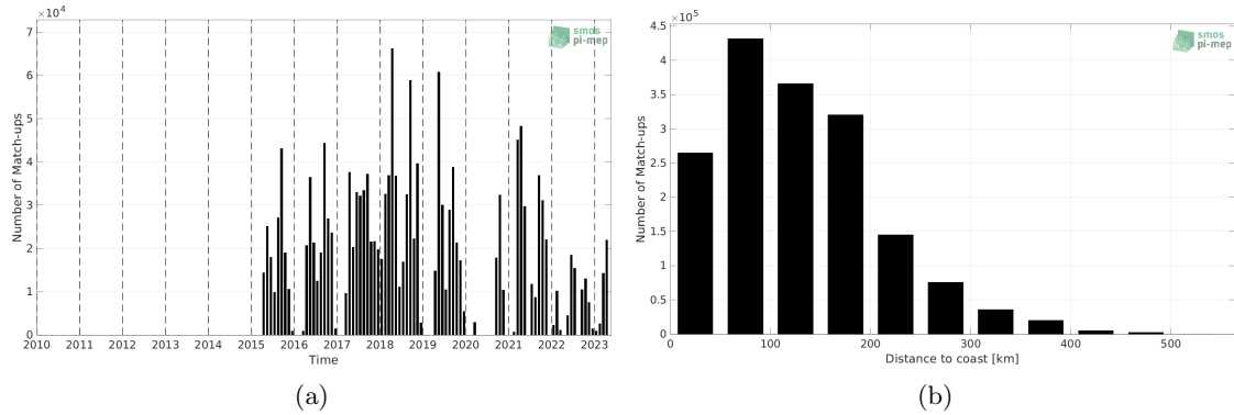
Figure 1: Number of match-ups between TSG (SAMOS) and SMAP SSS L2 v5 (RSS) SSS as a function of time (a) and as function of the distance to coast (b) over the Gulf of Mexico Pi-MEP region and for the full satellite product period.
