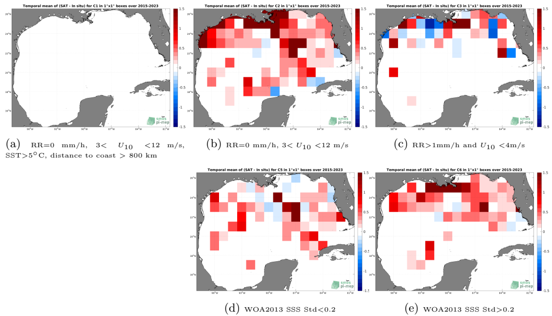
Figure 12: Temporal mean gridded over spatial boxes of size 1^\circ \times 1^\circ of \Delta SSS (SMAP SSS L2 v5 (RSS) - TSG (SAMOS)) for 5 different subdatasets corresponding to:RR=0 mm/h, 3 < U_{10} < 12 m/s, SST >5^\circ C, distance to coast > 800 km (a), RR=0 mm/h, 3 < U_{10} < 12 m/s (b), RR >1 mm/h and U_{10} < 4 m/s (c), WOA2013 SSS Std <0.2 (d), WOA2013 SSS Std >0.2 (e).
