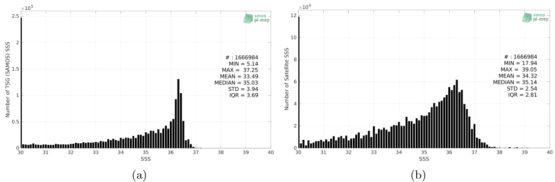
Figure 2: Histograms of SSS from TSG (SAMOS) (a) and SMAP SSS L2 v5 (RSS) (b) considering all match-up pairs per bins of 0.1 over the Gulf of Mexico Pi-MEP region and for the full satellite product period.
