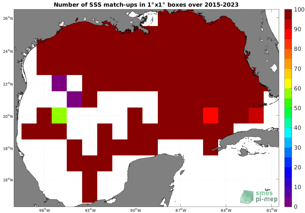
Figure 4: Number of SSS match-ups between TSG (SAMOS) SSS and the SMAP SSS L2 v5 (RSS) SSS product for the Gulf of Mexico Pi-MEP region over 1^\circ \times 1^\circ boxes and for the full satellite product period.
