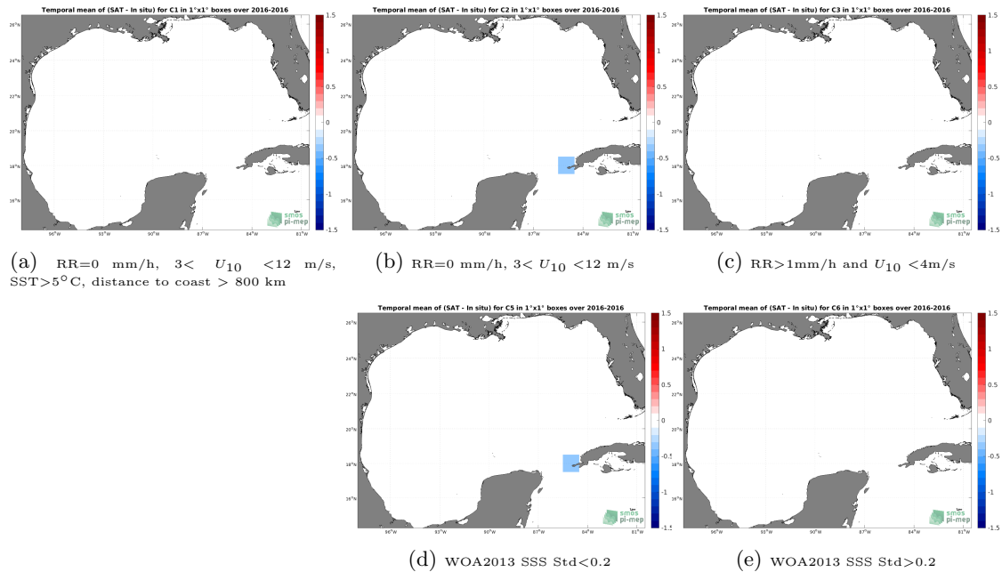
Figure 12: Temporal mean gridded over spatial boxes of size 1^{\circ}\times 1^{\circ} of \Delta\text{SSS} (SMAP SSS L2 v5 (RSS) - TSG (LEGOS-DM)) for 5 different subdatasets corresponding to:RR=0 mm/h, 3 < U_{10} < 12 m/s, SST >5^{\circ}\text{C} , distance to coast > 800 km (a), RR=0 mm/h, 3 < U_{10} < 12 m/s (b), RR >1 mm/h and U_{10} < 4 m/s (c), WOA2013 SSS Std <0.2 (d), WOA2013 SSS Std >0.2 (e).
