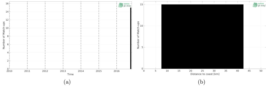
Figure 1: Number of match-ups between TSG (LEGOS-DM) and SMAP SSS L2 v5 (RSS) SSS as a function of time (a) and as function of the distance to coast (b) over the Gulf of Mexico Pi-MEP region and for the full satellite product period.
