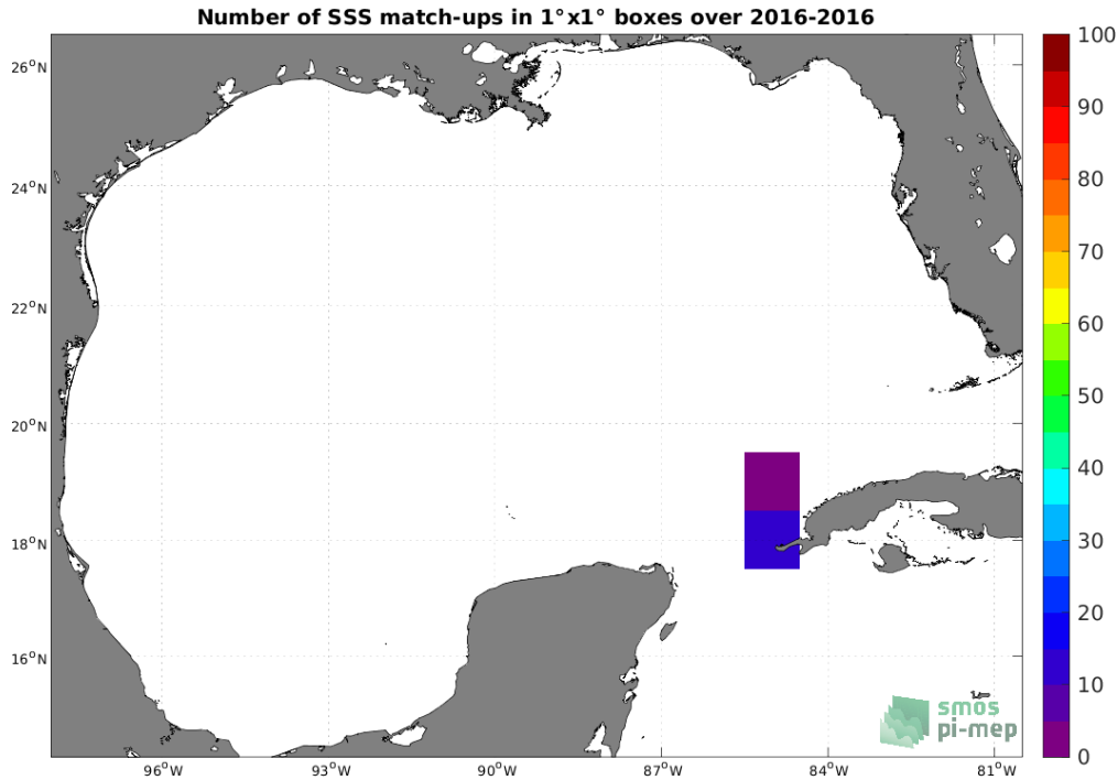
Figure 4: Number of SSS match-ups between TSG (LEGOS-DM) SSS and the SMAP SSS L2 v5 (RSS) SSS product for the Gulf of Mexico Pi-MEP region over 1^\circ \times 1^\circ boxes and for the full satellite product period.
