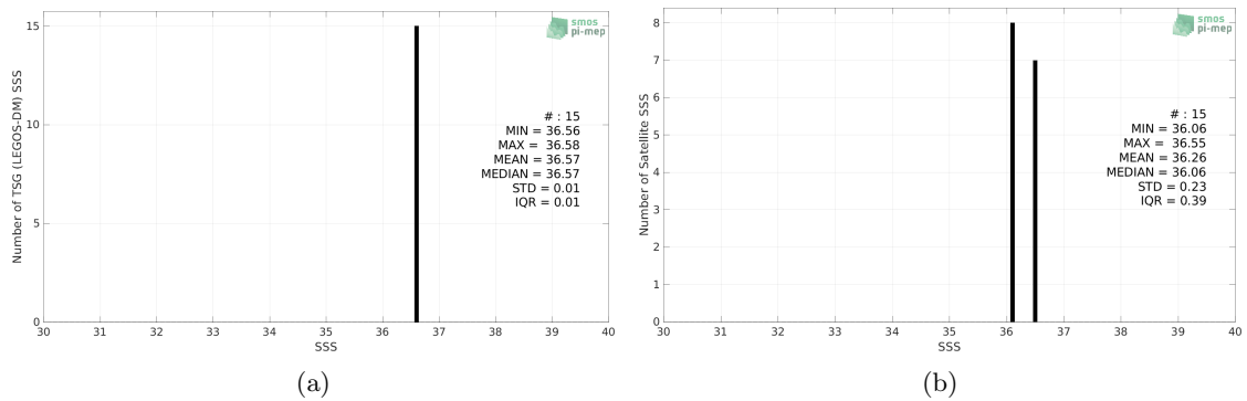
Figure 2: Histograms of SSS from TSG (LEGOS-DM) (a) and SMAP SSS L2 v5 (RSS) (b) considering all match-up pairs per bins of 0.1 over the Gulf of Mexico Pi-MEP region and for the full satellite product period.
