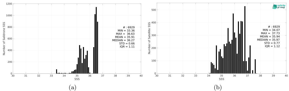
Figure 2: Histograms of SSS from Saildrone (a) and SMAP SSS L2 v5 (RSS) (b) considering all match-up pairs per bins of 0.1 over the Gulf of Mexico Pi-MEP region and for the full satellite product period.
