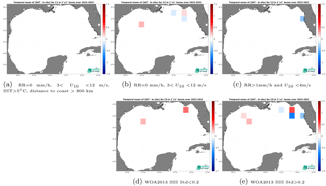
Figure 12: Temporal mean gridded over spatial boxes of size 1^{\circ}\times 1^{\circ} of \Delta\text{SSS} (SMAP SSS L2 v5 (RSS) - Saldrone) for 5 different subdatasets corresponding to:RR=0 mm/h, 3 < U_{10} < 12 m/s, SST >5^{\circ}\text{C} , distance to coast > 800 km (a), RR=0 mm/h, 3 < U_{10} < 12 m/s (b), RR >1 mm/h and U_{10} < 4 m/s (c), WOA2013 SSS Std <0.2 (d), WOA2013 SSS Std >0.2 (e).
