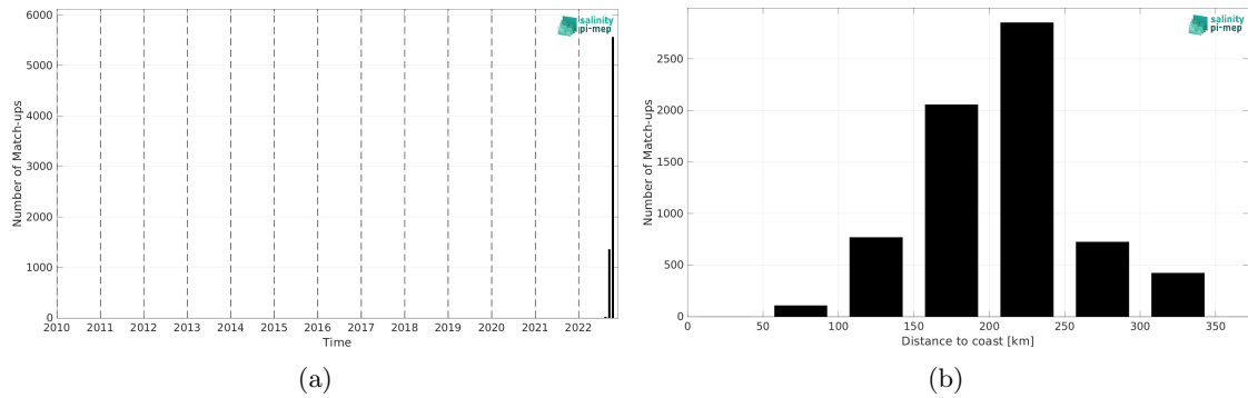
Figure 1: Number of match-ups between Saildrone and SMAP SSS L2 v5 (RSS) SSS as a function of time (a) and as function of the distance to coast (b) over the Gulf of Mexico Pi-MEP region and for the full satellite product period.
