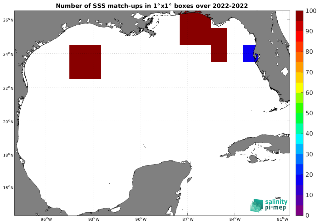
Figure 4: Number of SSS match-ups between Saildrone SSS and the SMAP SSS L2 v5 (RSS) SSS product for the Gulf of Mexico Pi-MEP region over 1°×1° boxes and for the full satellite product period.
