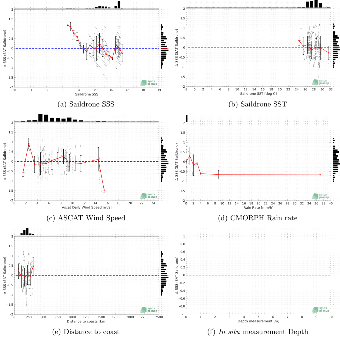
Figure 11: \Delta SSS (Satellite - Saildrone) sorted as function of SSS values a), SSS SST b), ASCAT Wind speed c), CMORPH rain rate d), distance to coast (e) and in situ measurement depth (f). In all plots the median and Std of \Delta SSS for each bin is indicated by the red curves and black vertical thick bars ( \pm 1 Std)
