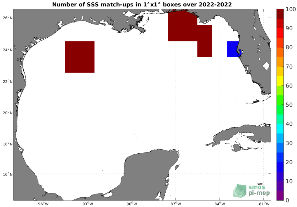
Figure 4: Number of SSS match-ups between Saildrone SSS and the SMAP SSS L2 v5 (RSS) SSS product for the Gulf of Mexico Pi-MEP region over 1^\circ \times 1^\circ boxes and for the full satellite product period.
