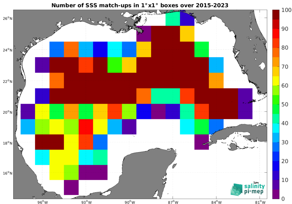
Figure 4: Number of SSS match-ups between Argo SSS and the SMAP SSS L2 v5 (RSS) SSS product for the Gulf of Mexico Pi-MEP region over 1^\circ \times 1^\circ boxes and for the full satellite product period.
