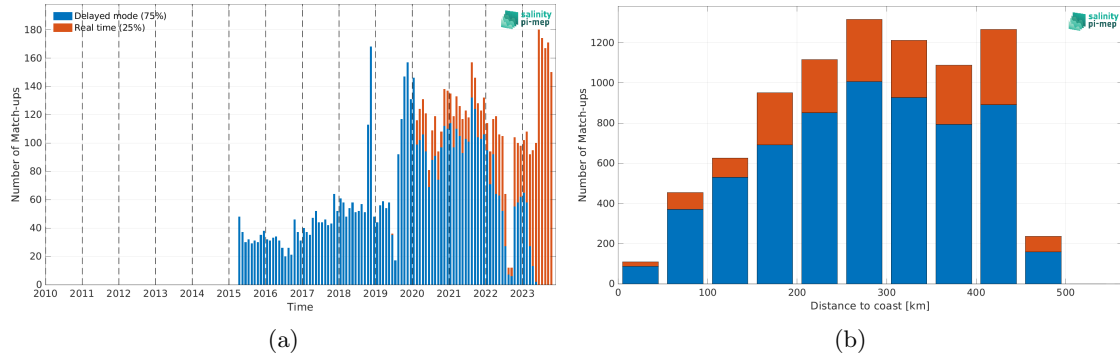
Figure 1: Number of match-ups between Argo and SMAP SSS L2 v5 (RSS) SSS as a function of time (a) and as function of the distance to coast (b) over the Gulf of Mexico Pi-MEP region and for the full satellite product period.
