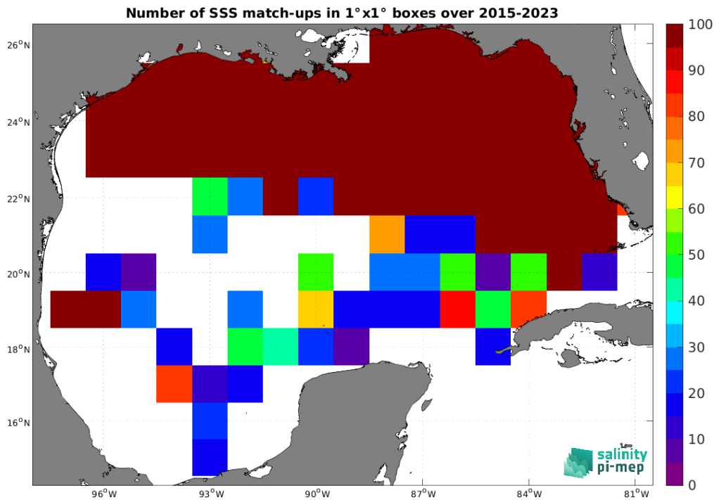
Figure 5: Number of SSS match-ups between TSG (SAMOS) SSS and the SMAP SSS L2 v5.3 (RSS) SSS product for the Gulf of Mexico Pi-MEP region over 1°×1° boxes and for the full satellite product period.
