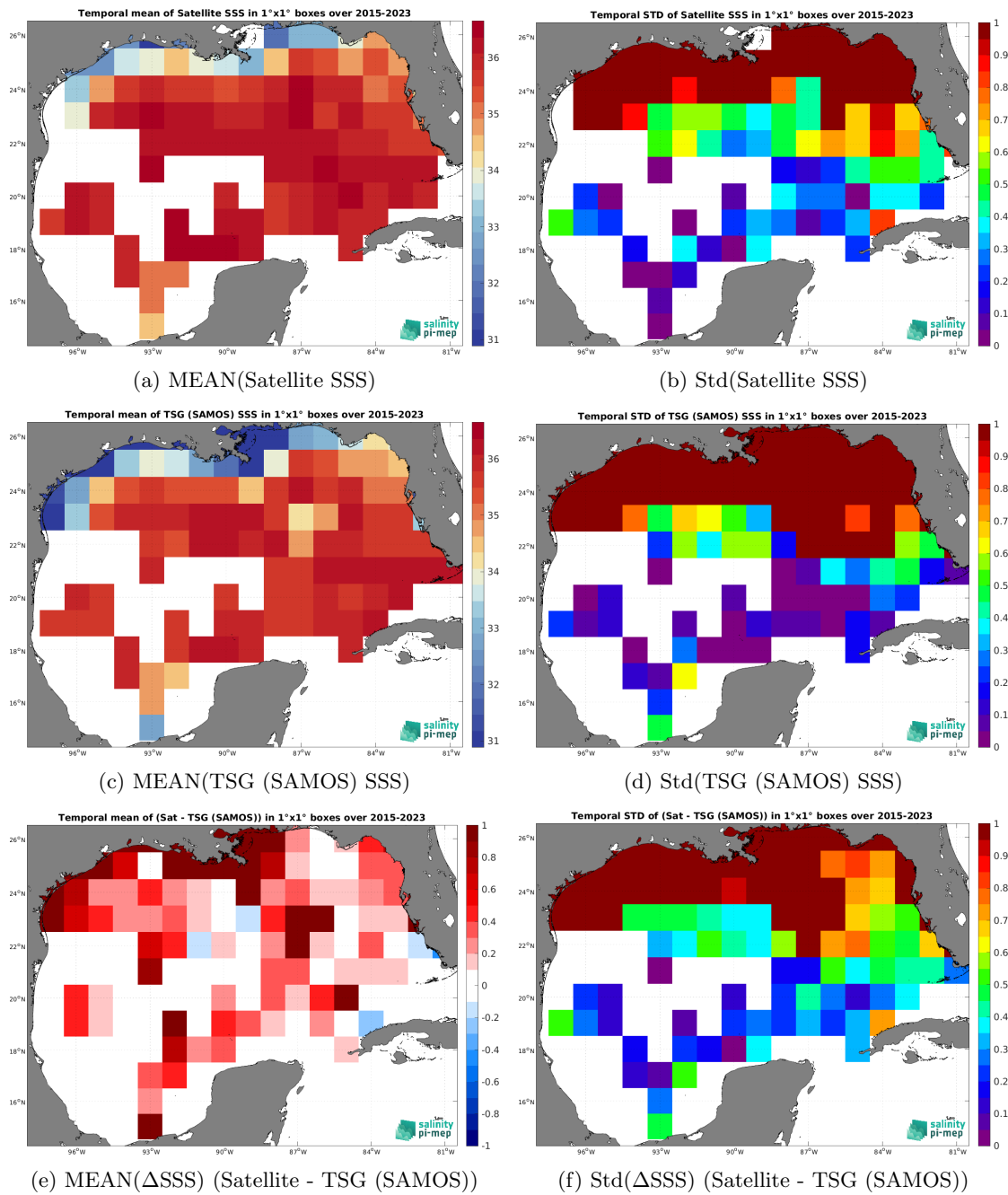
Figure 7: Temporal mean (left) and Std (right) of SSS from SMAP SSS L2 v5.3 (RSS) (top), TSG (SAMOS) (middle), and of \Delta SSS (Satellite - TSG (SAMOS)). Only match-up pairs are used to generate these maps.
