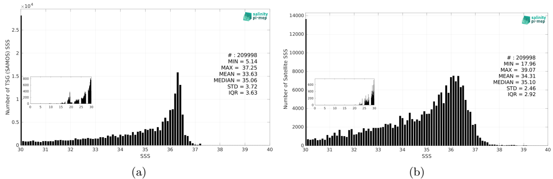
Figure 3: Histograms of SSS from TSG (SAMOS) (a) and SMAP SSS L2 v5.3 (RSS) (b) considering all match-up pairs per bins of 0.1 over the Gulf of Mexico Pi-MEP region and for the full satellite product period.
