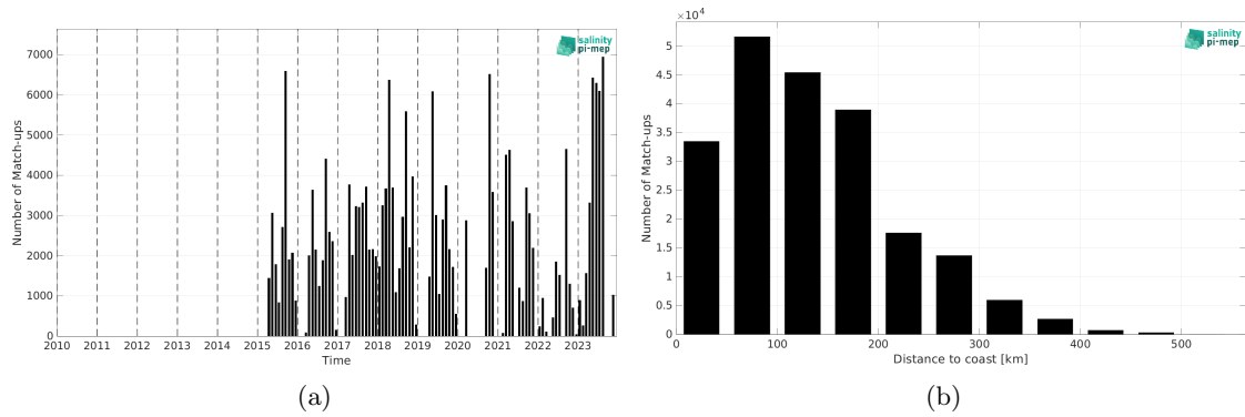
Figure 2: Number of match-ups between TSG (SAMOS) and SMAP SSS L2 v5.3 (RSS) SSS as a function of time (a) and as function of the distance to coast (b) over the Gulf of Mexico Pi-MEP region and for the full satellite product period.
