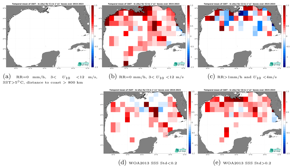
Figure 14: Temporal mean gridded over spatial boxes of size 1^\circ \times 1^\circ of \Delta SSS (SMAP SSS L2 v5.3 (RSS) - TSG (SAMOS)) for 5 different subdatasets corresponding to:RR=0 mm/h, 3 < U_{10} < 12 m/s, SST>5°C, distance to coast > 800 km (a), RR=0 mm/h, 3 < U_{10} < 12 m/s (b), RR>1mm/h and U_{10} < 4 m/s (c), WOA2013 SSS Std<0.2 (d), WOA2013 SSS Std>0.2 (e).
