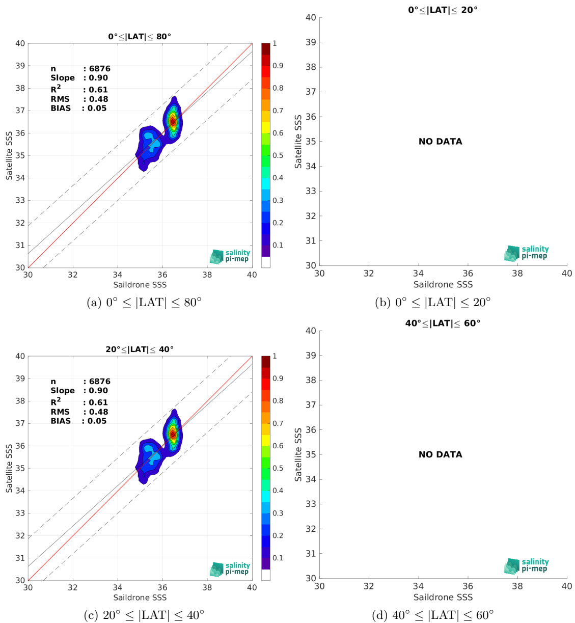
Figure 10: Contour maps of the concentration of SMAP SSS L2 v5.3 (RSS) SSS (y-axis) versus Saildrone SSS (x-axis) at match-up pairs for different latitude bands. For each plot, the red line shows x=y . The black thin and dashed lines indicate a linear fit through the data cloud and the \pm 95\% confidence levels, respectively. The number match-up pairs n , the slope and R^2 coefficient of the linear fit, the root mean square (RMS) and the mean bias between satellite and in situ data are indicated for each latitude band in each plots.
