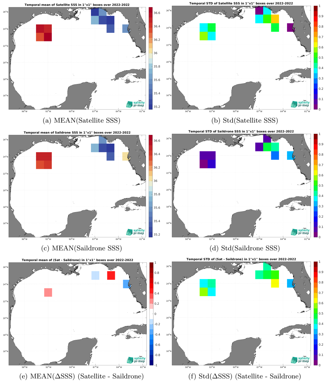
Figure 7: Temporal mean (left) and Std (right) of SSS from SMAP SSS L2 v5.3 (RSS) (top), Saildrone (middle), and of \Delta SSS (Satellite - Saildrone). Only match-up pairs are used to generate these maps.
