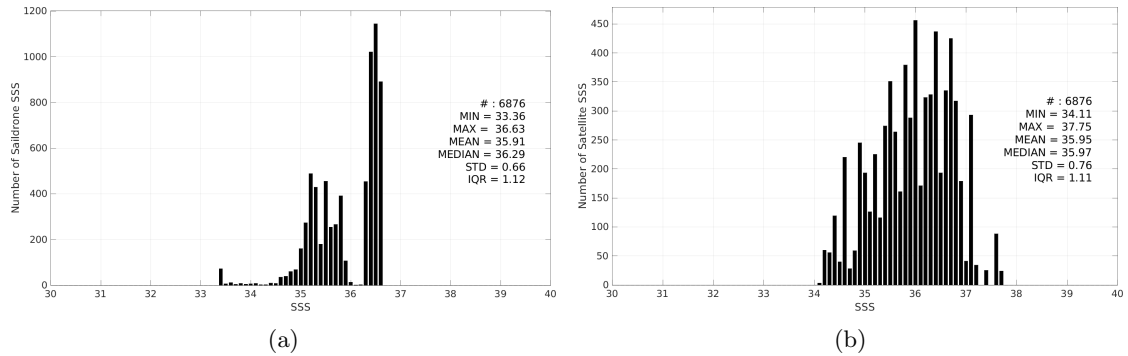
Figure 3: Histograms of SSS from Saildrone (a) and SMAP SSS L2 v5.3 (RSS) (b) considering all match-up pairs per bins of 0.1 over the Gulf of Mexico Pi-MEP region and for the full satellite product period.
