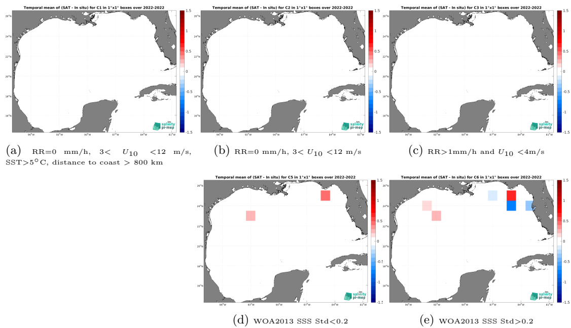
Figure 14: Temporal mean gridded over spatial boxes of size 1^\circ \times 1^\circ of \Delta\text{SSS} (SMAP SSS L2 v5.3 (RSS) - Saildrone) for 5 different subdatasets corresponding to:RR=0 mm/h, 3 < U_{10} < 12 m/s, SST >5^\circ\text{C} , distance to coast > 800 km (a), RR=0 mm/h, 3 < U_{10} < 12 m/s (b), RR >1 mm/h and U_{10} < 4 m/s (c), WOA2013 SSS Std <0.2 (d), WOA2013 SSS Std >0.2 (e).
