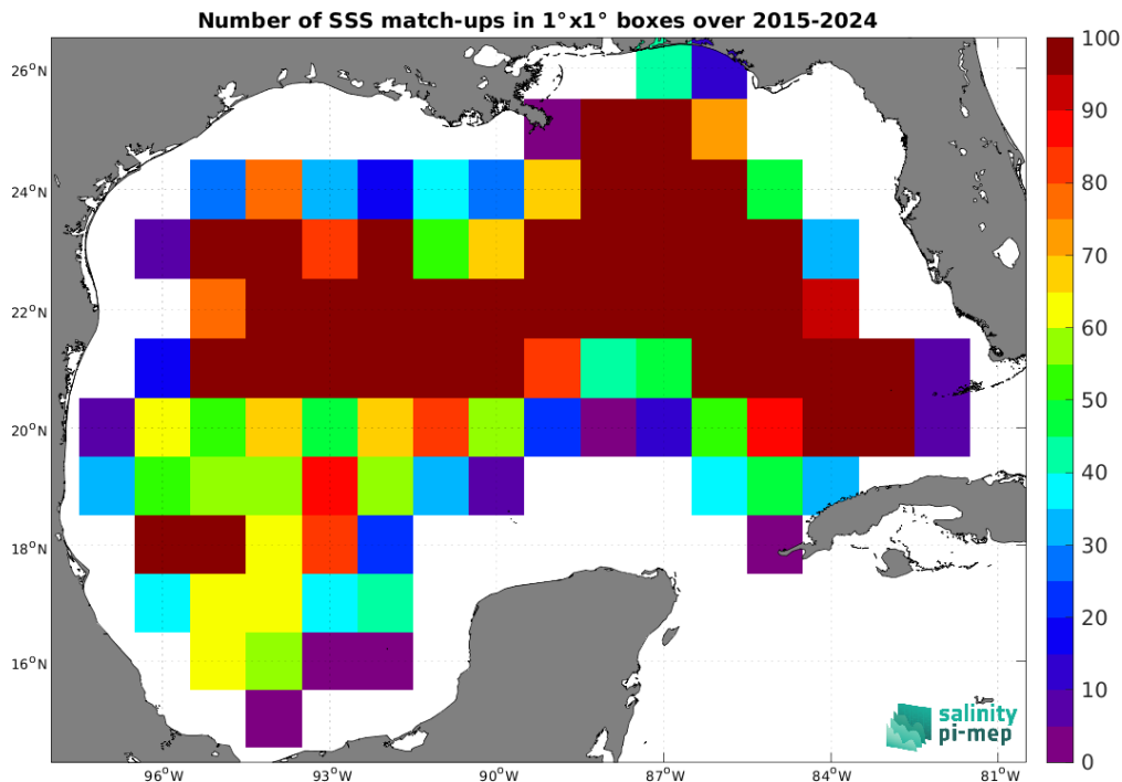
Figure 5: Number of SSS match-ups between Argo SSS and the SMAP SSS L2 v5.3 (RSS) SSS product for the Gulf of Mexico Pi-MEP region over 1^\circ \times 1^\circ boxes and for the full satellite product period.
