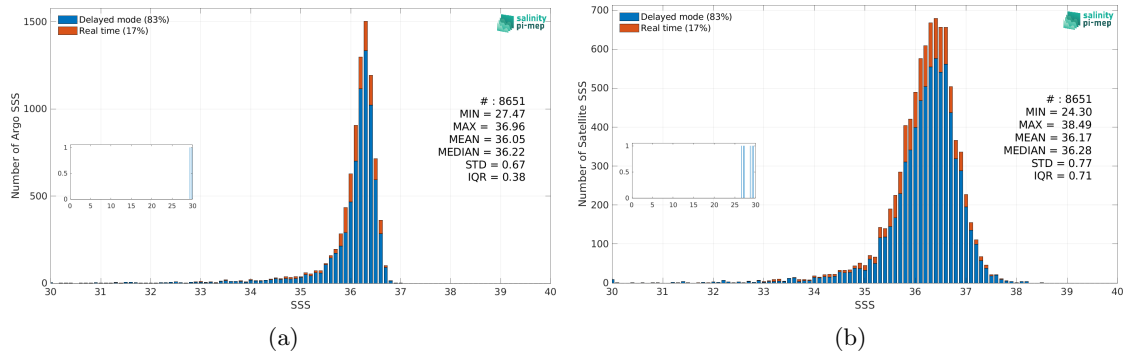
Figure 3: Histograms of SSS from Argo (a) and SMAP SSS L2 v5.3 (RSS) (b) considering all match-up pairs per bins of 0.1 over the Gulf of Mexico Pi-MEP region and for the full satellite product period.
