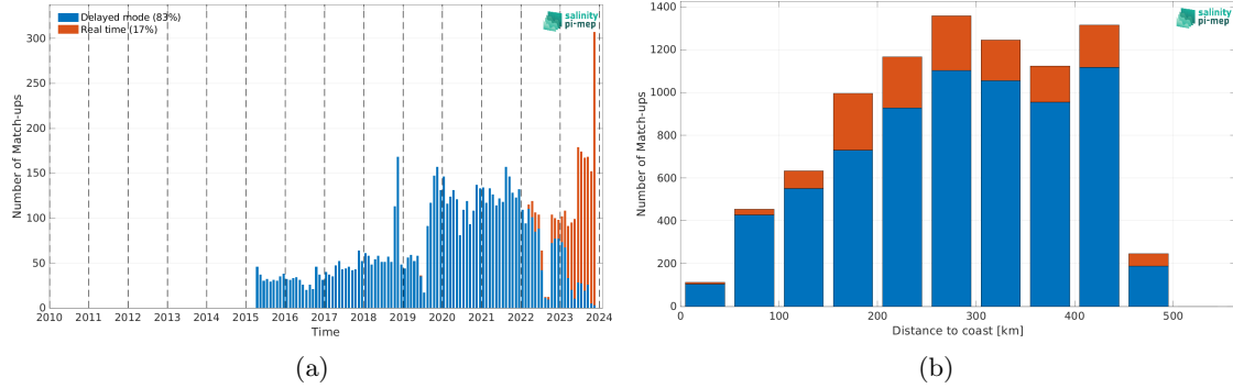
Figure 2: Number of match-ups between Argo and SMAP SSS L2 v5.3 (RSS) SSS as a function of time (a) and as function of the distance to coast (b) over the Gulf of Mexico Pi-MEP region and for the full satellite product period.
