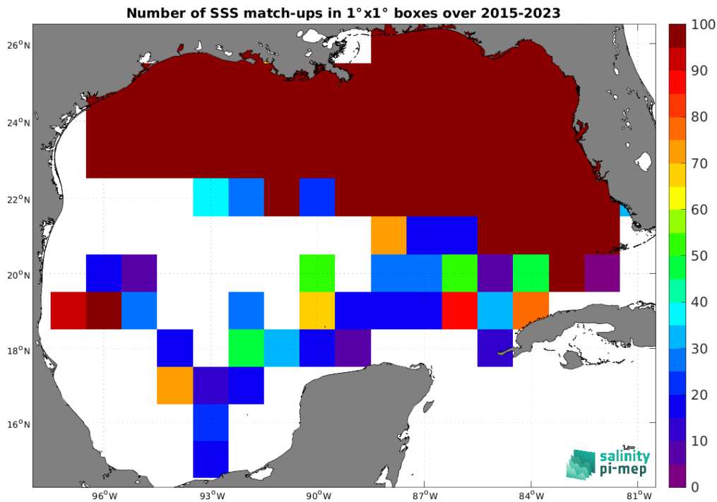
Figure 5: Number of SSS match-ups between TSG (SAMOS) SSS and the SMAP SSS L2 v5.3 - 40 km (RSS) SSS product for the Gulf of Mexico Pi-MEP region over 1^\circ \times 1^\circ boxes and for the full satellite product period.
