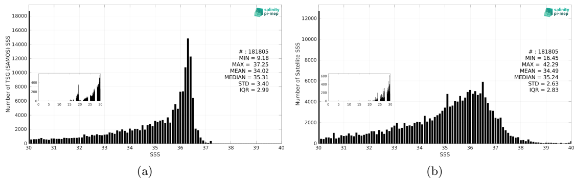
Figure 3: Histograms of SSS from TSG (SAMOS) (a) and SMAP SSS L2 v5.3 - 40 km (RSS) (b) considering all match-up pairs per bins of 0.1 over the Gulf of Mexico Pi-MEP region and for the full satellite product period.
