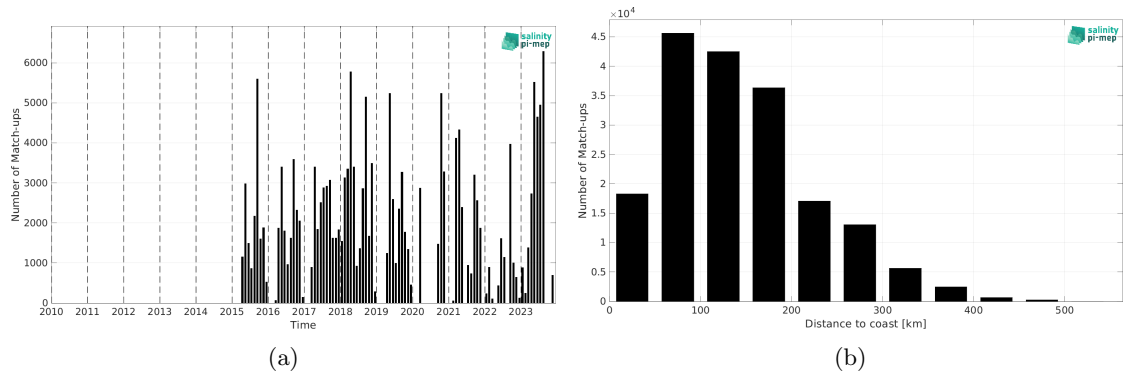
Figure 2: Number of match-ups between TSG (SAMOS) and SMAP SSS L2 v5.3 - 40 km (RSS) SSS as a function of time (a) and as function of the distance to coast (b) over the Gulf of Mexico Pi-MEP region and for the full satellite product period.
