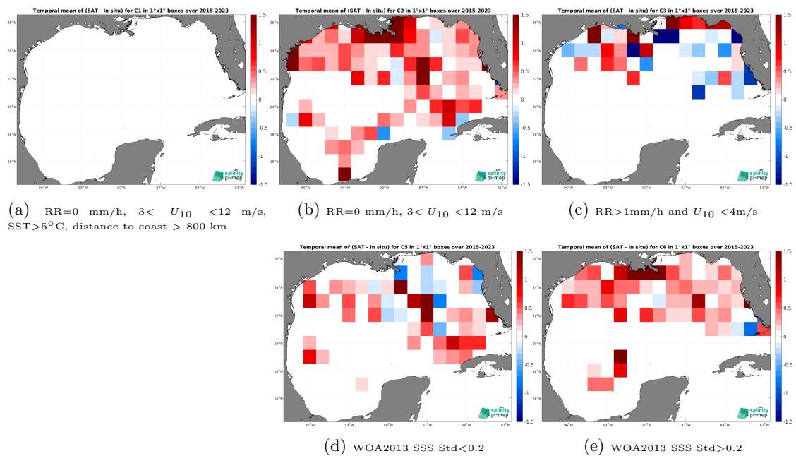
Figure 14: Temporal mean gridded over spatial boxes of size 1^\circ \times 1^\circ of \Delta SSS (SMAP SSS L2 v5.3 - 40 km (RSS) - TSG (SAMOS)) for 5 different subdatasets corresponding to:RR=0 mm/h, 3 < U_{10} < 12 m/s, SST>5°C, distance to coast > 800 km (a), RR=0 mm/h, 3 < U_{10} < 12 m/s (b), RR>1mm/h and U_{10} < 4 m/s (c), WOA2013 SSS Std<0.2 (d), WOA2013 SSS Std>0.2 (e).
