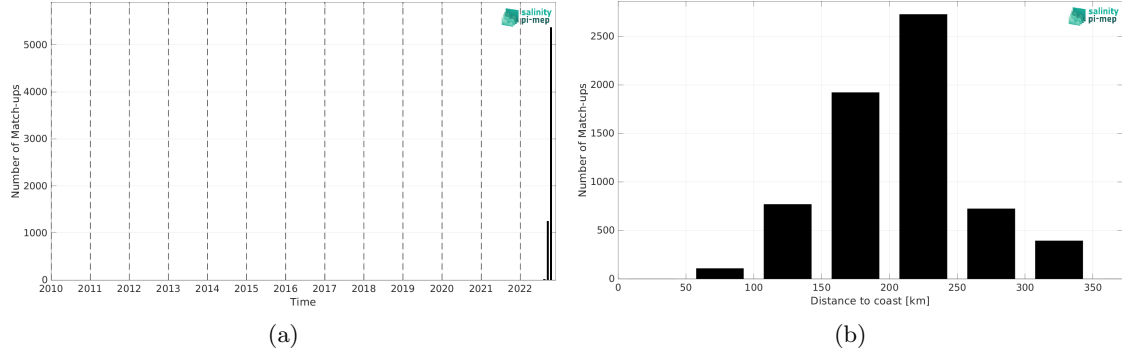
Figure 2: Number of match-ups between Saildrone and SMAP SSS L2 v5.3 - 40 km (RSS) SSS as a function of time (a) and as function of the distance to coast (b) over the Gulf of Mexico Pi-MEP region and for the full satellite product period.
