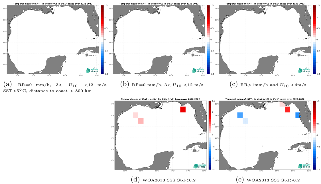
Figure 14: Temporal mean gridded over spatial boxes of size 1^\circ \times 1^\circ of \Delta SSS (SMAP SSS L2 v5.3 - 40 km (RSS) - Saildrone) for 5 different subdatasets corresponding to:RR=0 mm/h, 3 < U_{10} < 12 m/s, SST >5^\circ\text{C} , distance to coast > 800 km (a), RR=0 mm/h, 3 < U_{10} < 12 m/s (b), RR >1 mm/h and U_{10} < 4 m/s (c), WOA2013 SSS Std <0.2 (d), WOA2013 SSS Std >0.2 (e).
