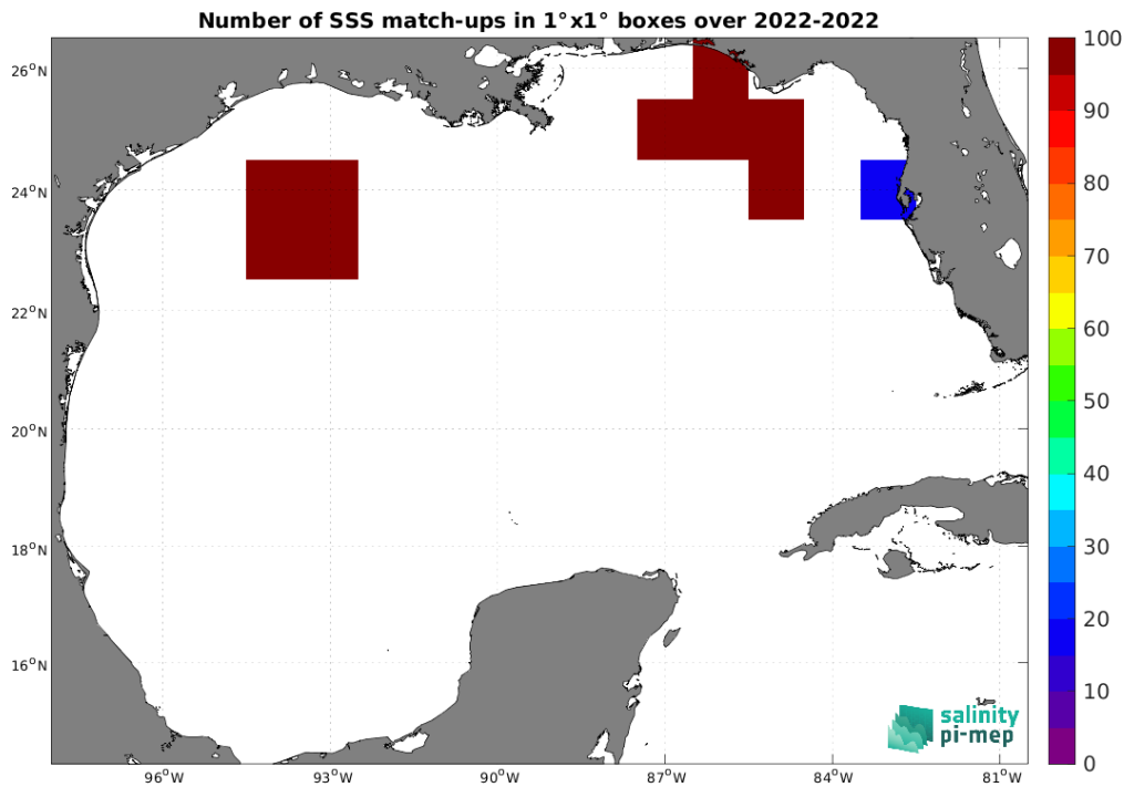
Figure 5: Number of SSS match-ups between Saildrone SSS and the SMAP SSS L2 v5.3 - 40 km (RSS) SSS product for the Gulf of Mexico Pi-MEP region over 1^\circ \times 1^\circ boxes and for the full satellite product period.
