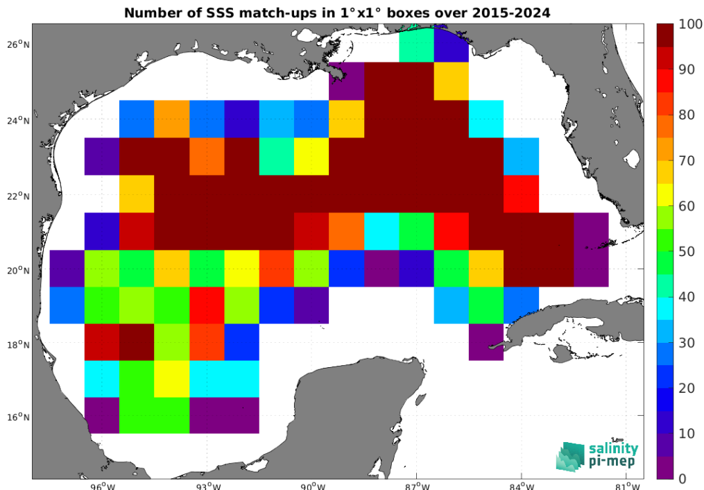
Figure 5: Number of SSS match-ups between Argo SSS and the SMAP SSS L2 v5.3 - 40 km (RSS) SSS product for the Gulf of Mexico Pi-MEP region over 1^\circ \times 1^\circ boxes and for the full satellite product period.
