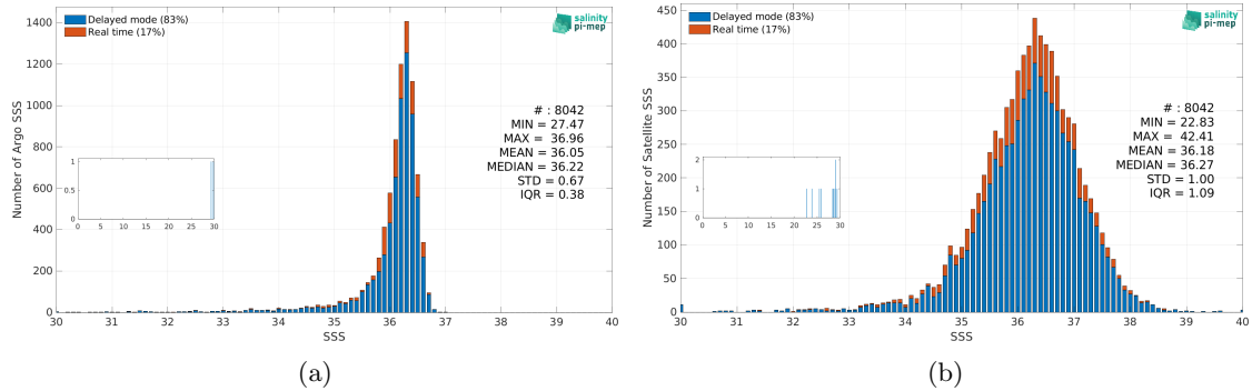
Figure 3: Histograms of SSS from Argo (a) and SMAP SSS L2 v5.3 - 40 km (RSS) (b) considering all match-up pairs per bins of 0.1 over the Gulf of Mexico Pi-MEP region and for the full satellite product period.
