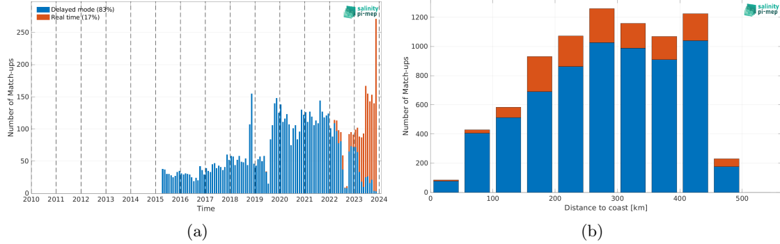
Figure 2: Number of match-ups between Argo and SMAP SSS L2 v5.3 - 40 km (RSS) SSS as a function of time (a) and as function of the distance to coast (b) over the Gulf of Mexico Pi-MEP region and for the full satellite product period.
