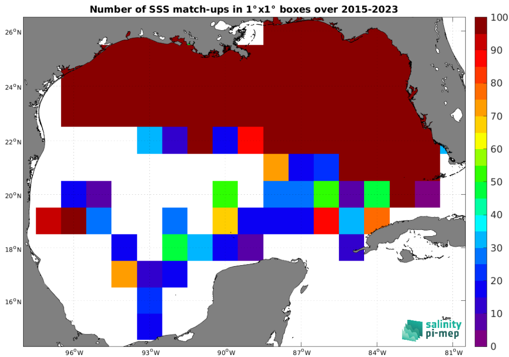
Figure 4: Number of SSS match-ups between TSG (SAMOS) SSS and the SMAP SSS L2 v5 - 40 km (RSS) SSS product for the Gulf of Mexico Pi-MEP region over 1^\circ \times 1^\circ boxes and for the full satellite product period.
