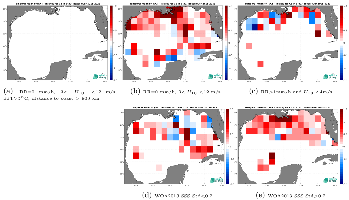
Figure 12: Temporal mean gridded over spatial boxes of size 1^\circ \times 1^\circ of \Delta SSS (SMAP SSS L2 v5 - 40 km (RSS) - TSG (SAMOS)) for 5 different subdatasets corresponding to:RR=0 mm/h, 3 < U_{10} < 12 m/s, SST >5^\circ\text{C} , distance to coast > 800 km (a), RR=0 mm/h, 3 < U_{10} < 12 m/s (b), RR >1 mm/h and U_{10} < 4 m/s (c), WOA2013 SSS Std <0.2 (d), WOA2013 SSS Std >0.2 (e).
