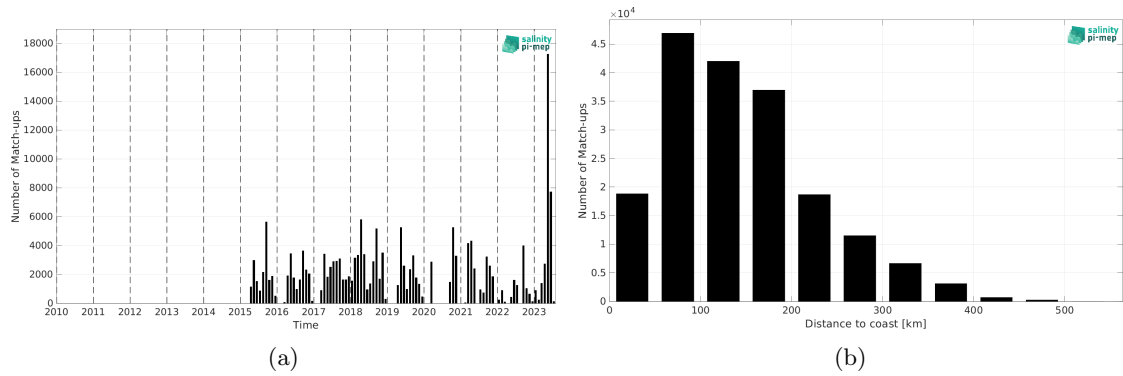
Figure 1: Number of match-ups between TSG (SAMOS) and SMAP SSS L2 v5 - 40 km (RSS) SSS as a function of time (a) and as function of the distance to coast (b) over the Gulf of Mexico Pi-MEP region and for the full satellite product period.
