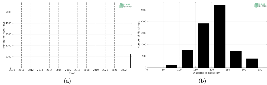
Figure 1: Number of match-ups between Saildrone and SMAP SSS L2 v5 - 40 km (RSS) SSS as a function of time (a) and as function of the distance to coast (b) over the Gulf of Mexico Pi-MEP region and for the full satellite product period.
