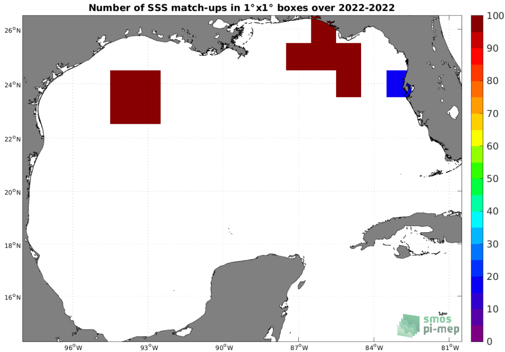
Figure 4: Number of SSS match-ups between Saildrone SSS and the SMAP SSS L2 v5 - 40 km (RSS) SSS product for the Gulf of Mexico Pi-MEP region over 1^\circ \times 1^\circ boxes and for the full satellite product period.
