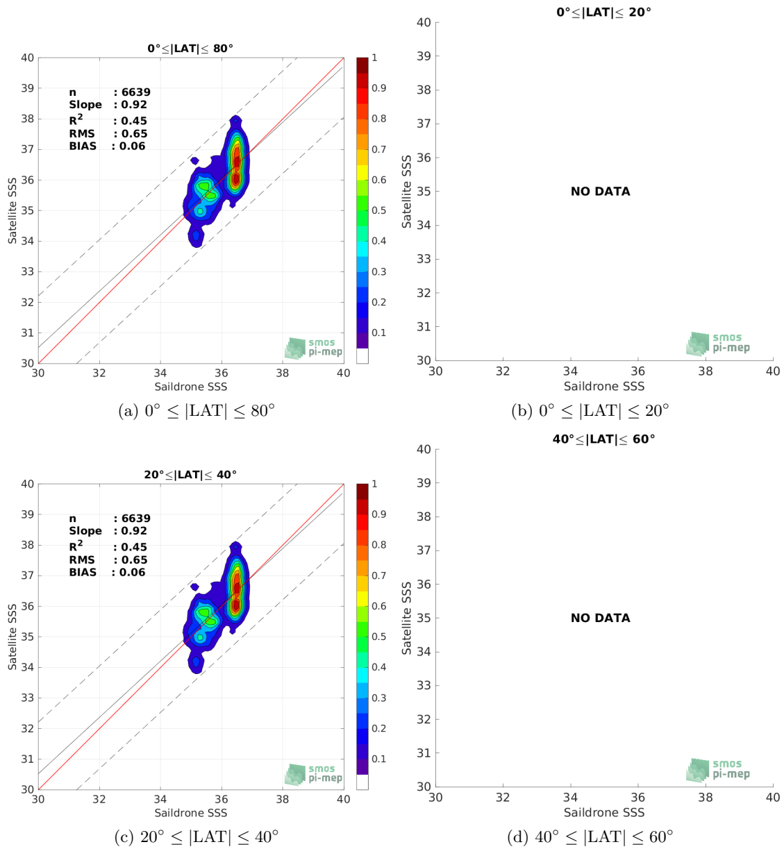
Figure 9: Contour maps of the concentration of SMAP SSS L2 v5 - 40 km (RSS) SSS (y-axis) versus Saïdrone SSS (x-axis) at match-up pairs for different latitude bands. For each plot, the red line shows x=y . The black thin and dashed lines indicate a linear fit through the data cloud and the \pm 95\% confidence levels, respectively. The number match-up pairs n , the slope and R^2 coefficient of the linear fit, the root mean square (RMS) and the mean bias between satellite and in situ data are indicated for each latitude band in each plots.
