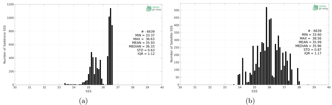
Figure 2: Histograms of SSS from Saildrone (a) and SMAP SSS L2 v5 - 40 km (RSS) (b) considering all match-up pairs per bins of 0.1 over the Gulf of Mexico Pi-MEP region and for the full satellite product period.
