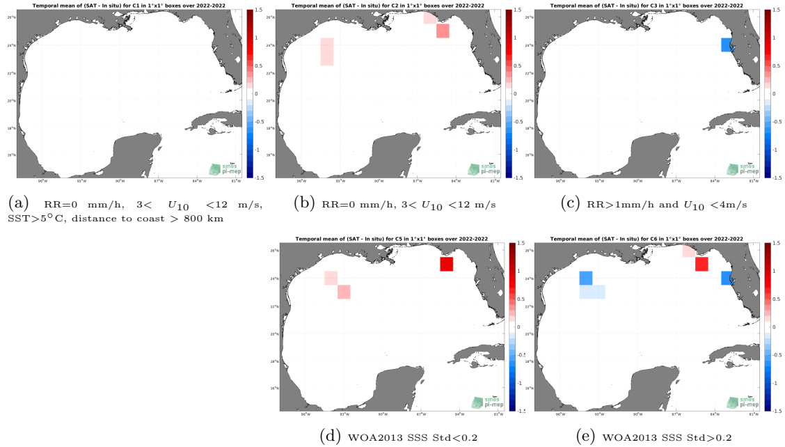
Figure 12: Temporal mean gridded over spatial boxes of size 1^{\circ}\times 1^{\circ} of \Delta\text{SSS} (SMAP SSS L2 v5 - 40 km (RSS) - Saildrone) for 5 different subdatasets corresponding to:RR=0 mm/h, 3 < U_{10} < 12 m/s, SST >5^{\circ}\text{C} , distance to coast > 800 km (a), RR=0 mm/h, 3 < U_{10} < 12 m/s (b), RR >1 mm/h and U_{10} < 4 m/s (c), WOA2013 SSS Std <0.2 (d), WOA2013 SSS Std >0.2 (e).
