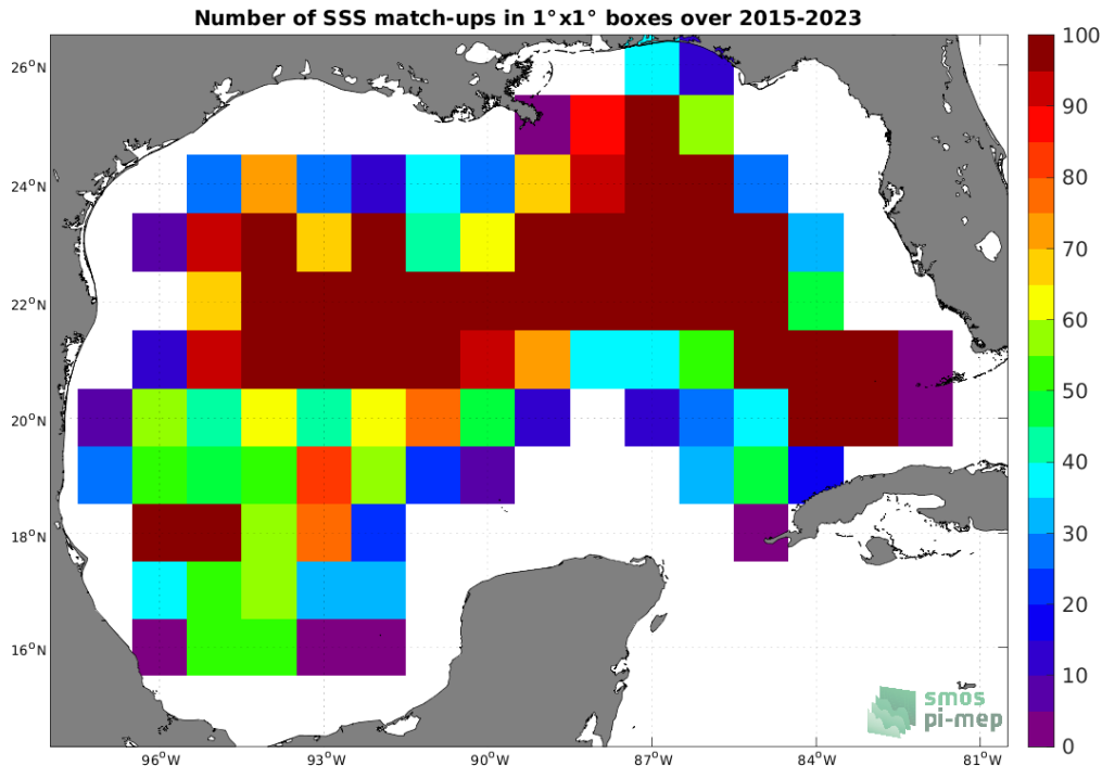
Figure 4: Number of SSS match-ups between Argo SSS and the SMAP SSS L2 v5 - 40 km (RSS) SSS product for the Gulf of Mexico Pi-MEP region over 1^{\circ} \times 1^{\circ} boxes and for the full satellite product period.
