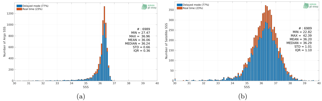
Figure 2: Histograms of SSS from Argo (a) and SMAP SSS L2 v5 - 40 km (RSS) (b) considering all match-up pairs per bins of 0.1 over the Gulf of Mexico Pi-MEP region and for the full satellite product period.
