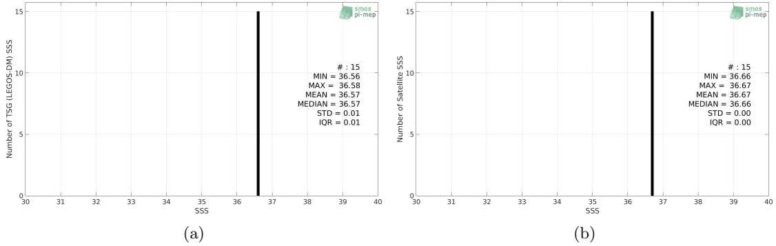
Figure 2: Histograms of SSS from TSG (LEGOS-DM) (a) and SMAP SSS L2 v4 (RSS) (b) considering all match-up pairs per bins of 0.1 over the Gulf of Mexico Pi-MEP region and for the full satellite product period.
