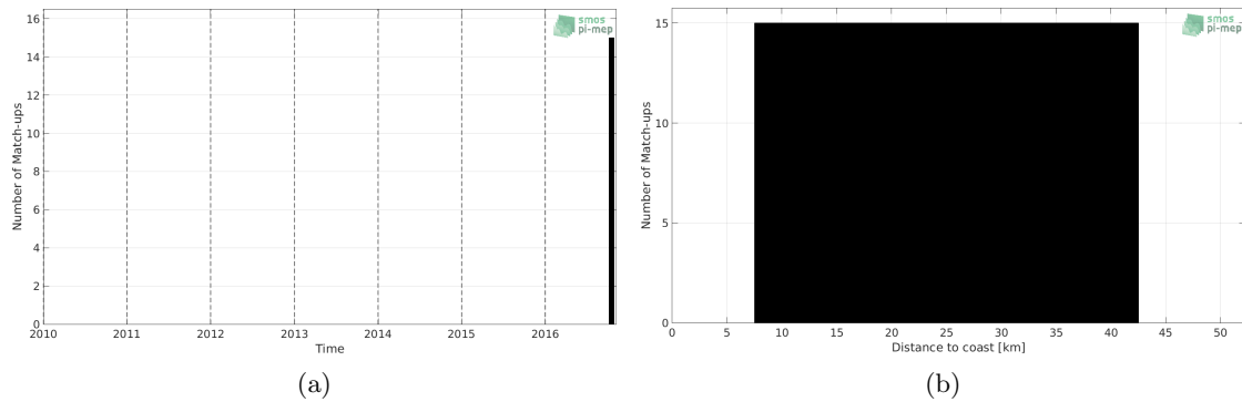
Figure 1: Number of match-ups between TSG (LEGOS-DM) and SMAP SSS L2 v4 (RSS) SSS as a function of time (a) and as function of the distance to coast (b) over the Gulf of Mexico Pi-MEP region and for the full satellite product period.
