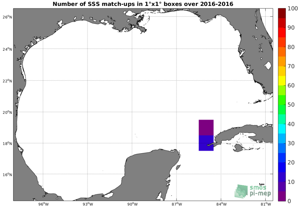
Figure 4: Number of SSS match-ups between TSG (LEGOS-DM) SSS and the SMAP SSS L2 v4 (RSS) SSS product for the Gulf of Mexico Pi-MEP region over 1°x1° boxes and for the full satellite product period.
