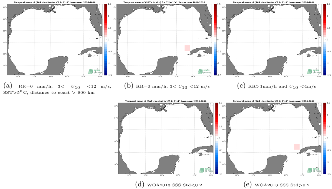
Figure 12: Temporal mean gridded over spatial boxes of size 1^{\circ}\times 1^{\circ} of \Delta\text{SSS} (SMAP SSS L2 v4 (RSS) - TSG (LEGOS-DM)) for 5 different subdatasets corresponding to: RR=0 mm/h, 3 < U_{10} < 12 m/s, SST > 5^{\circ}\text{C} , distance to coast > 800 km (a), RR=0 mm/h, 3 < U_{10} < 12 m/s (b), RR > 1 mm/h and U_{10} < 4 m/s (c), WOA2013 SSS Std < 0.2 (d), WOA2013 SSS Std > 0.2 (e).
