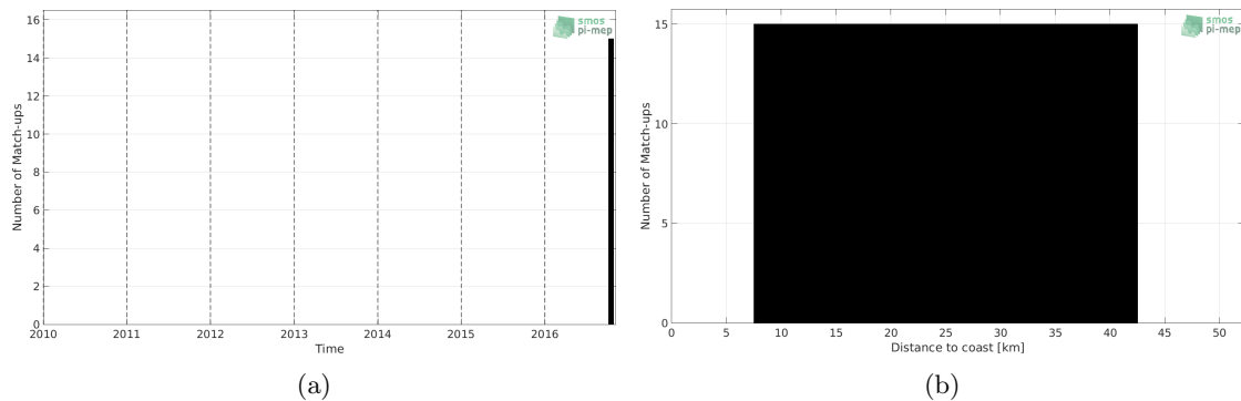
Figure 1: Number of match-ups between TSG-LEGOS-DM and SMAP-L2-RSS-V4 SSS as a function of time (a) and as function of the distance to coast (b) over the Gulf of Mexico Pi-MEP region and for the full satellite product period.
