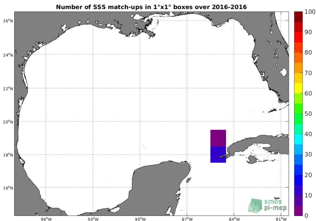
Figure 4: Number of SSS match-ups between TSG-LEGOS-DM SSS and the SMAP-L2-RSS-V4 SSS product for the Gulf of Mexico Pi-MEP region over 1°x1° boxes and for the full satellite product period.
