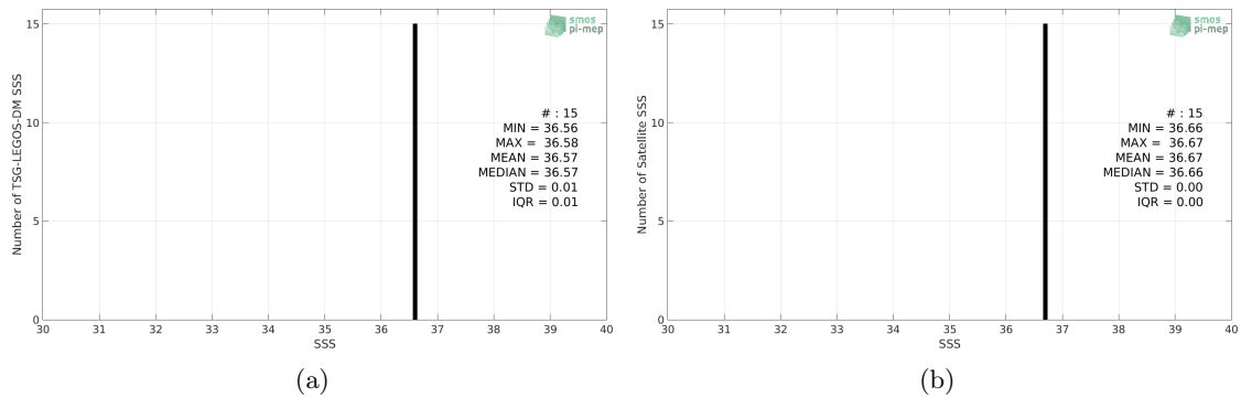
Figure 2: Histograms of SSS from TSG-LEGOS-DM (a) and SMAP-L2-RSS-V4 (b) considering all match-up pairs per bins of 0.1 over the Gulf of Mexico Pi-MEP region and for the full satellite product period.
