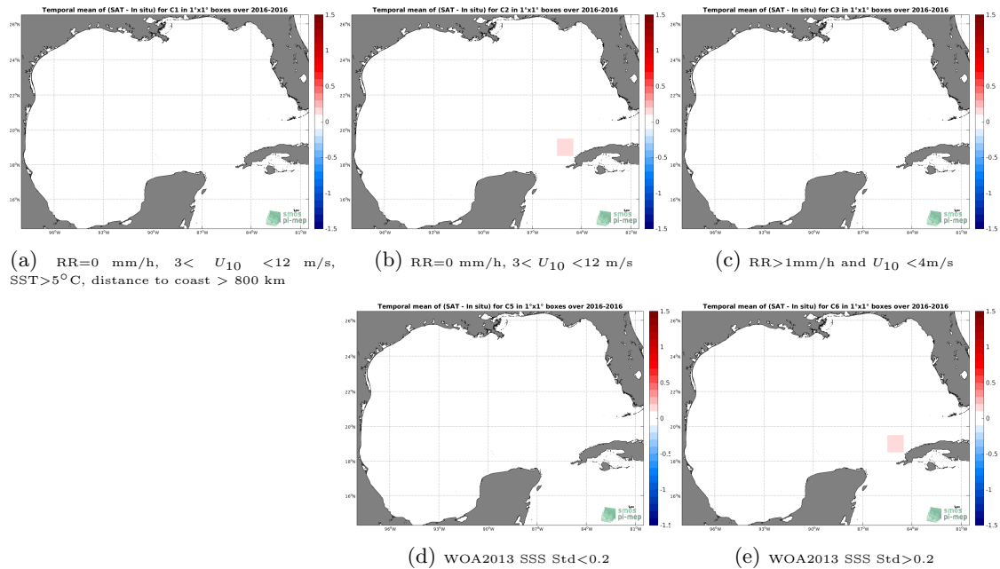
Figure 12: Temporal mean gridded over spatial boxes of size 1^{\circ}\times 1^{\circ} of \Delta\text{SSS} (SMAP-L2-RSS-V4 - TSG-LEGOS-DM) for 5 different subdatasets corresponding to:RR=0 mm/h, 3 < U_{10} < 12 m/s, SST >5^{\circ}\text{C} , distance to coast > 800 km (a), RR=0 mm/h, 3 < U_{10} < 12 m/s (b), RR >1 mm/h and U_{10} < 4 m/s (c), WOA2013 SSS Std <0.2 (d), WOA2013 SSS Std >0.2 (e).
