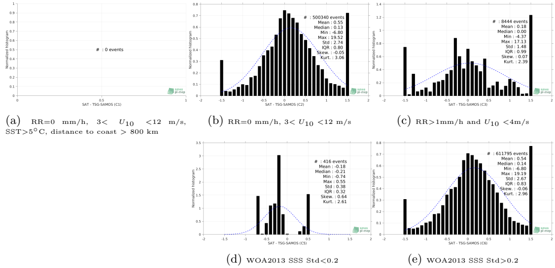
Figure 13: Normalized histogram of \Delta SSS (SMAP-L2-RSS-V3-70KM - TSG-SAMOS) for 5 different subdatasets corresponding to: RR=0 mm/h, 3 < U_{10} < 12 m/s, SST > 5°C, distance to coast > 800 km (a), RR=0 mm/h, 3 < U_{10} < 12 m/s (b), RR > 1mm/h and U_{10} < 4 m/s (c), WOA2013 SSS Std < 0.2 (d), WOA2013 SSS Std > 0.2 (e).
