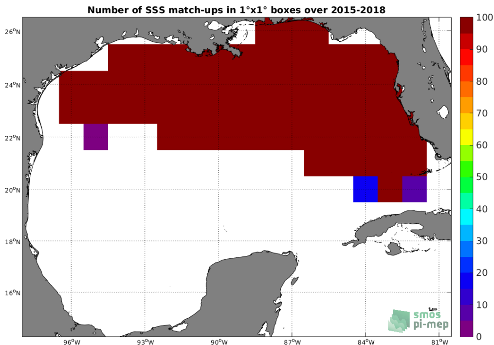
Figure 4: Number of SSS match-ups between TSG-SAMOS SSS and the SMAP-L2-RSS-V3-70KM SSS product for the Gulf of Mexico Pi-MEP region over 1°x1° boxes and for the full satellite product period.
