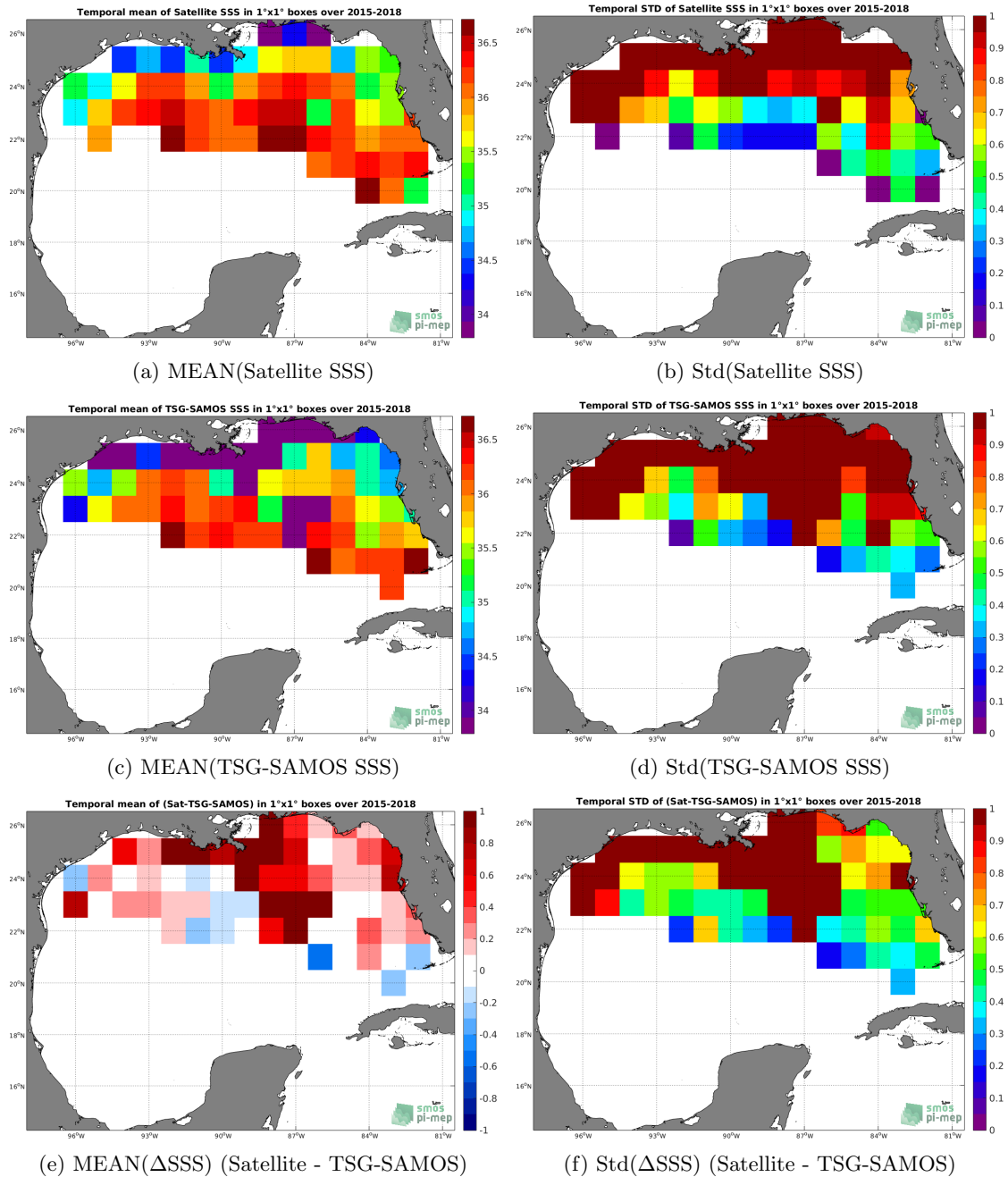
Figure 6: Temporal mean (left) and Std (right) of SSS from SMAP-L2-RSS-V3-70KM (top), TSG-SAMOS (middle), and of \Delta SSS (Satellite - TSG-SAMOS). Only match-up pairs are used to generate these maps.
