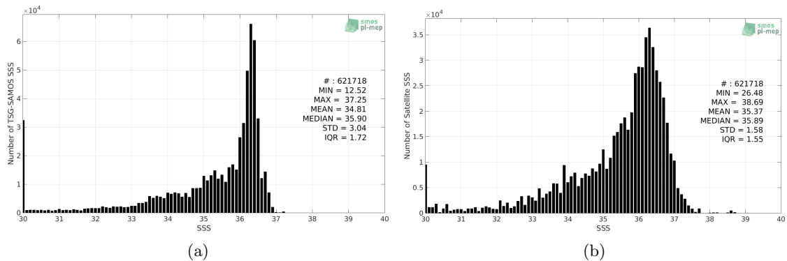
Figure 2: Histograms of SSS from TSG-SAMOS (a) and SMAP-L2-RSS-V3-70KM (b) considering all match-up pairs per bins of 0.1 over the Gulf of Mexico Pi-MEP region and for the full satellite product period.
