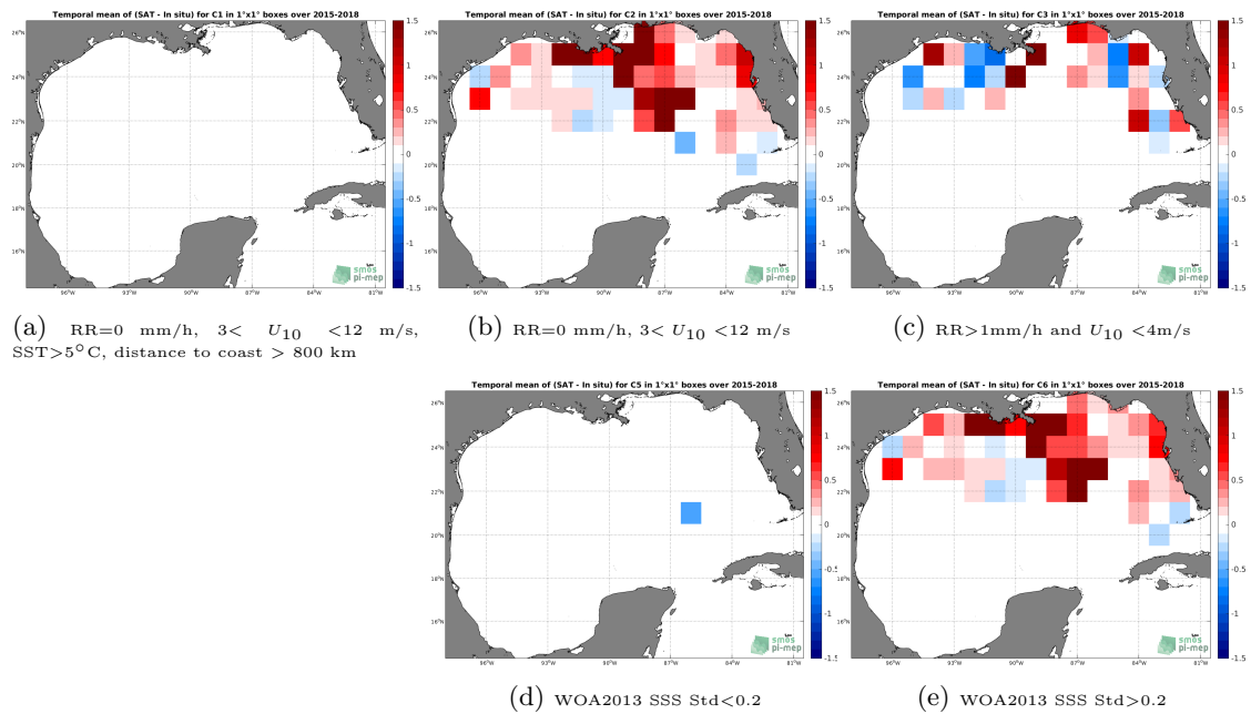
Figure 12: Temporal mean gridded over spatial boxes of size 1^\circ \times 1^\circ of \Delta SSS (SMAP-L2-RSS-V3-70KM - TSG-SAMOS) for 5 different subdatasets corresponding to:RR=0 mm/h, 3 < U_{10} < 12 m/s, SST >5^\circ\text{C} , distance to coast > 800 km (a), RR=0 mm/h, 3 < U_{10} < 12 m/s (b), RR >1 mm/h and U_{10} < 4 m/s (c), WOA2013 SSS Std <0.2 (d), WOA2013 SSS Std >0.2 (e).
