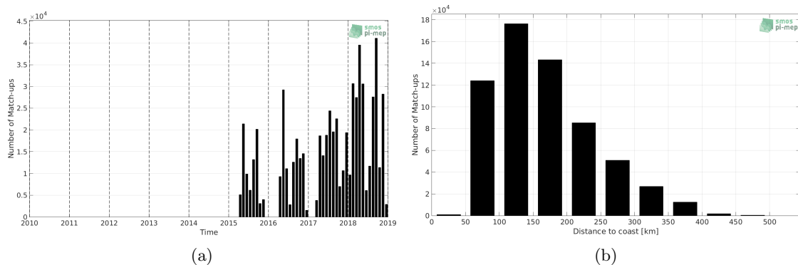
Figure 1: Number of match-ups between TSG-SAMOS and SMAP-L2-RSS-V3-70KM SSS as a function of time (a) and as function of the distance to coast (b) over the Gulf of Mexico Pi-MEP region and for the full satellite product period.
