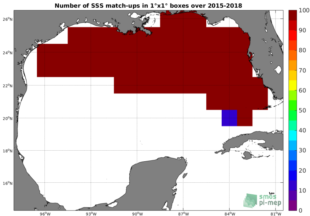
Figure 4: Number of SSS match-ups between TSG-SAMOS SSS and the SMAP-L2-RSS-V3-70KM SSS product for the Gulf of Mexico Pi-MEP region over 1^\circ \times 1^\circ boxes and for the full satellite product period.
