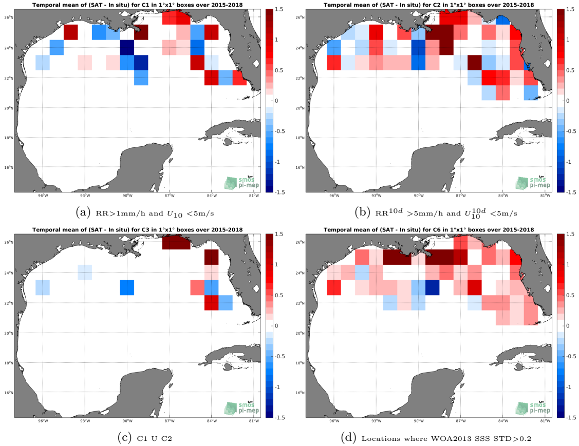
Figure 12: Temporal mean gridded over spatial boxes of size 1^\circ \times 1^\circ of \Delta SSS (SMAP-L2-RSS-V3-70KM - TSG-SAMOS) for 4 different subdatasets corresponding to: RR > 1 mm/h and U_{10} < 5 m/s (a), RR 10d > 5 mm/h and U_{10}^{10d} < 5 m/s (b), C1 U C2 (c), Locations where WOA2013 SSS STD > 0.2 (d).
