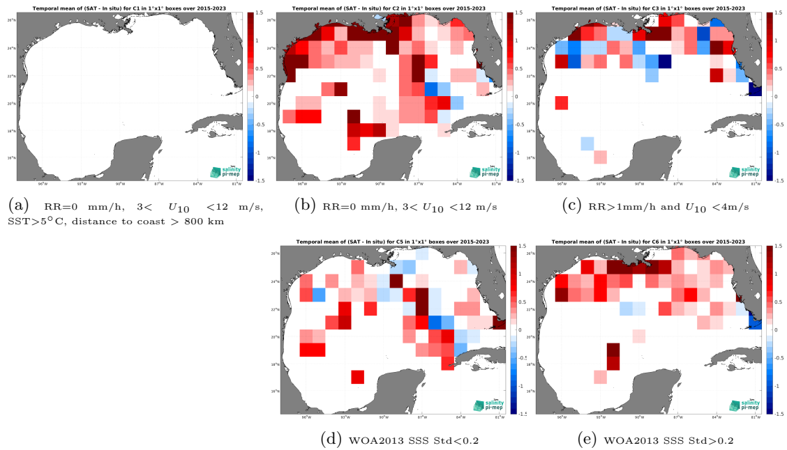
Figure 12: Temporal mean gridded over spatial boxes of size 1^\circ \times 1^\circ of \Delta\text{SSS} (SMAP SSS L2 v5.0 (JPL) - TSG (SAMOS)) for 5 different subdatasets corresponding to:RR=0 mm/h, 3 < U_{10} < 12 m/s, SST >5^\circ\text{C} , distance to coast > 800 km (a), RR=0 mm/h, 3 < U_{10} < 12 m/s (b), RR >1 mm/h and U_{10} < 4 m/s (c), WOA2013 SSS Std <0.2 (d), WOA2013 SSS Std >0.2 (e).
