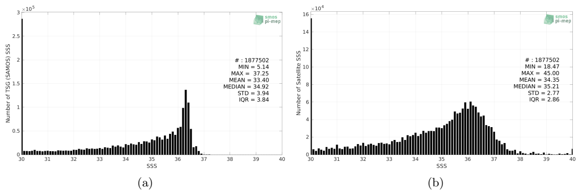
Figure 2: Histograms of SSS from TSG (SAMOS) (a) and SMAP SSS L2 v5.0 (JPL) (b) considering all match-up pairs per bins of 0.1 over the Gulf of Mexico Pi-MEP region and for the full satellite product period.
