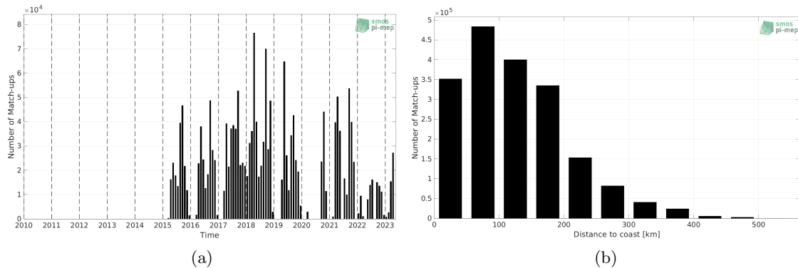
Figure 1: Number of match-ups between TSG (SAMOS) and SMAP SSS L2 v5.0 (JPL) SSS as a function of time (a) and as function of the distance to coast (b) over the Gulf of Mexico Pi-MEP region and for the full satellite product period.
