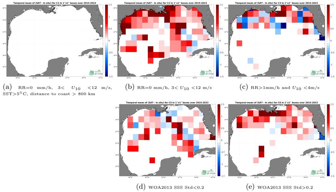
Figure 12: Temporal mean gridded over spatial boxes of size 1^\circ \times 1^\circ of \Delta SSS (SMAP SSS L2 v5.0 (JPL) - TSG (SAMOS)) for 5 different subdatasets corresponding to:RR=0 mm/h, 3 < U_{10} < 12 m/s, SST >5^\circ\text{C} , distance to coast > 800 km (a), RR=0 mm/h, 3 < U_{10} < 12 m/s (b), RR >1 mm/h and U_{10} < 4 m/s (c), WOA2013 SSS Std <0.2 (d), WOA2013 SSS Std >0.2 (e).
