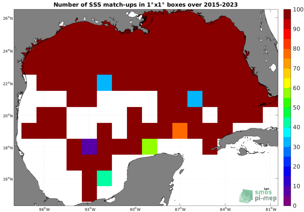
Figure 4: Number of SSS match-ups between TSG (SAMOS) SSS and the SMAP SSS L2 v5.0 (JPL) SSS product for the Gulf of Mexico Pi-MEP region over 1^\circ \times 1^\circ boxes and for the full satellite product period.
