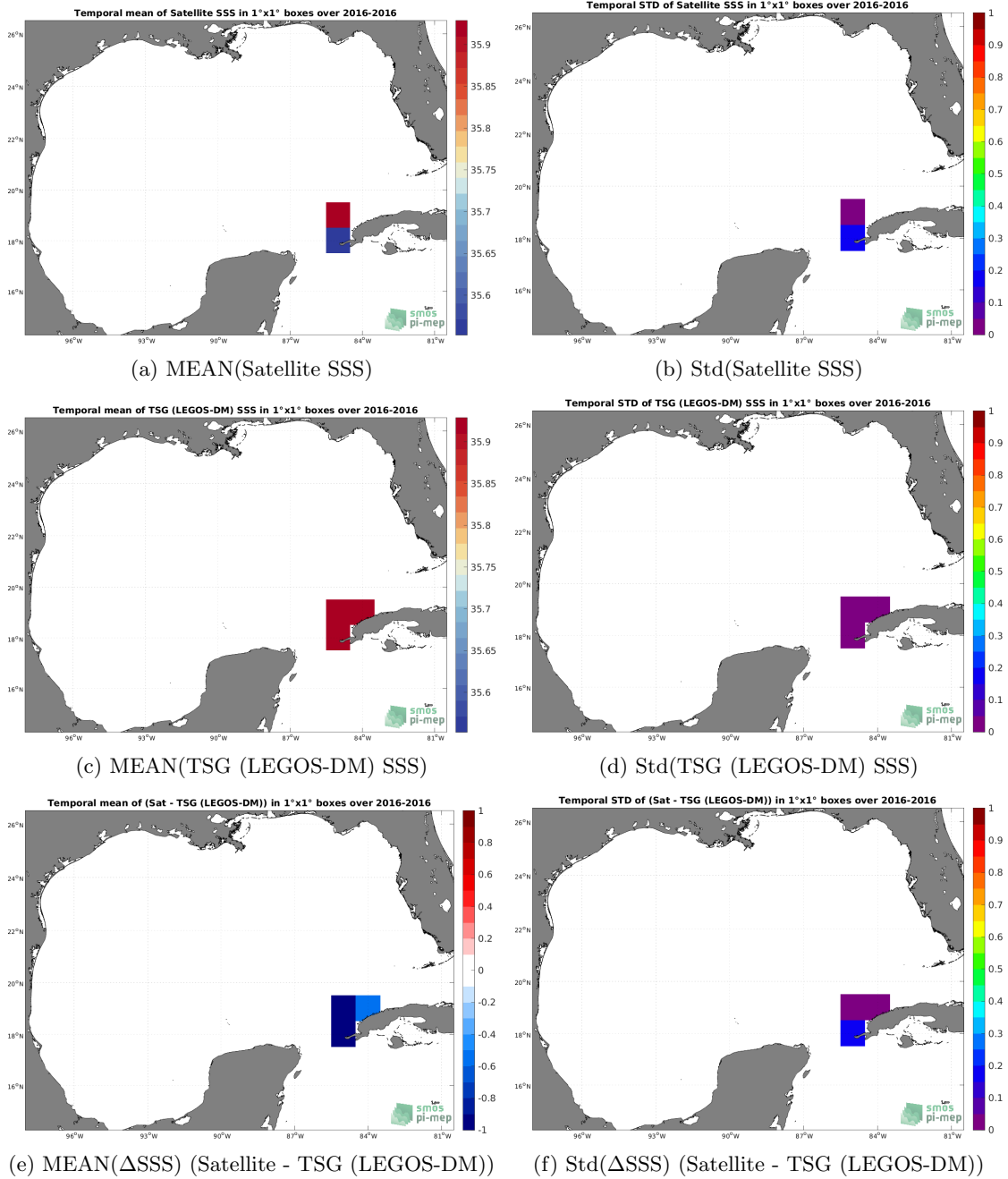
Figure 6: Temporal mean (left) and Std (right) of SSS from SMAP SSS L2 v5.0 (JPL) (top), TSG (LEGOS-DM) (middle), and of \Delta SSS (Satellite - TSG (LEGOS-DM)). Only match-up pairs are used to generate these maps.
