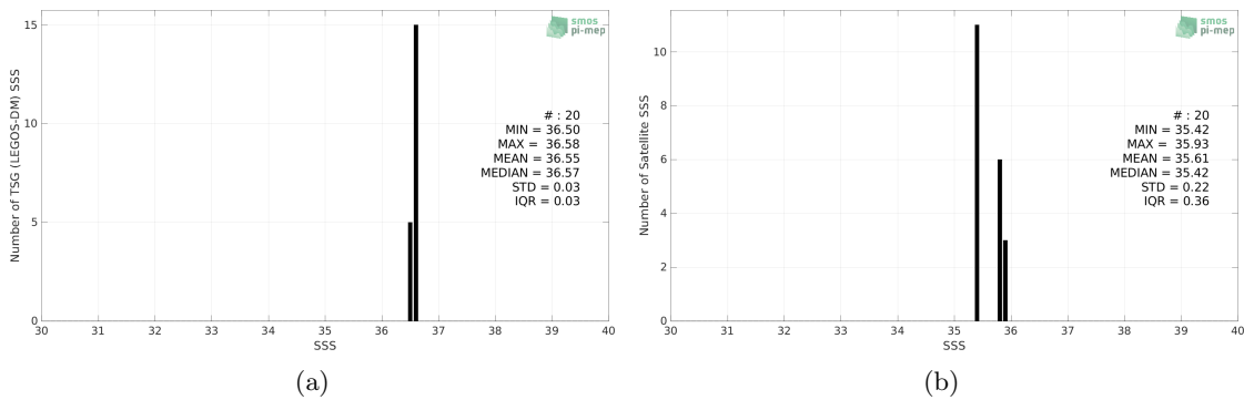
Figure 2: Histograms of SSS from TSG (LEGOS-DM) (a) and SMAP SSS L2 v5.0 (JPL) (b) considering all match-up pairs per bins of 0.1 over the Gulf of Mexico Pi-MEP region and for the full satellite product period.
