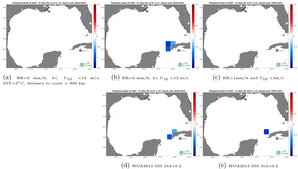
Figure 12: Temporal mean gridded over spatial boxes of size 1^{\circ}\times 1^{\circ} of \Delta\text{SSS} (SMAP SSS L2 v5.0 (JPL) - TSG (LEGOS-DM)) for 5 different subdatasets corresponding to:RR=0 mm/h, 3 < U_{10} < 12 m/s, SST >5^{\circ}\text{C} , distance to coast > 800 km (a), RR=0 mm/h, 3 < U_{10} < 12 m/s (b), RR >1 mm/h and U_{10} < 4 m/s (c), WOA2013 SSS Std <0.2 (d), WOA2013 SSS Std >0.2 (e).
