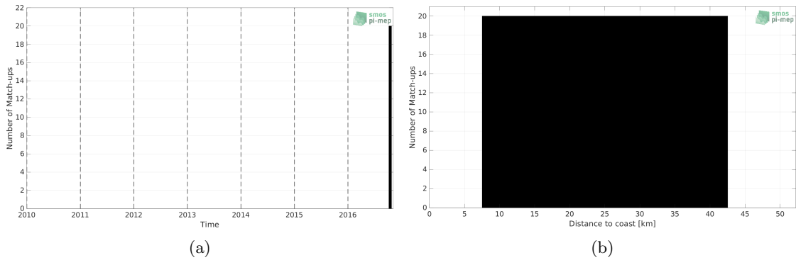
Figure 1: Number of match-ups between TSG (LEGOS-DM) and SMAP SSS L2 v5.0 (JPL) SSS as a function of time (a) and as function of the distance to coast (b) over the Gulf of Mexico Pi-MEP region and for the full satellite product period.
