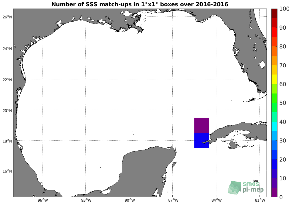
Figure 4: Number of SSS match-ups between TSG (LEGOS-DM) SSS and the SMAP SSS L2 v5.0 (JPL) SSS product for the Gulf of Mexico Pi-MEP region over 1°x1° boxes and for the full satellite product period.
