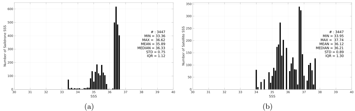
Figure 3: Histograms of SSS from Saildrone (a) and SMAP SSS L2 v5.0 (JPL) (b) considering all match-up pairs per bins of 0.1 over the Gulf of Mexico Pi-MEP region and for the full satellite product period.
