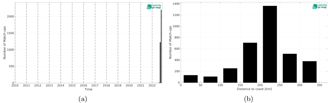
Figure 2: Number of match-ups between Saildrone and SMAP SSS L2 v5.0 (JPL) SSS as a function of time (a) and as function of the distance to coast (b) over the Gulf of Mexico Pi-MEP region and for the full satellite product period.
