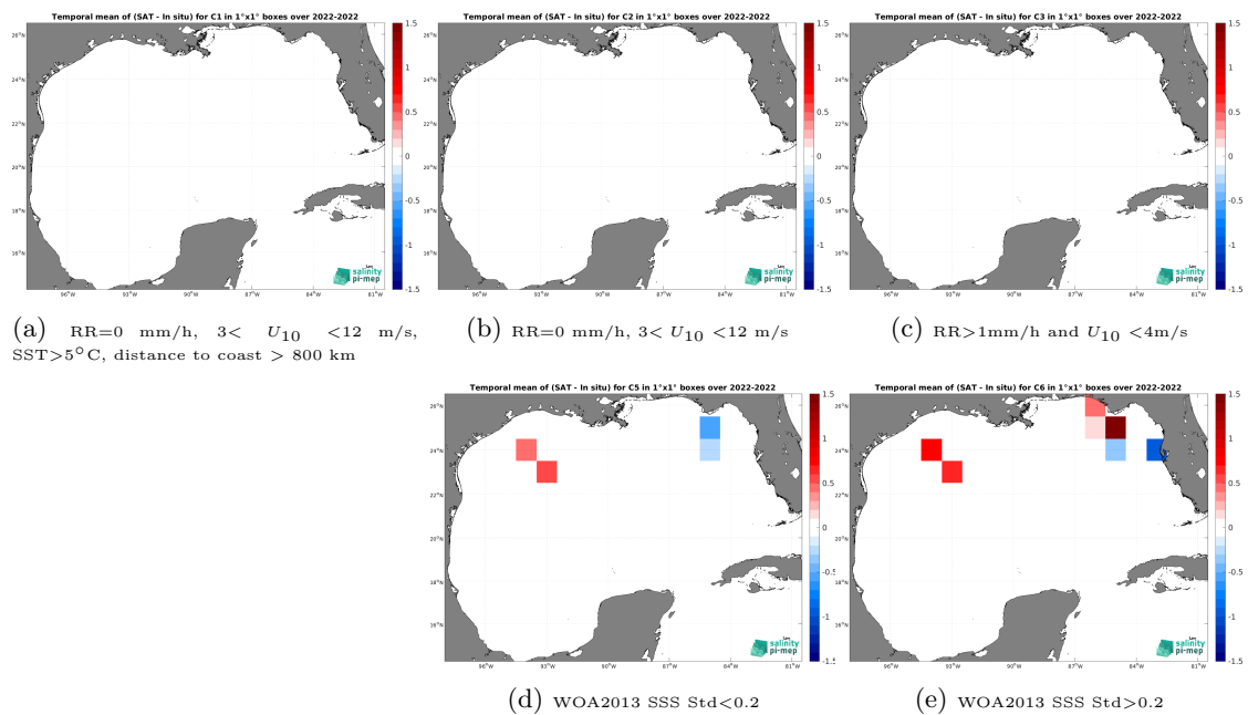
Figure 14: Temporal mean gridded over spatial boxes of size 1^\circ \times 1^\circ of \Delta SSS (SMAP SSS L2 v5.0 (JPL) - Saildrone) for 5 different subdatasets corresponding to:RR=0 mm/h, 3 < U_{10} < 12 m/s, SST >5^\circ C, distance to coast > 800 km (a), RR=0 mm/h, 3 < U_{10} < 12 m/s (b), RR >1 mm/h and U_{10} < 4 m/s (c), WOA2013 SSS Std <0.2 (d), WOA2013 SSS Std >0.2 (e).
