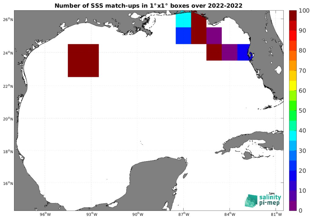
Figure 5: Number of SSS match-ups between Saildrone SSS and the SMAP SSS L2 v5.0 (JPL) SSS product for the Gulf of Mexico Pi-MEP region over 1^\circ \times 1^\circ boxes and for the full satellite product period.
