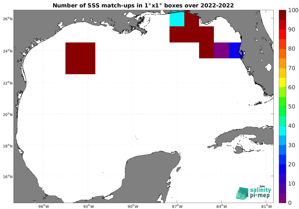
Figure 4: Number of SSS match-ups between Saildrone SSS and the SMAP SSS L2 v5.0 (JPL) SSS product for the Gulf of Mexico Pi-MEP region over 1^{\circ} \times 1^{\circ} boxes and for the full satellite product period.
