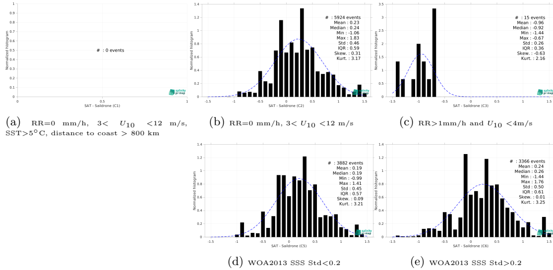
Figure 13: Normalized histogram of \Delta SSS (SMAP SSS L2 v5.0 (JPL) - Sairdrone) for 5 different subdatasets corresponding to: RR=0 mm/h, 3 < U_{10} < 12 m/s, SST > 5°C, distance to coast > 800 km (a), RR=0 mm/h, 3 < U_{10} < 12 m/s (b), RR > 1mm/h and U_{10} < 4 m/s (c), WOA2013 SSS Std < 0.2 (d), WOA2013 SSS Std > 0.2 (e).
