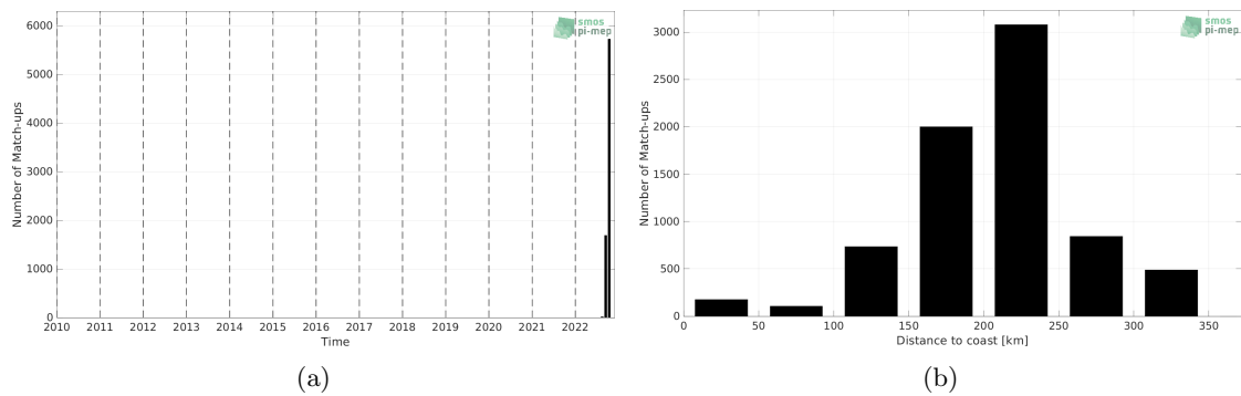
Figure 1: Number of match-ups between Saildrone and SMAP SSS L2 v5.0 (JPL) SSS as a function of time (a) and as function of the distance to coast (b) over the Gulf of Mexico Pi-MEP region and for the full satellite product period.
