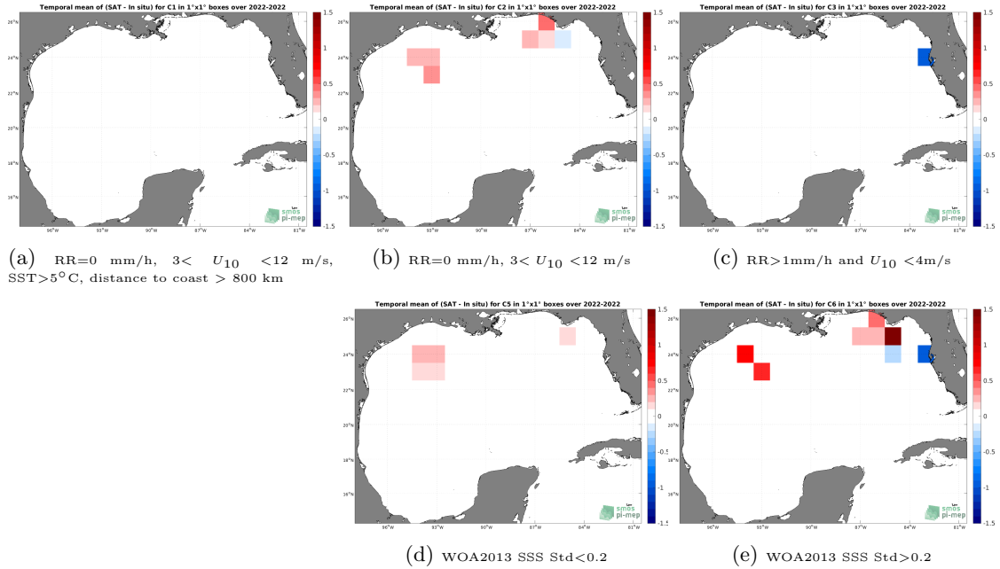
Figure 12: Temporal mean gridded over spatial boxes of size 1^{\circ}\times 1^{\circ} of \Delta\text{SSS} (SMAP SSS L2 v5.0 (JPL) - Saldrone) for 5 different subdatasets corresponding to:RR=0 mm/h, 3 < U_{10} < 12 m/s, SST >5^{\circ}\text{C} , distance to coast > 800 km (a), RR=0 mm/h, 3 < U_{10} < 12 m/s (b), RR >1 mm/h and U_{10} < 4 m/s (c), WOA2013 SSS Std <0.2 (d), WOA2013 SSS Std >0.2 (e).
