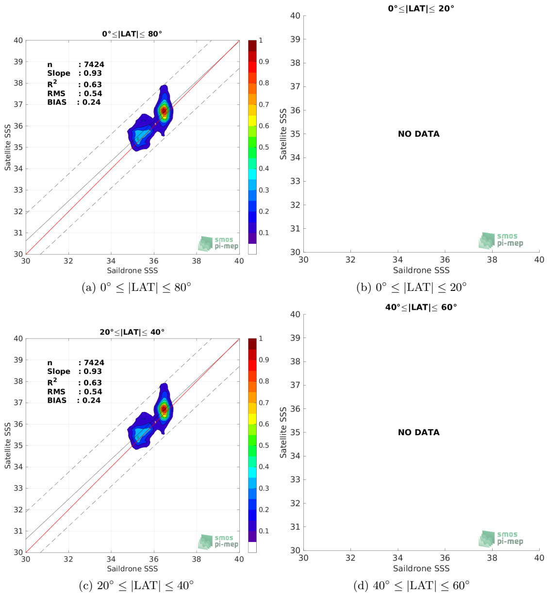
Figure 9: Contour maps of the concentration of SMAP SSS L2 v5.0 (JPL) SSS (y-axis) versus Saïldrone SSS (x-axis) at match-up pairs for different latitude bands. For each plot, the red line shows x=y . The black thin and dashed lines indicate a linear fit through the data cloud and the \pm 95\% confidence levels, respectively. The number match-up pairs n , the slope and R^2 coefficient of the linear fit, the root mean square (RMS) and the mean bias between satellite and in situ data are indicated for each latitude band in each plots.
