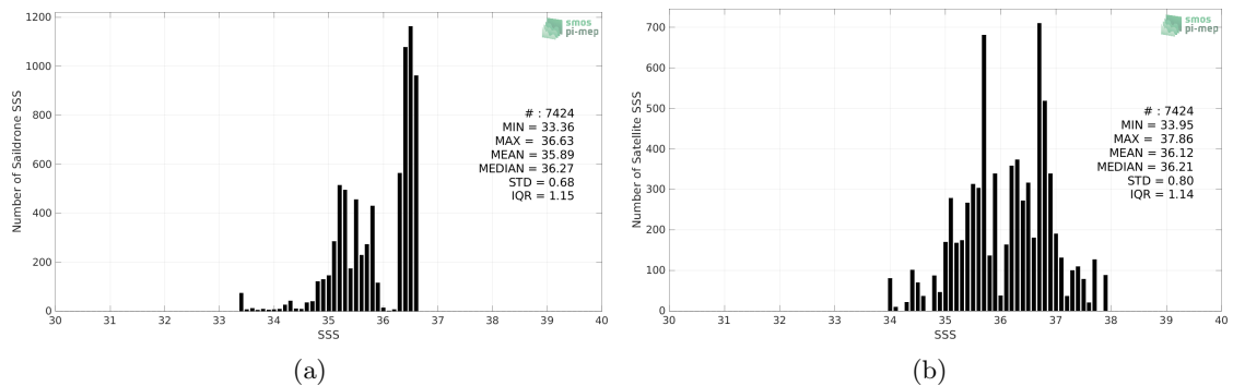
Figure 2: Histograms of SSS from Saildrone (a) and SMAP SSS L2 v5.0 (JPL) (b) considering all match-up pairs per bins of 0.1 over the Gulf of Mexico Pi-MEP region and for the full satellite product period.
